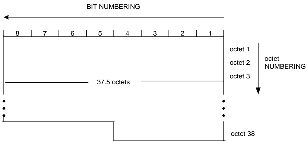
Figure 6.11: FACCH9 block format
