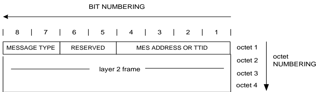
Figure 6.12: TACCH block format when the message type field indicates "01"
