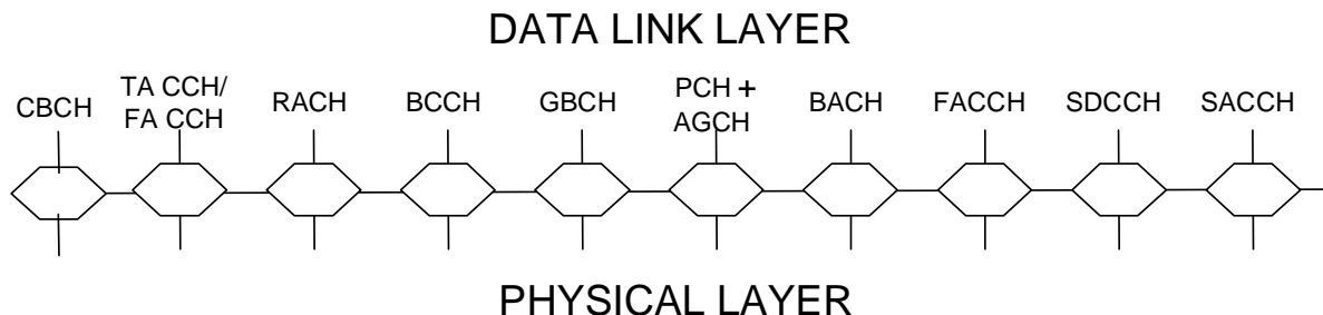
Figure 5.2: SAPs between the physical layer and the data link layer in the MES
