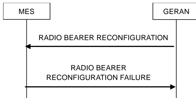
Figure 7.14.1.0.4: Radio Bearer Reconfiguration, failure case
