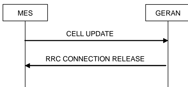
Figure 7.8.1.0.5: Cell Update procedure, failure case
