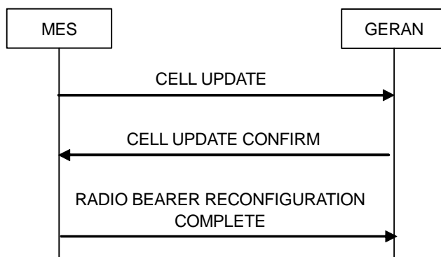
Figure 7.8.1.0.4: Cell Update procedure with radio bearer reconfiguration
