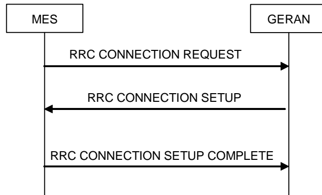
Figure 7.5.1.0.1: RRC Connection Establishment, network accepts RRC connection
