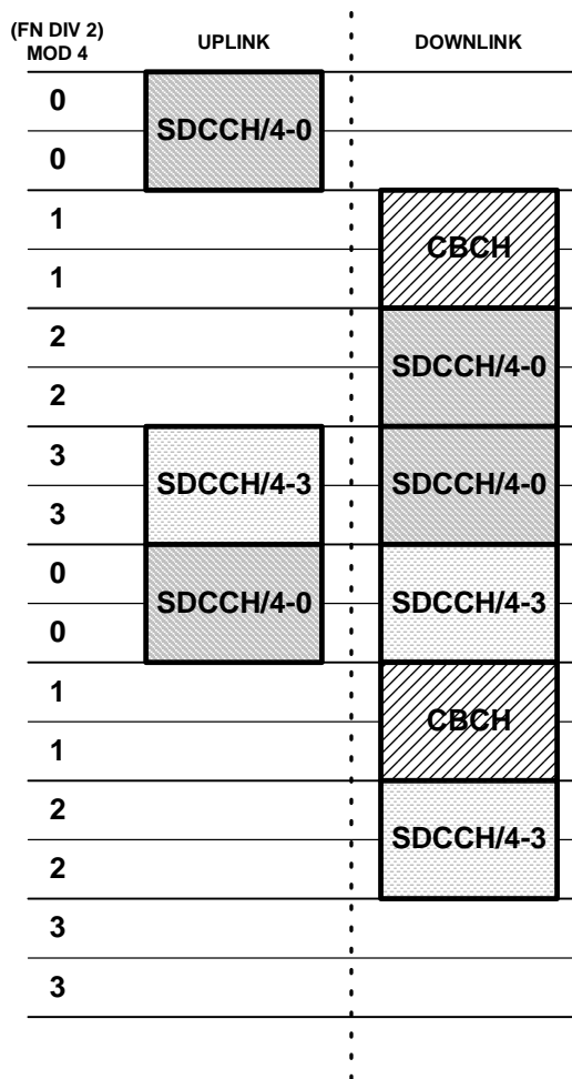
Figure 8.1: An SDCCH multiplexed in a PC6d
