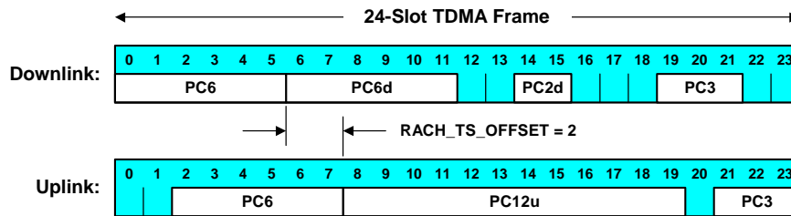
Figure 9.1: A RACH_TS_OFFSET example
