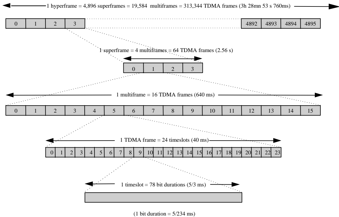
Figure 6.1: Timeframe structures and timeslots
