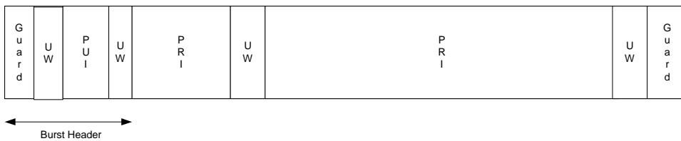
(c) PNB3(5,3) Uplink
