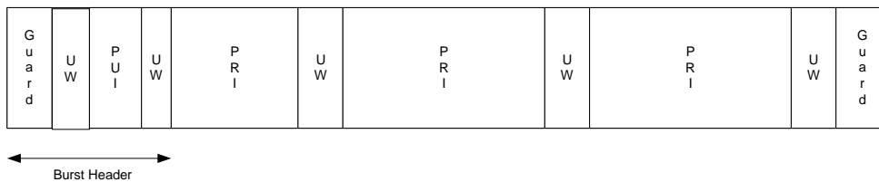
(f) PNB3(5,12) Uplink
