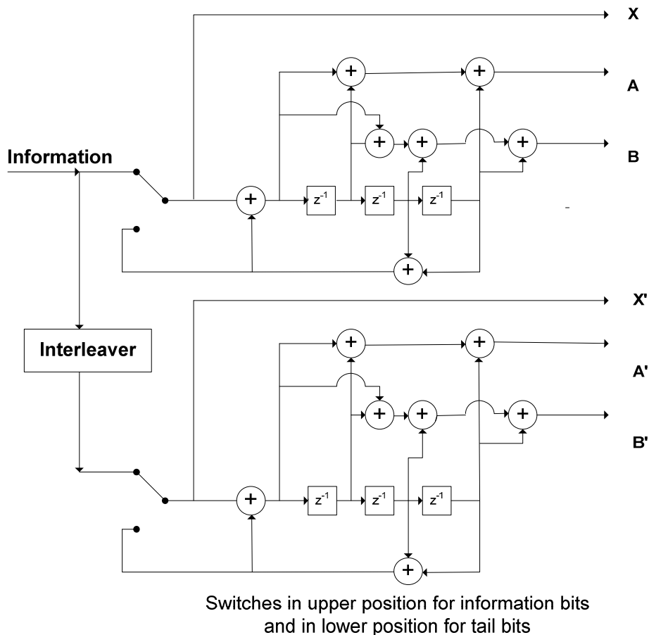
Figure 4.1 Structure of Turbo encoder
