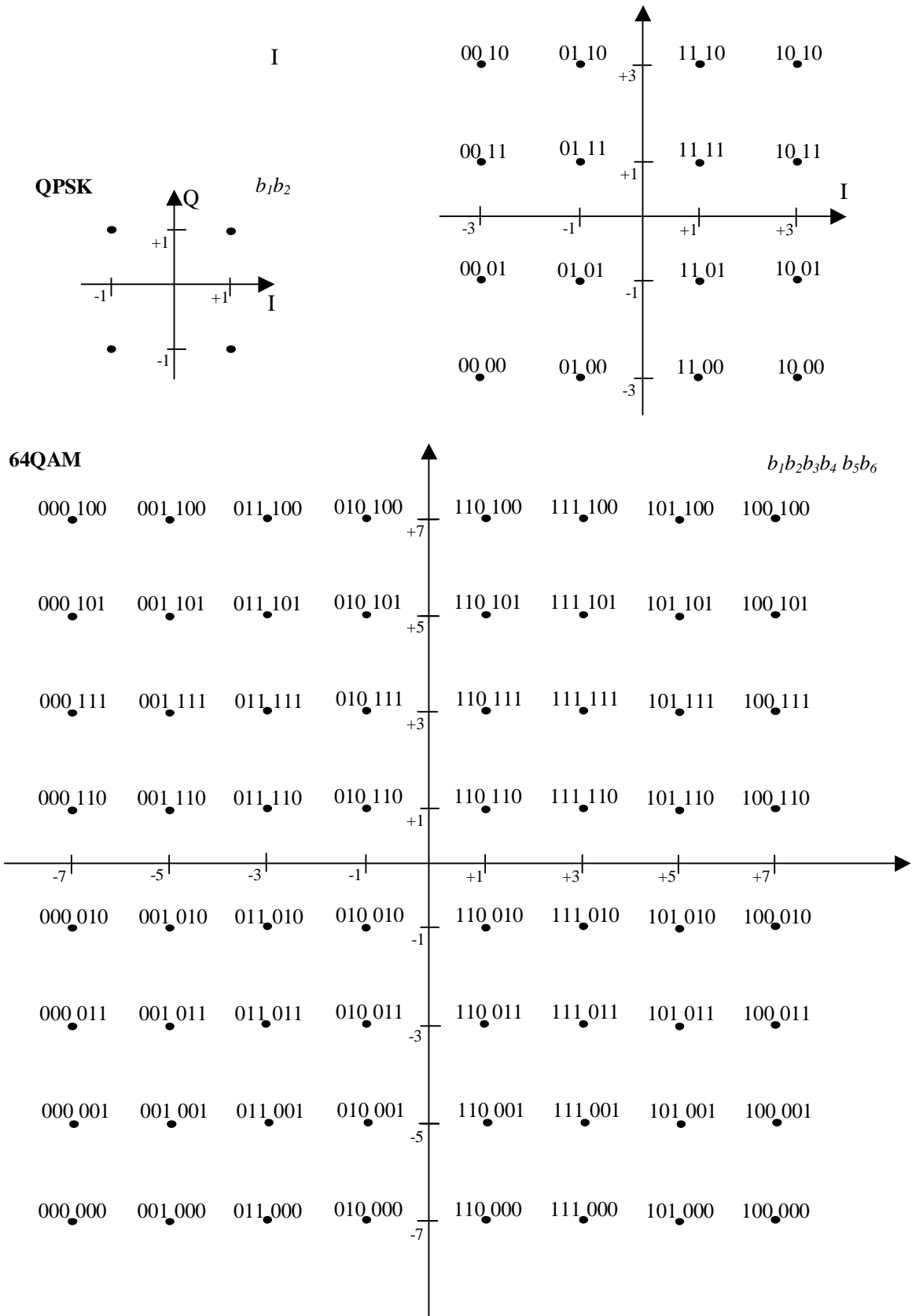
Figure 7: BPSK, QPSK, 16QAM and 64QAM constellation bit encoding
