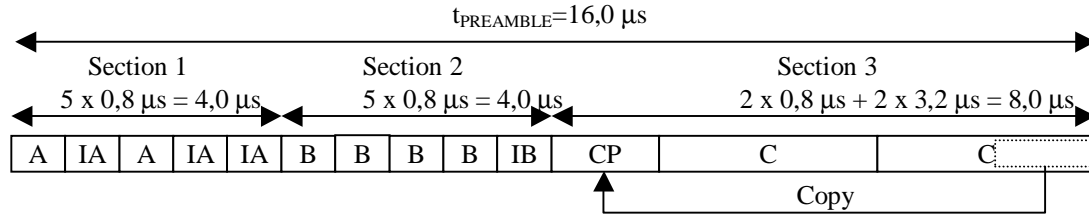
Figure 12: Broadcast burst preamble
