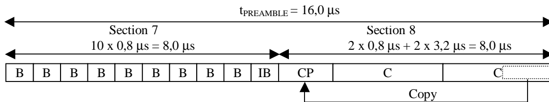
Figure 15: Long preamble for uplink bursts
