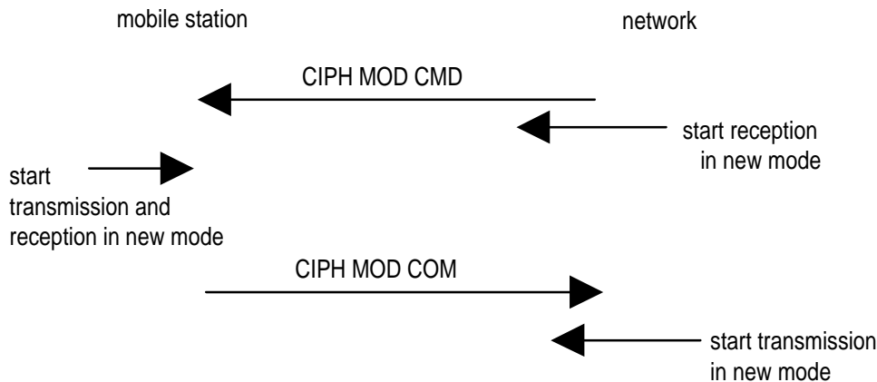
Figure 3.4.7.2.1/3GPP TS 04.18: Cipherring mode setting sequence
