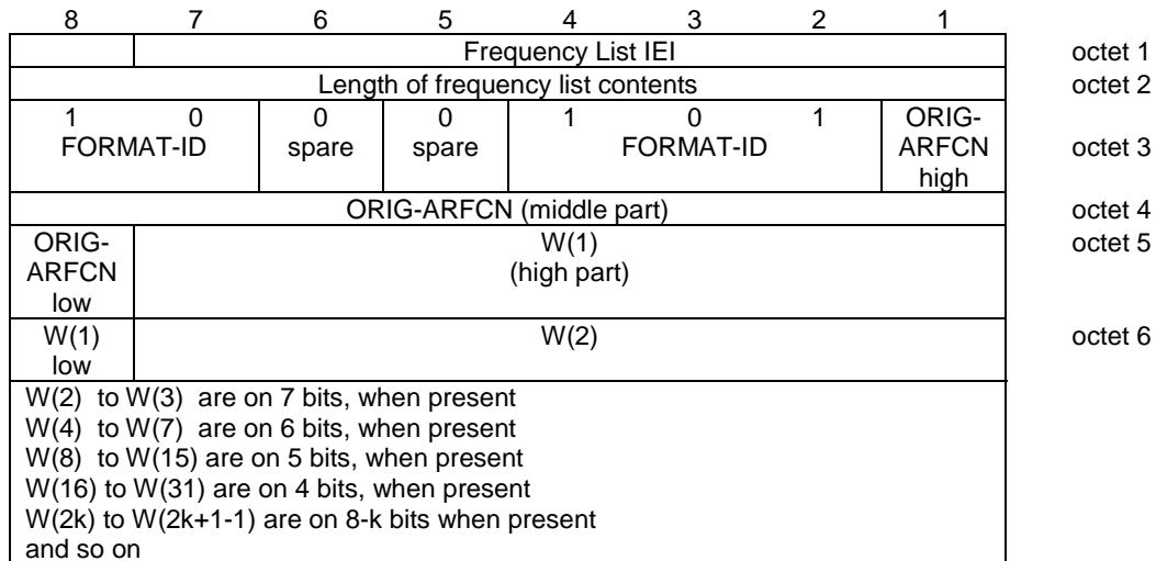
Figure 10.5.2.13.5.1/3GPP TS 04.18: Frequency List information element (Range 256 format)
