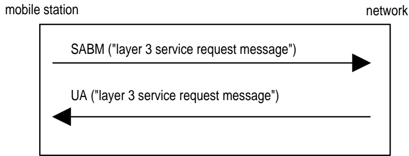
Figure 3.1.5.1/3GPP TS 04.18: Service request and contention resolution
