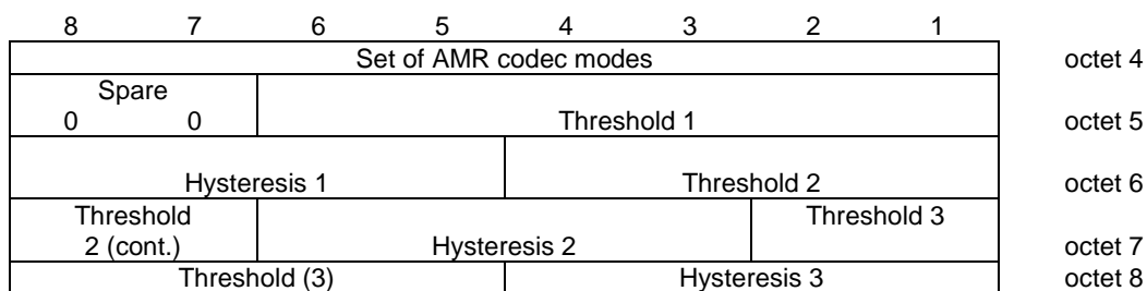
Figure 10.5.2.21aa.5/3GPP TS 04.18: Parameters for multirate speech field for the MR version 1 when a set of four modes is chosen
