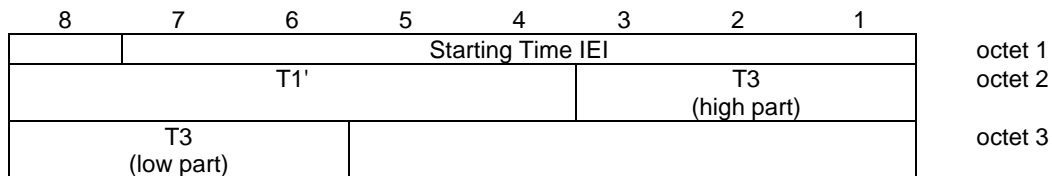
Figure 10.5.2.38.1/3GPP TS 04.18: Starting Time information element
