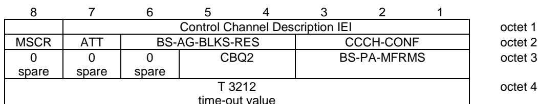
Figure 10.5.2.11.1/3GPP TS 04.18: Control Channel Description information element
