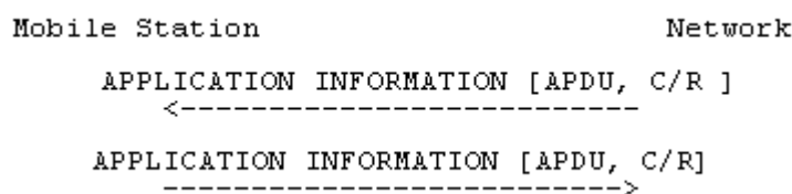
Figure 3.4.21.3.4.1/3GPP TS 04.18: Application Information Transfer without segmentation
