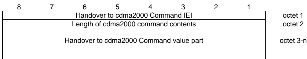
Figure 10.5.2.52.1/3GPP TS 04.18: Handover to cdma2000 Command information element
