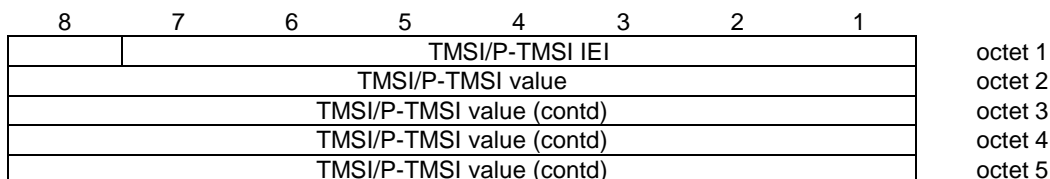
Figure 10.5.2.42.1/3GPP TS 04.18: TMSI/P-TMSI information element
