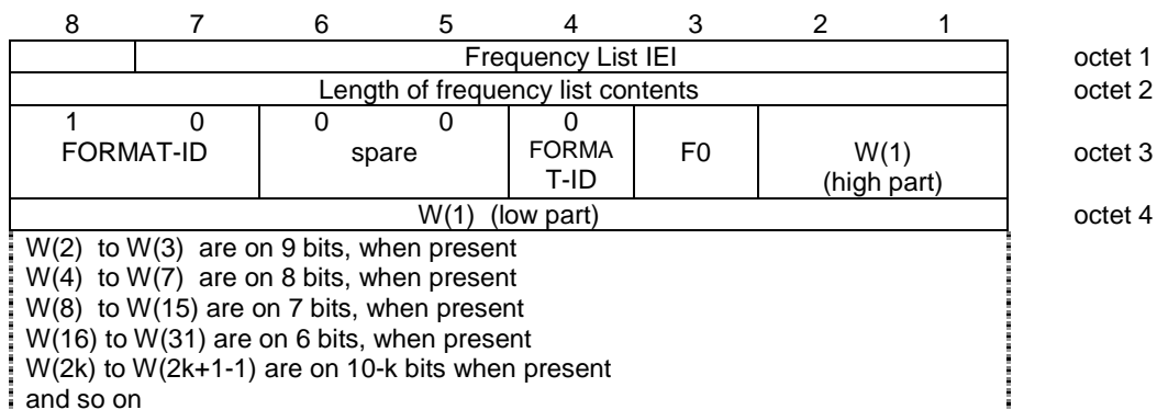
Figure 10.5.2.13.3.1/3GPP TS 04.18: Frequency List information element (Range 1024 format)
