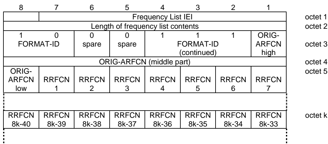
Figure 10.5.2.13.7.1/3GPP TS 04.18: Frequency List information element, variable bit map format
