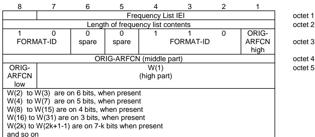
Figure 10.5.2.13.6.1/3GPP TS 04.18: Frequency List information element (Range 128 format)
