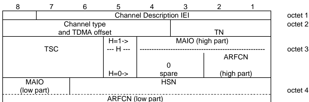
Figure 10.5.2.5.1/3GPP TS 04.18: Channel Description information element
