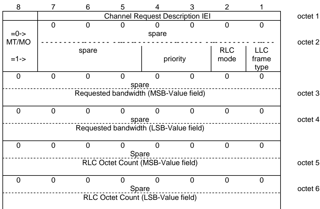
Figure 10.5.2.8a.1/3GPP TS 04.18: Channel Request Description information element
