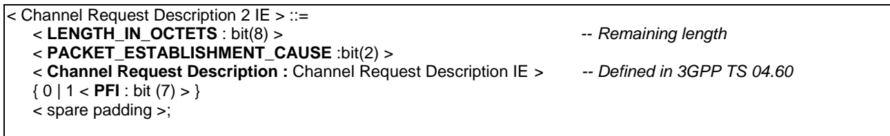
Figure 10.5.2.8b.1/3GPP TS 04.18: Channel Request Description 2 information element
