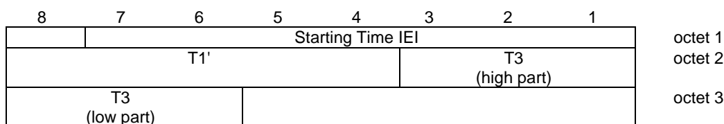
Figure 10.5.2.38.1/3GPP TS 04.18: Starting Time information element
