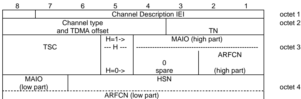
Figure 10.5.2.5a.1/3GPP TS 04.18: Channel Description 2 information element
