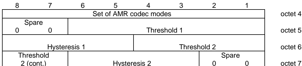
Figure 10.5.2.21aa.4/3GPP TS 04.18: Parameters for multirate speech field for the MR version 1 when a set of three codec modes is chosen
