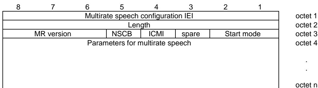
Figure 10.5.2.21aa.1/3GPP TS 04.18: MultiRate configuration information element
