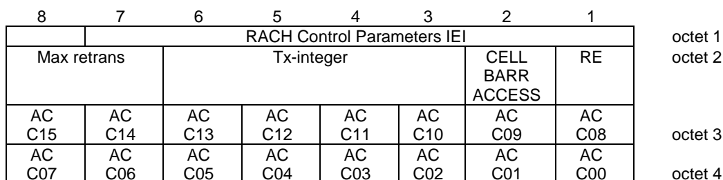
Figure 10.5.2.29.1/3GPP TS 04.18: RACH Control Parameters information element
