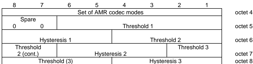
Figure 10.5.2.21aa.5/3GPP TS 04.18: Parameters for multirate speech field for the MR version 1 when a set of four modes is chosen
