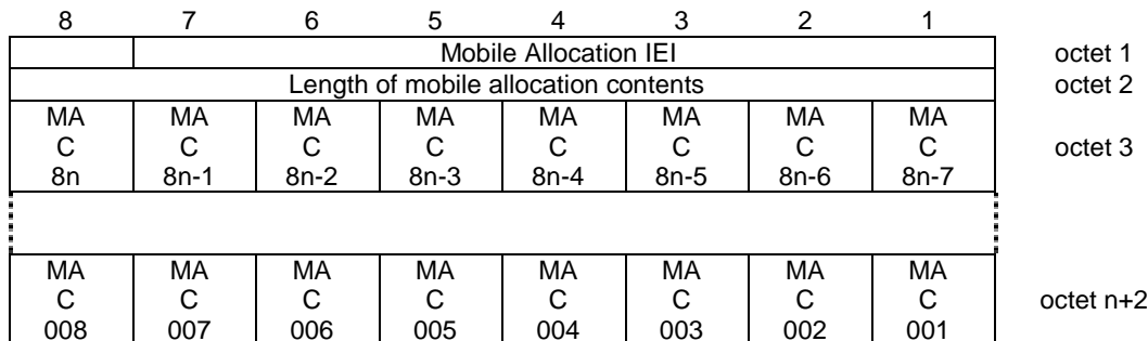
Figure 10.5.2.21.1/3GPP TS 04.18: Mobile Allocation information element
