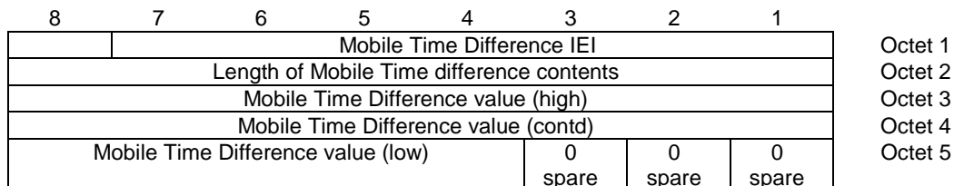
Figure 10.5.2.21a.1/3GPP TS 04.18: Mobile Time Difference information element
