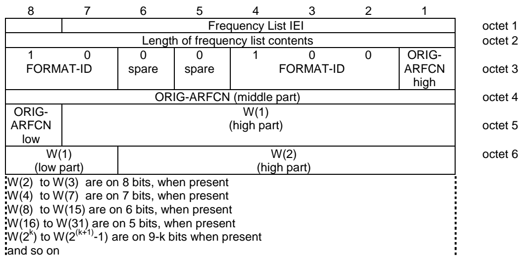
Figure 10.5.2.13.4.1/3GPP TS 04.18: Frequency List information element (Range 512 format)
