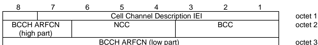
Figure 10.5.2.2.1/3GPP TS 04.18: Cell Description information element
