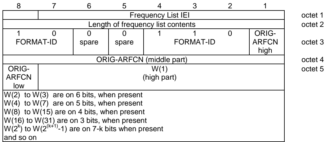
Figure 10.5.2.13.6.1/3GPP TS 04.18: Frequency List information element (Range 128 format)
