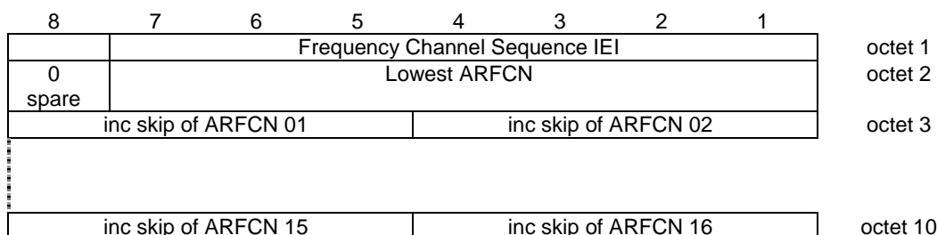
Figure 10.5.2.12.1/3GPP TS 04.18: Frequency Channel Sequence information element
