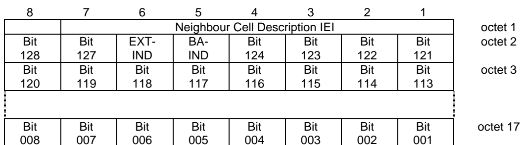
Figure 10.5.2.22.1/3GPP TS 04.18: Neighbour Cell Description information element
