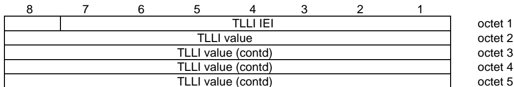
Figure 10.5.2.41a.1/3GPP TS 04.18: TLLI information element
