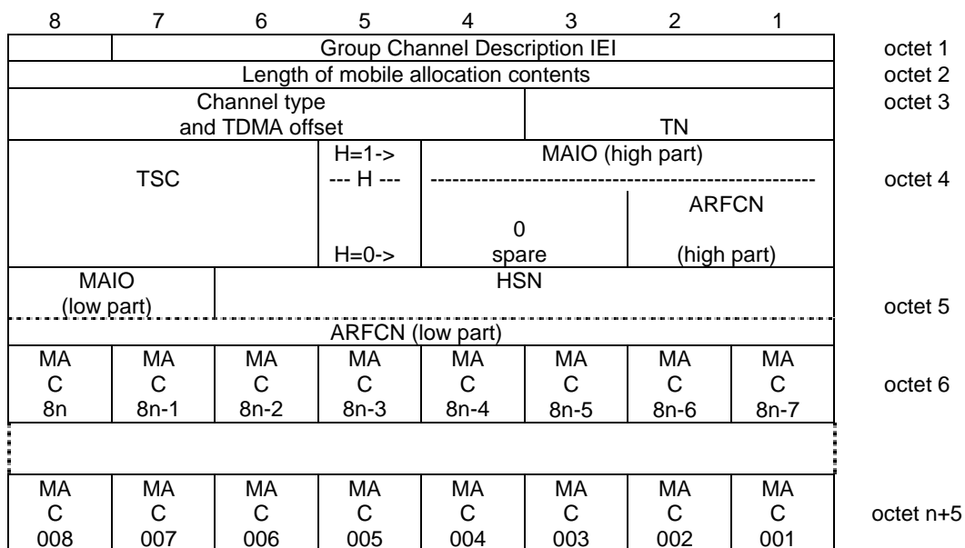
Figure 10.5.2.14b.1/3GPP TS 04.18: Group Channel Description information element
