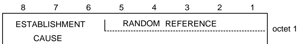
Figure 9.1.45.1/3GPP TS 04.18: UPLINK ACCESS message content
