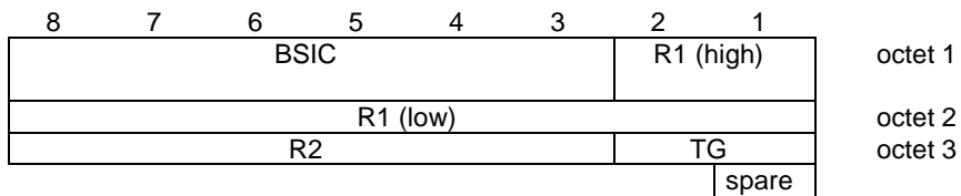
Figure 9.1.30b.1/3GPP TS 04.18: COMPACT Frame synchronization information element
