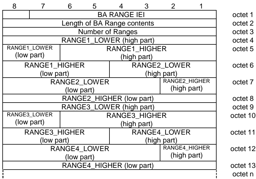
Figure 10.5.2.1a.1/3GPP TS 04.18: BA RANGE information element
