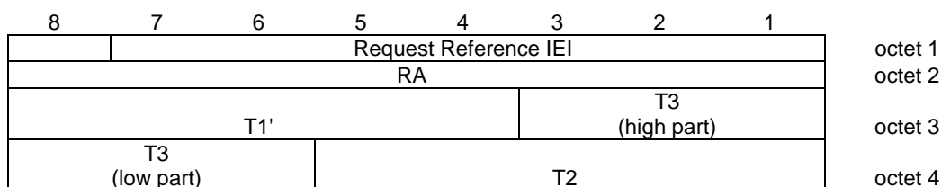
Figure 10.5.2.30.1/3GPP TS 04.18: Request Reference information element
