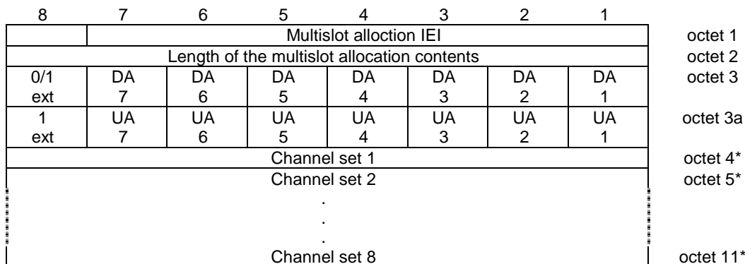
Figure 10.5.2.21b.1/3GPP TS 04.18: Multislot Allocation information element
