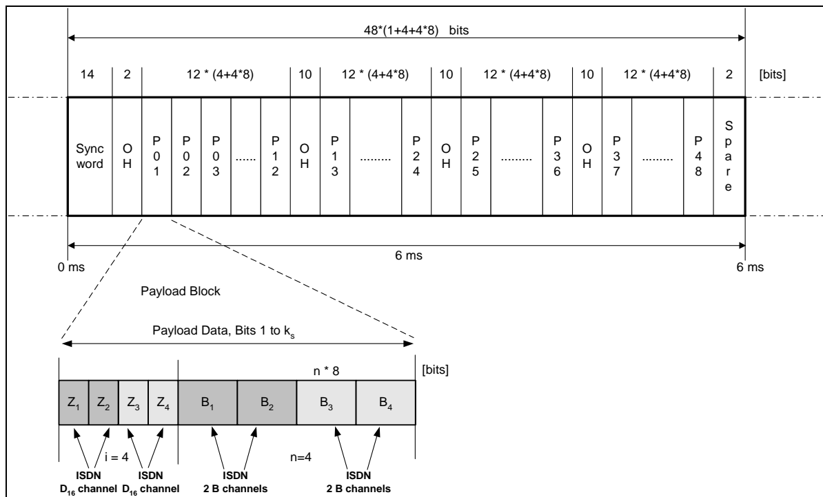
Figure A-4: Framing example: 2 x ISDN BRA
