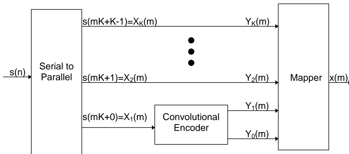
Figure 9-8: Block diagram of the UC-PAM encoder
