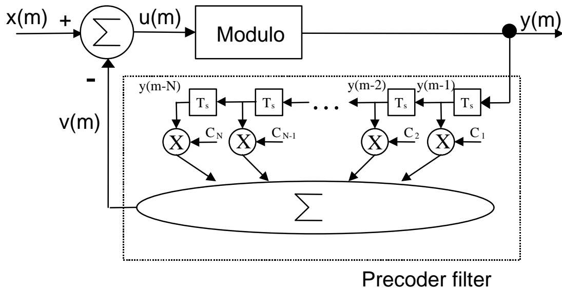
Figure 9-10: Block diagram of the channel precoder
