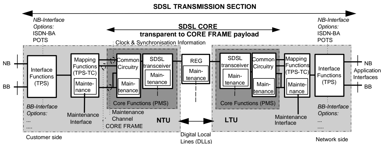
Figure 4-1: Reference configuration
