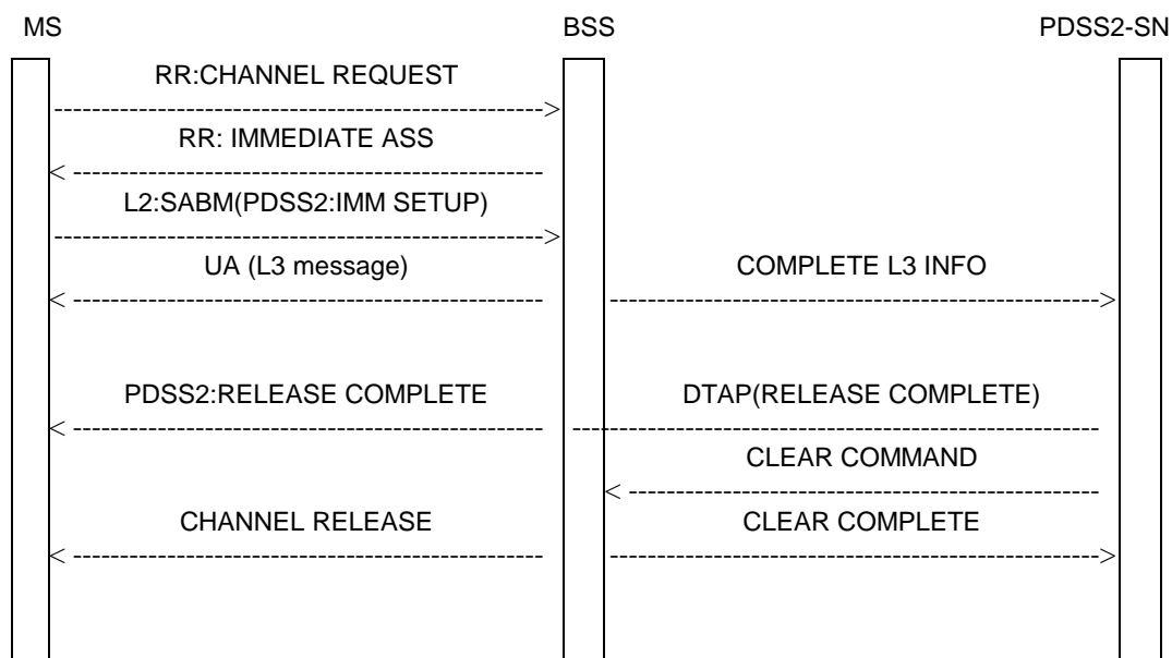
Figure 9: Signalling flow for PDSS2 (rejection of service)
