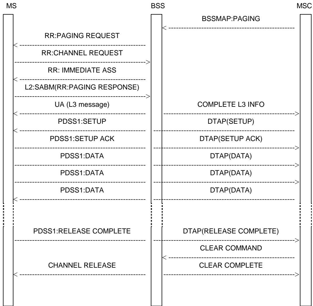
Figure 2: Signalling flow for mobile terminating PDSS1 (from idle mode, release by mobile station)
