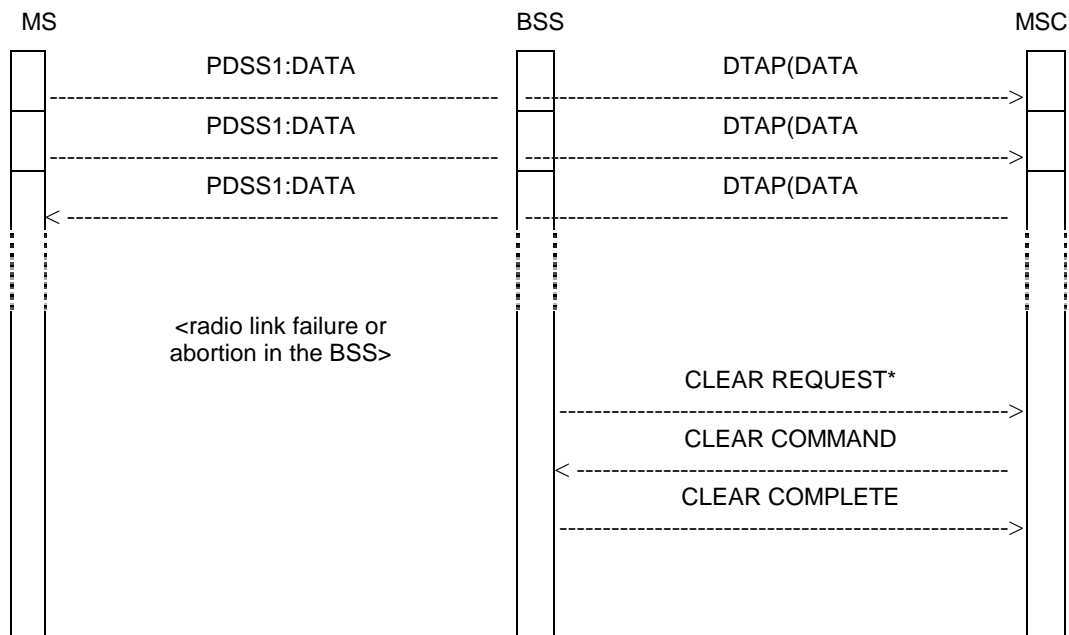
Figure 3: Signalling flow for PDSS1 (from PDSS1-connected mode: radio link failure or radio link abortion in the BSS)
