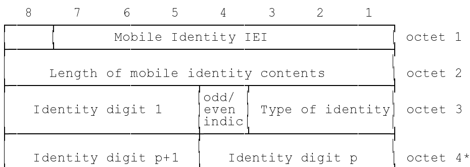
FIGURE 10.3/GSM 04.63 Mobile Identity 2 information element
