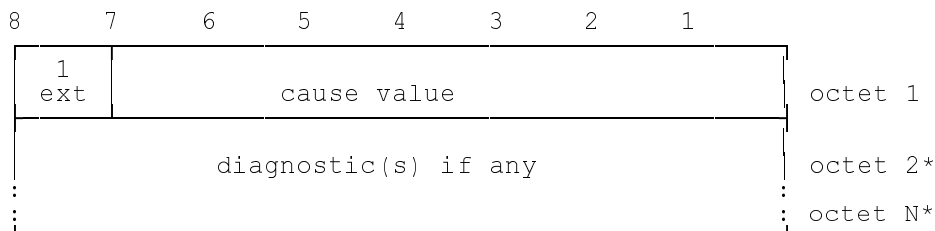
FIGURE 10.2/GSM 04.63 cause information element
