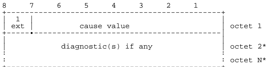
FIGURE 10.2/GSM 04.63 cause information element
