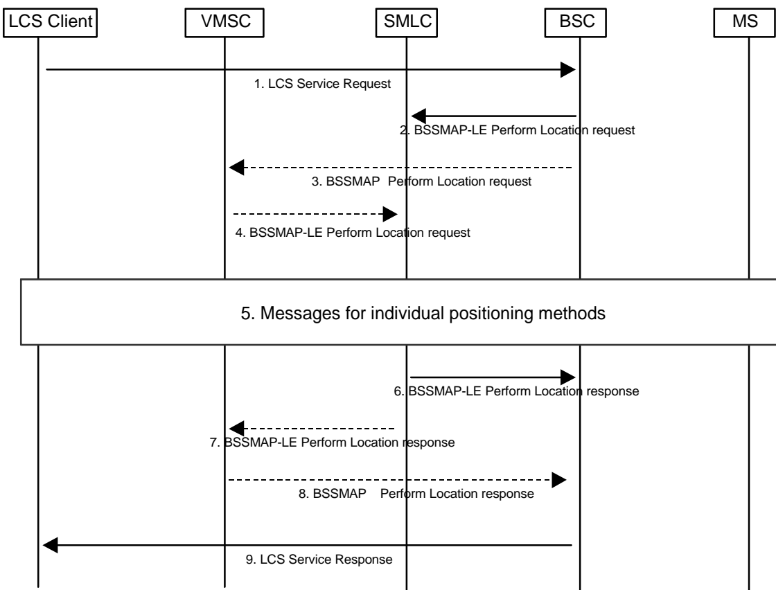
Figure 32: Network Induced Location Request from a Serving BSC
