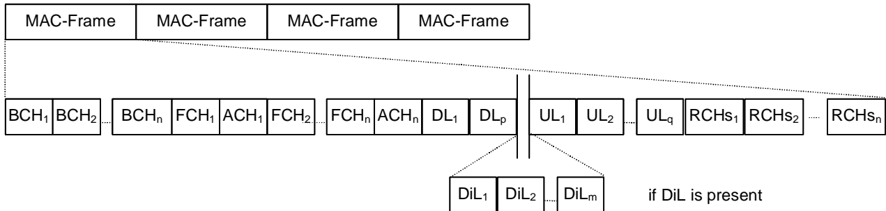
Figure 8: Basic MAC frame structure for multiple sectors (N = number of sector used by the AP)
