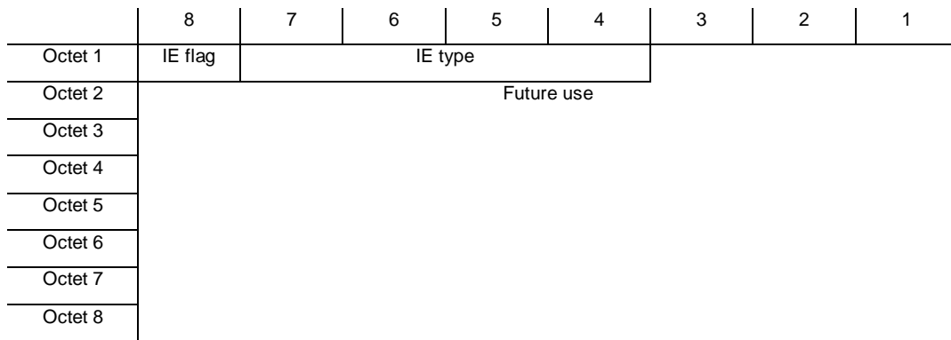
Figure 18: Transfer Syntax of the RG for empty parts in a MAC frame
