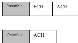
Figure 58: Possible FCH-and-ACH PDU trains
