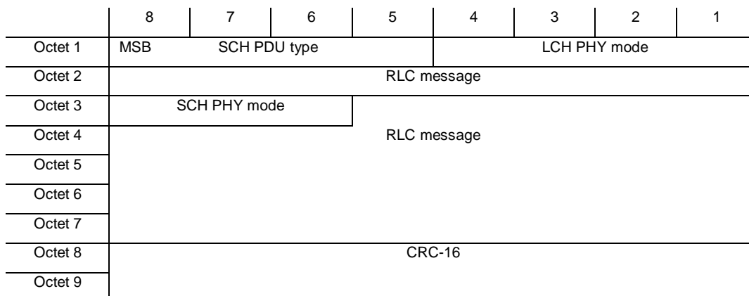
Figure 32: Transfer syntax of uplink RLC messages in SCHs
