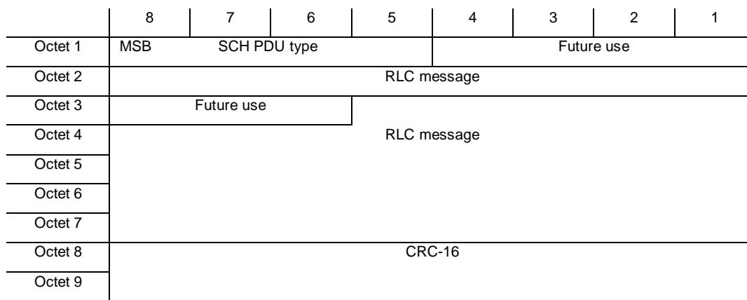
Figure 22: Transfer syntax of the downlink RLC message in an SCH
