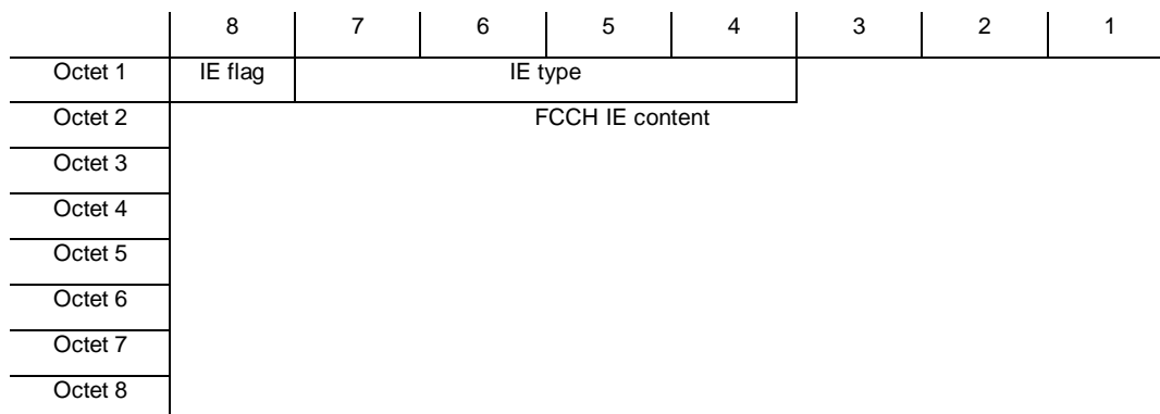
Figure 10: FCH transfer syntax
