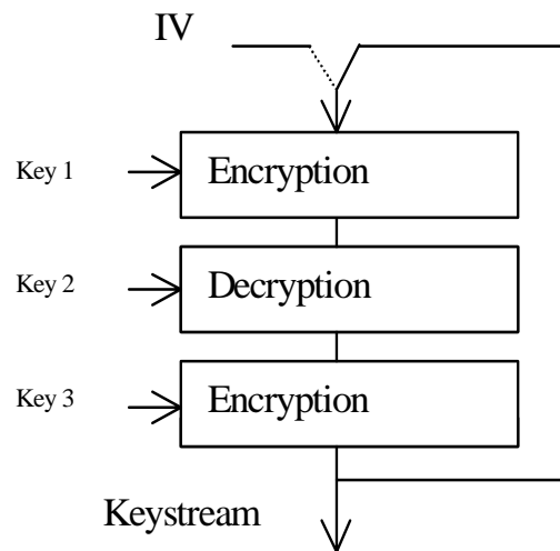
Figure 49: TripleDES encryption in OFB mode
