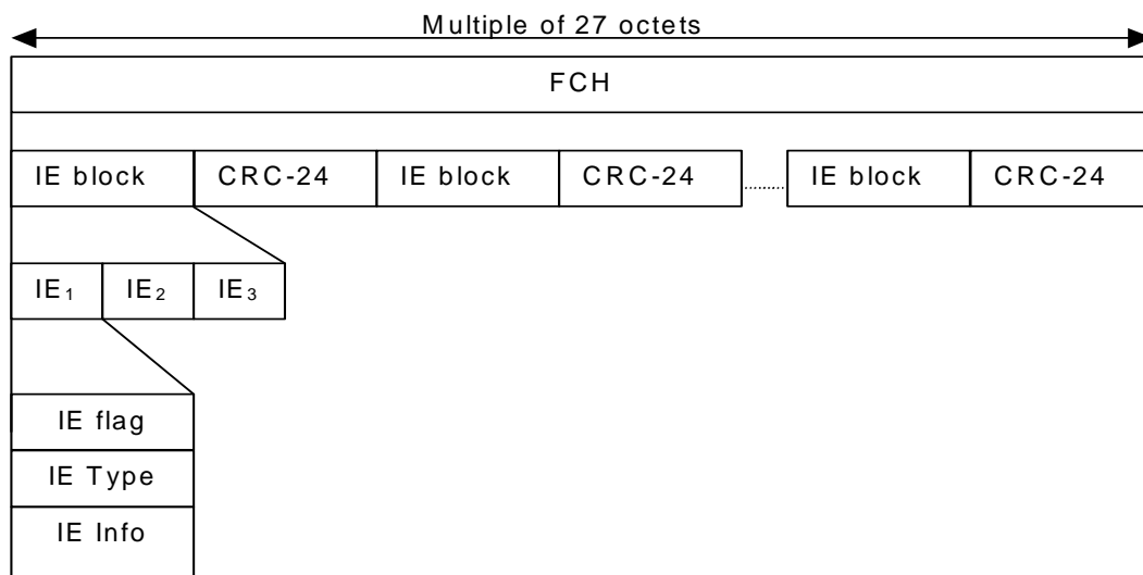
Figure 9: FCH structure
