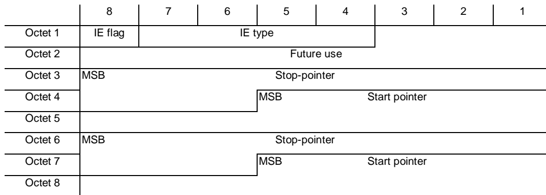
Figure 17: Transfer Syntax of the RG for empty parts in a MAC frame
