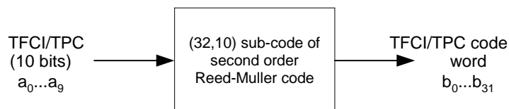
Figure 10: Channel coding of TFCI / TPC information bits
