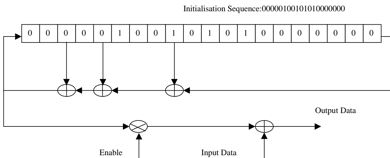
Figure 9: Scrambler operation
