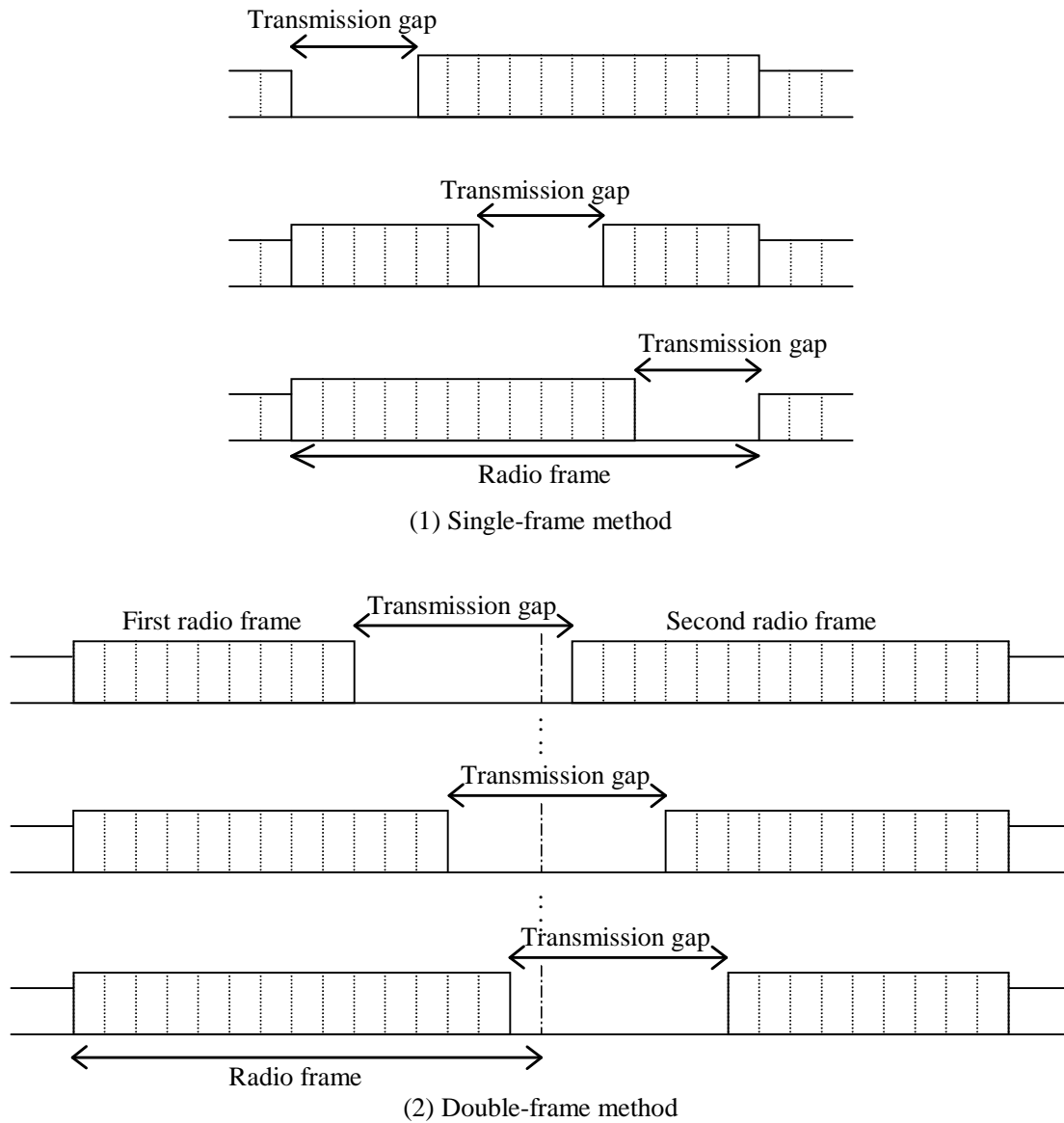
Figure 16: Transmission gap positions with different N_{\text{first}}
