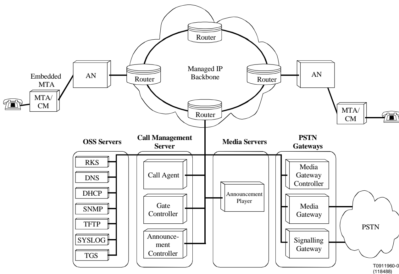
Figure 3: IP-Cablecom component reference model
