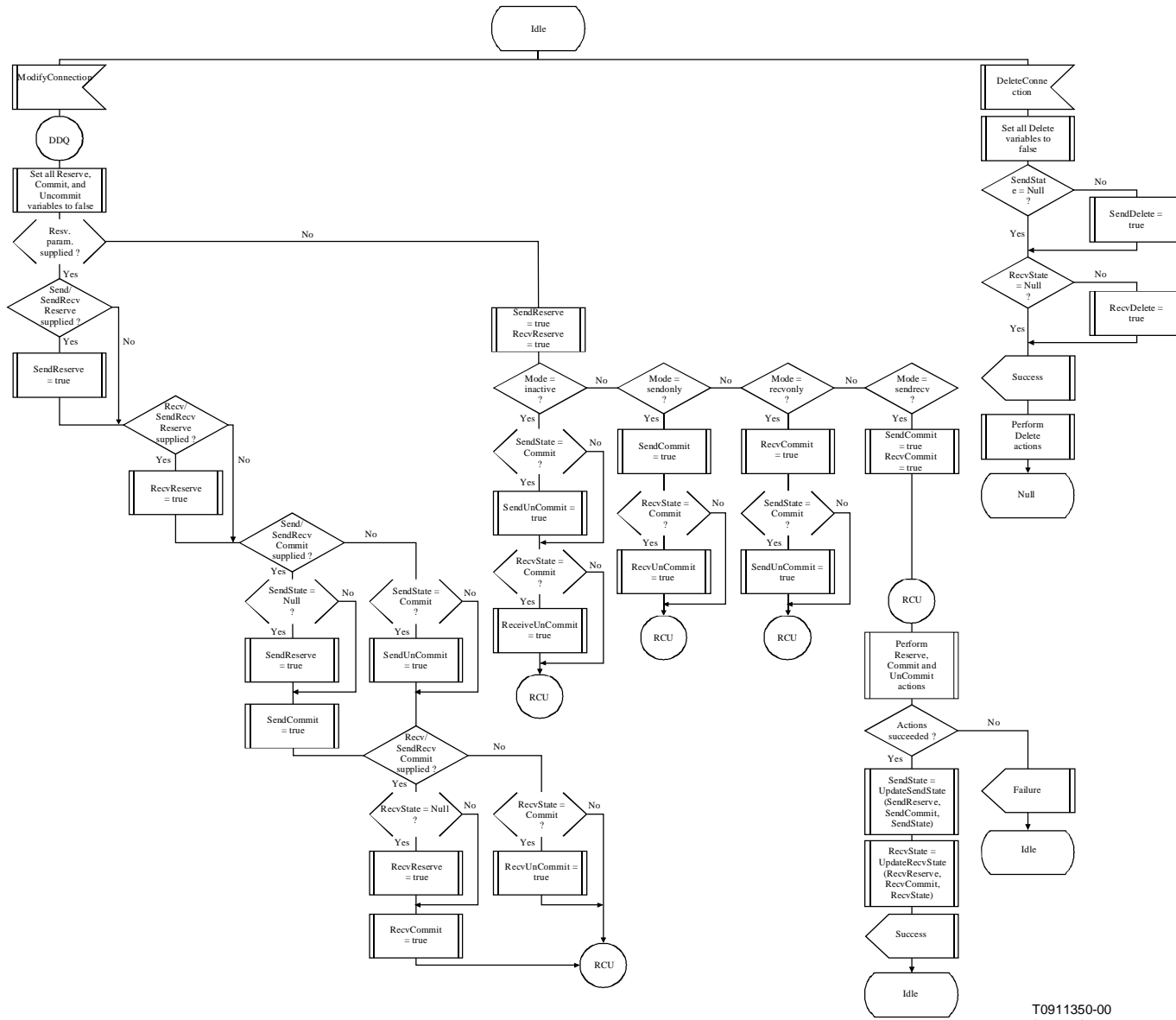
Figure B.2: NCS/D-QoS state diagram (2:2)
