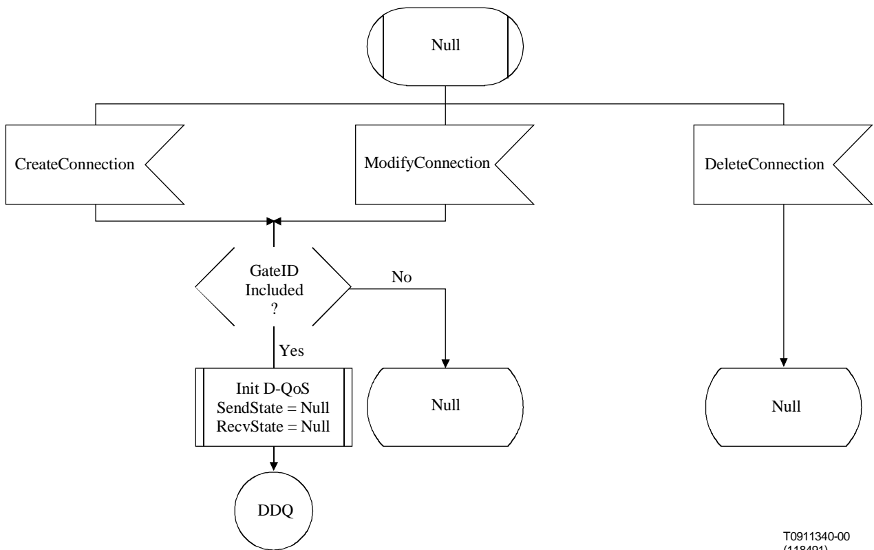
Figure B.1: NCS/D-QoS state diagram (1:2)
