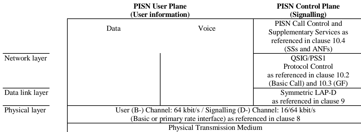
Figure 2: Protocol Stack
