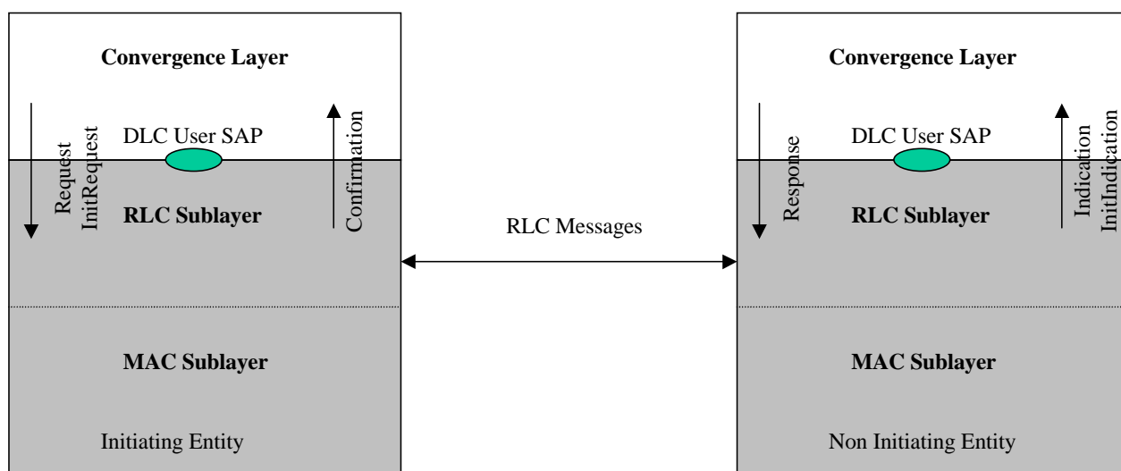
Figure 54: Use of primitives
