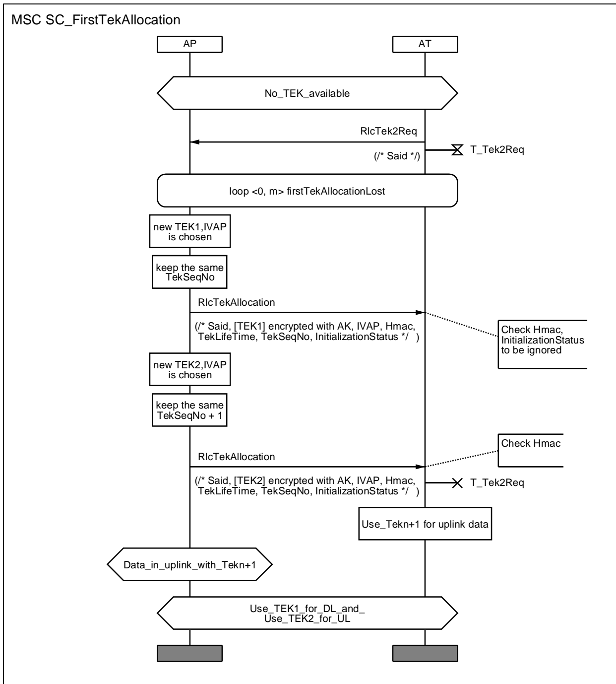
Diagram 25: MSC for first TEK requests
