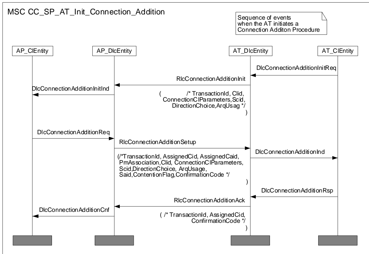
Diagram 30: MSC (4 entities) for AT initiated connection set up
