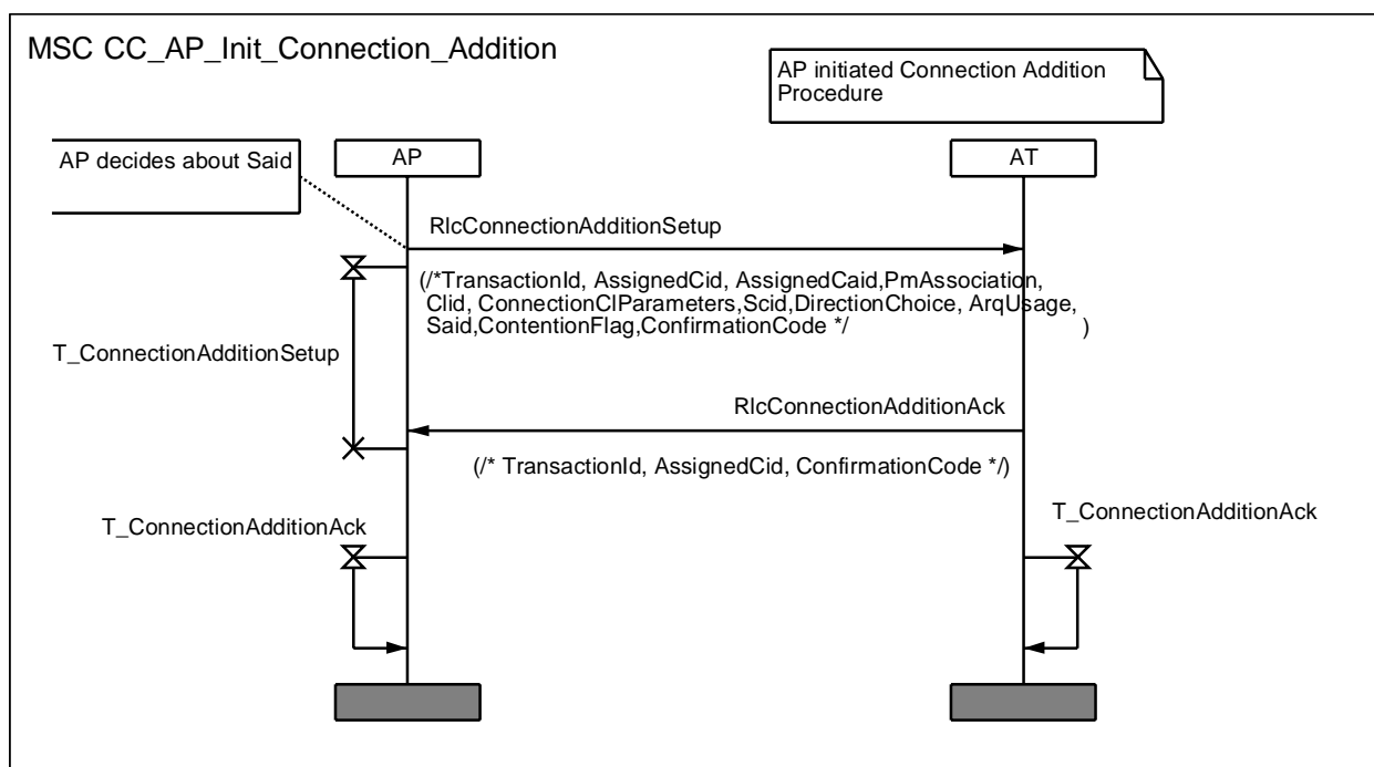
Diagram 37: MSC for AP initiated Connection Establishment
