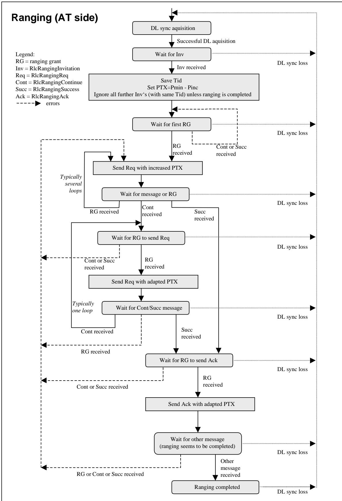
Diagram 8: State diagram for ranging (AT side)
