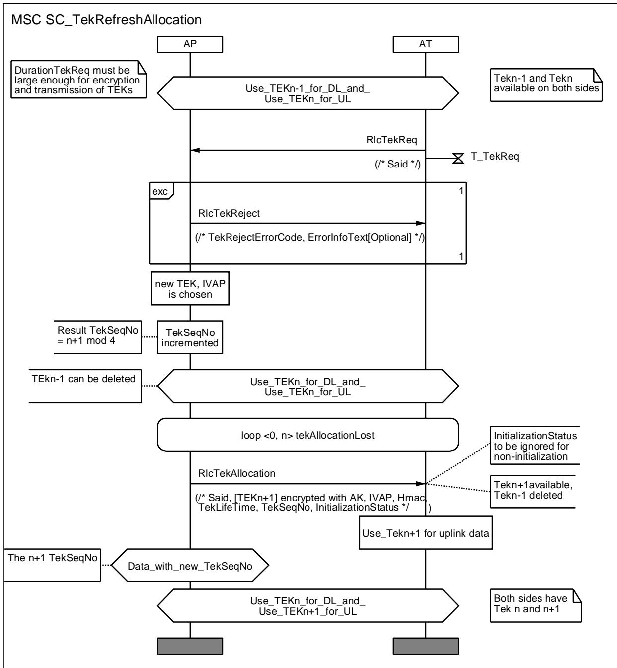
Diagram 27: MSC for key renewal before life time expiration
