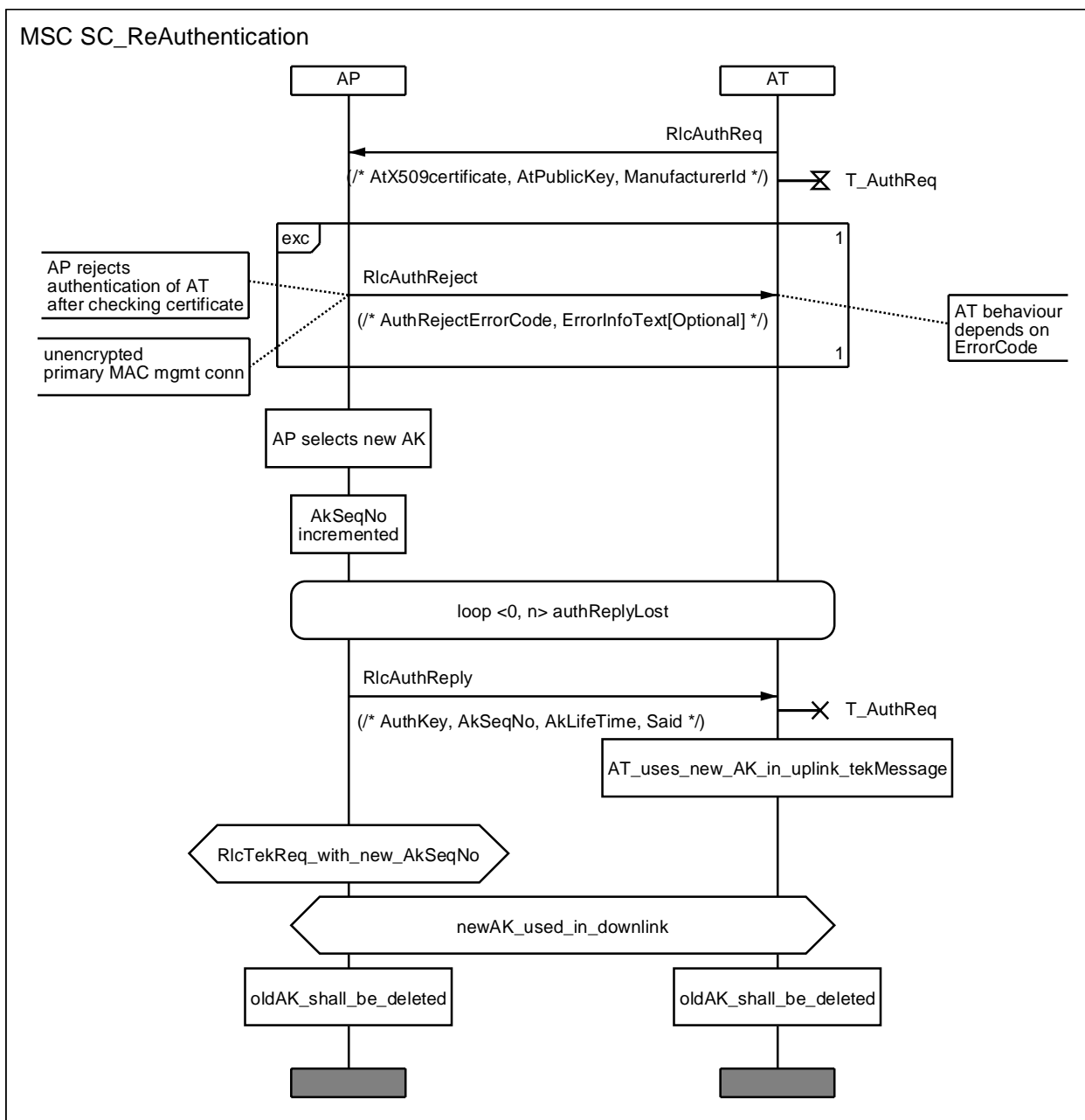
Diagram 24: MSC for re-authorization of AT before AK lifetime expiration
