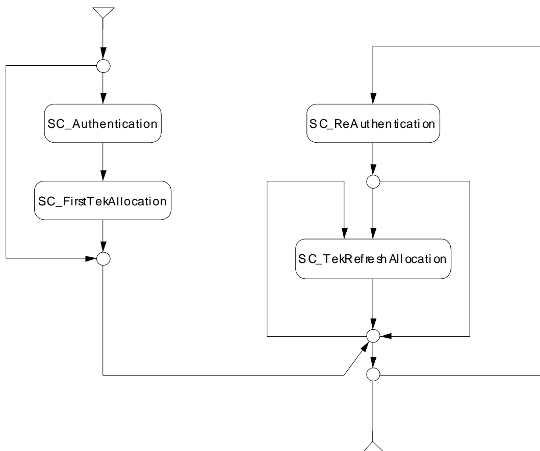
Figure 49: HMSC for security overview
