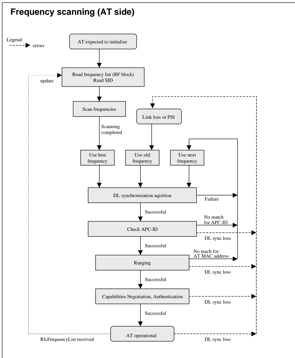
Figure 44: Frequency scanning in the context of initialization steps
