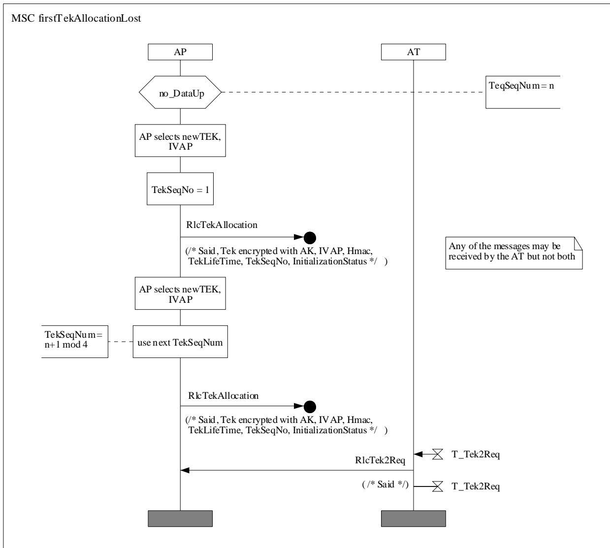
Diagram 26: MSC for retransmission in case of RlcTekAllocation loss during first initialization
