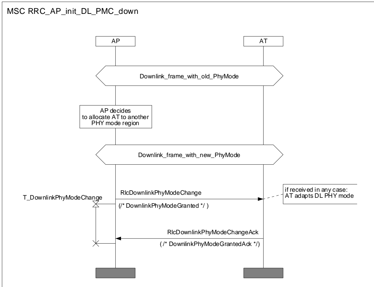
Diagram 18: MSC for AP initiated DL PHY mode change (to a more robust mode)
