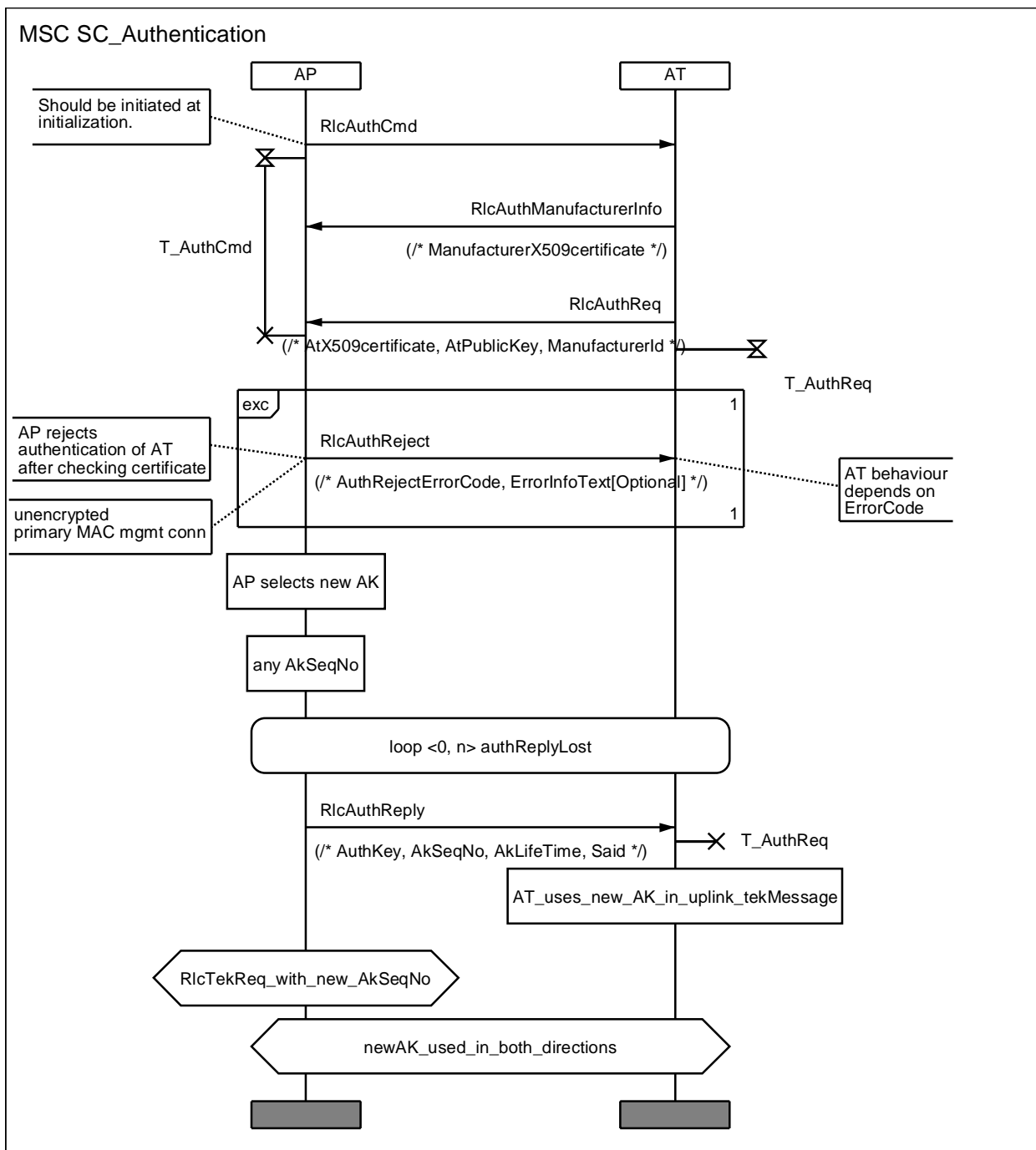
Diagram 22: MSC for successful initial authentication
