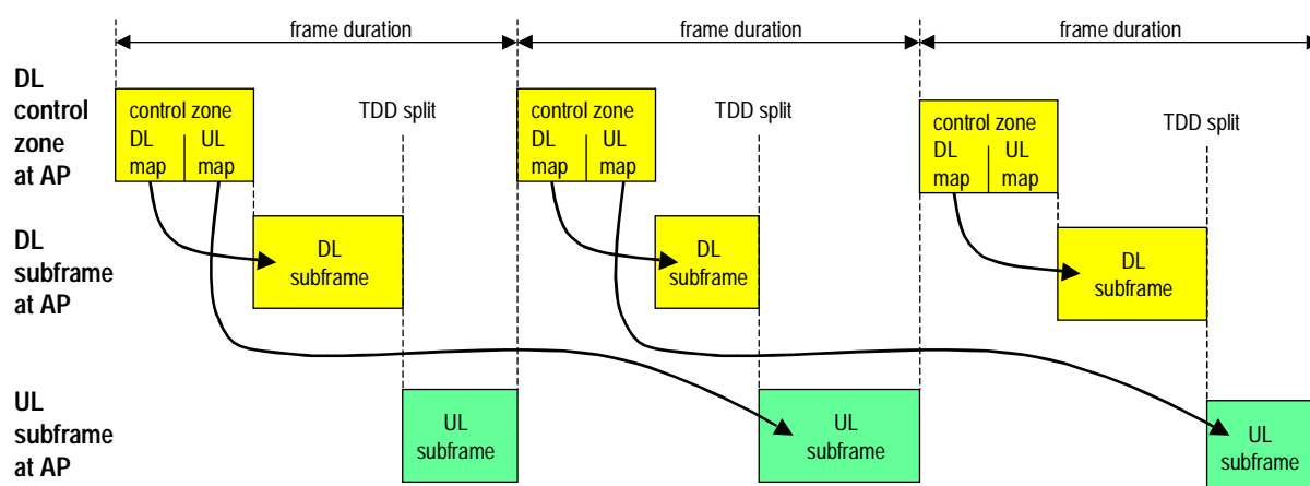
Figure 36: Maximum time relevance for UL map (TDD mode)
