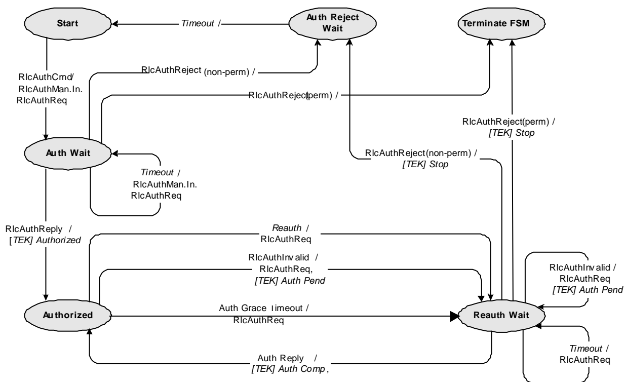
Figure 51: Authorization finite state machine flow diagram (AT side)
