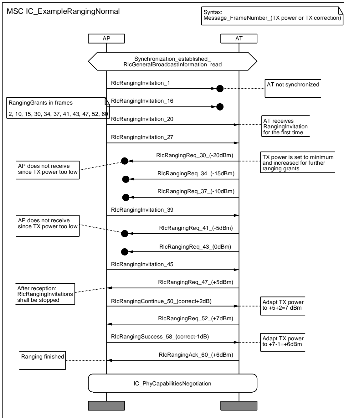
Diagram 6: MSC of a ranging example with many errors
