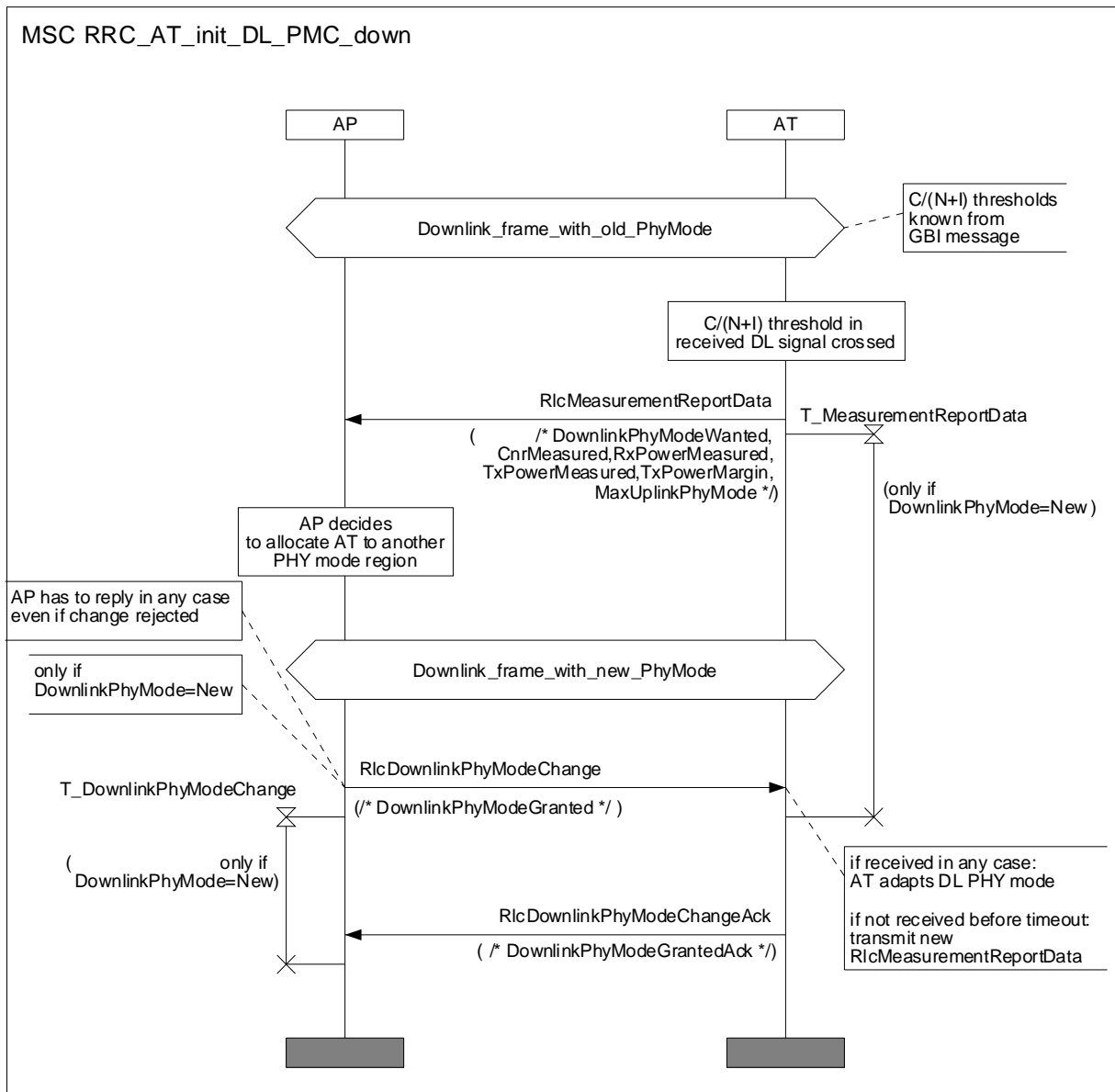
Diagram 16: MSC for AT initiated DL PHY mode change (to a more robust mode)
