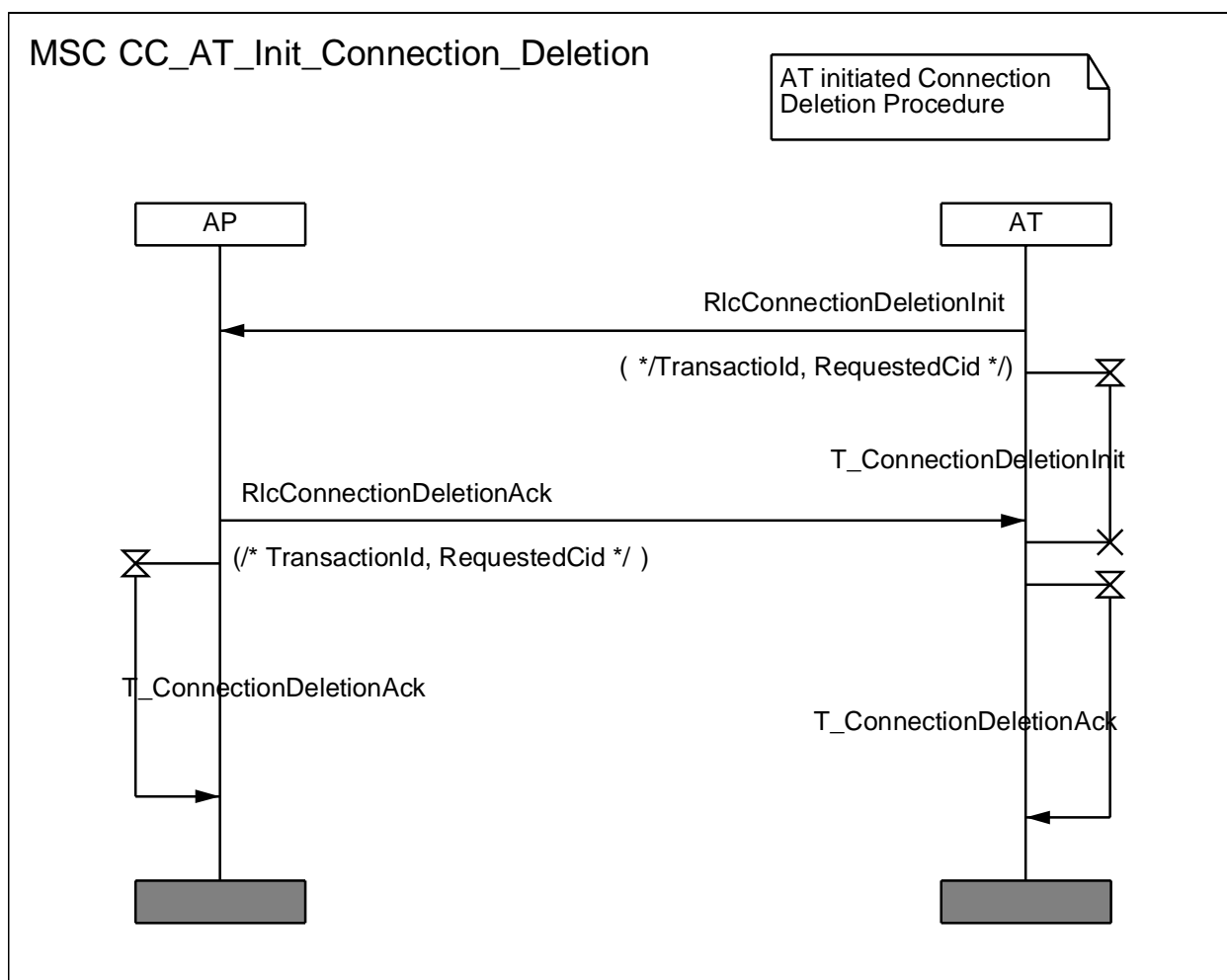
Diagram 40: MSC for AT initiated connection release
