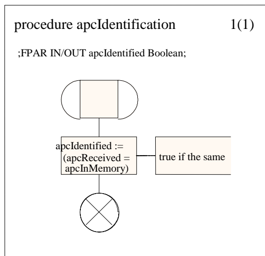
Figure 42: APC identification
