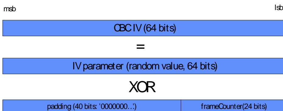
Figure 53: CBC IV generation
