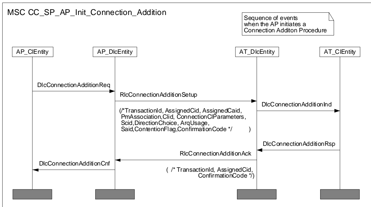
Diagram 31: MSC (4 entities) for AP initiated connection set up
