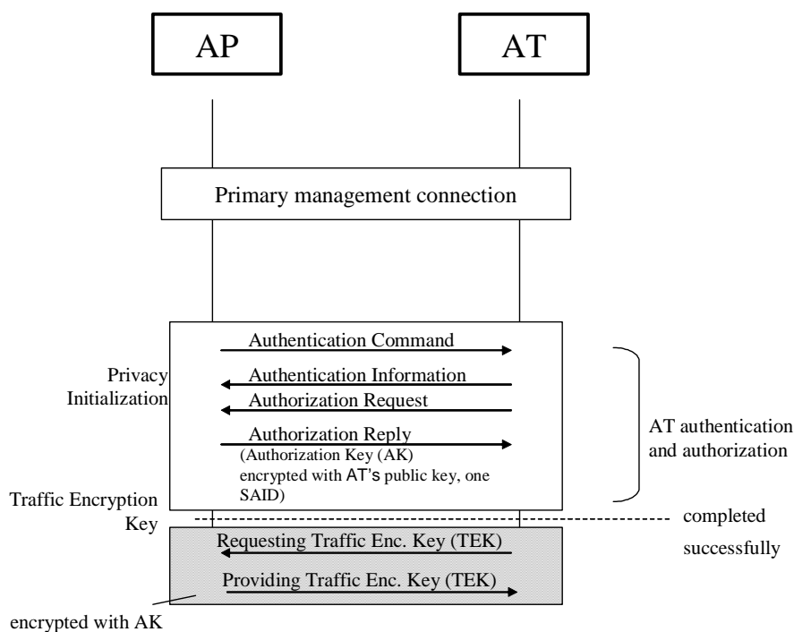
Figure 48: Illustration of the authentication and privacy initialization
