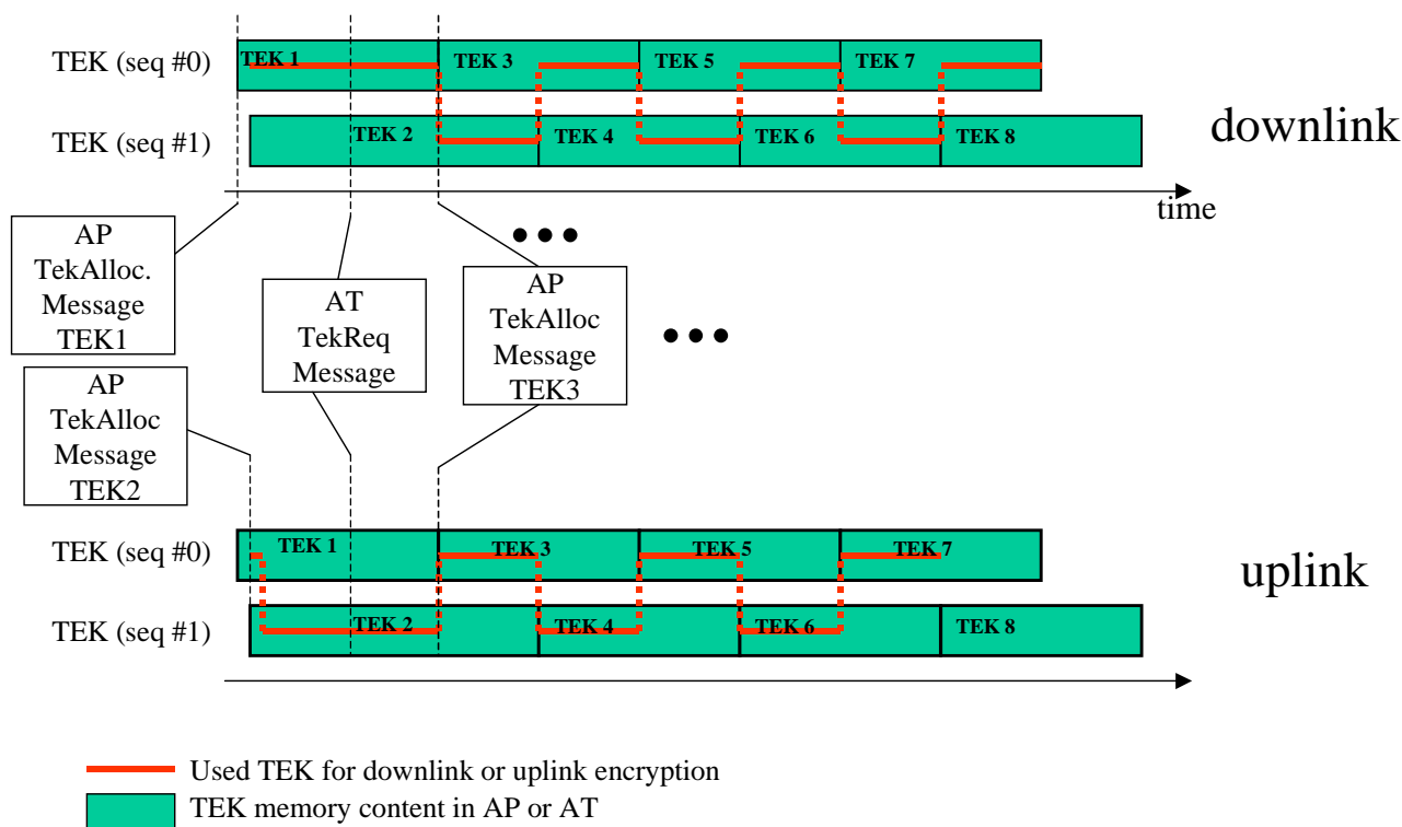
Figure 50: TEK lifetime and switch over (AT viewpoint)
