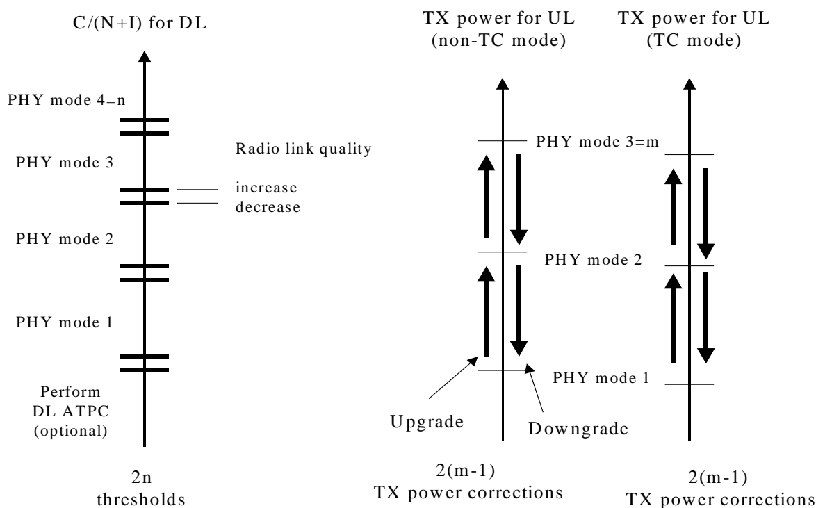
Figure 37: Parameters for PHY mode set description
