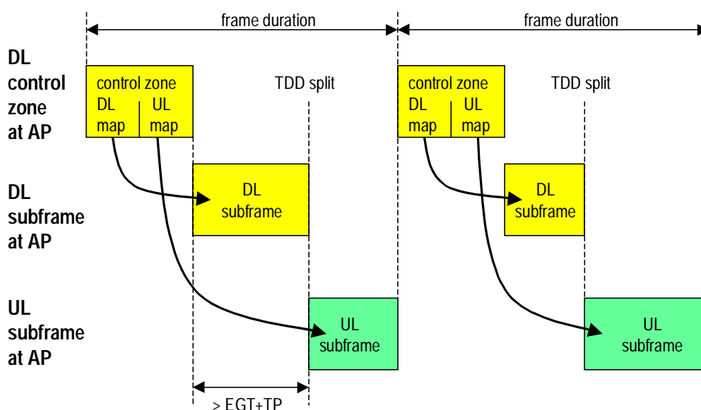
Figure 35: Minimum time relevance for UL map (TDD mode)
