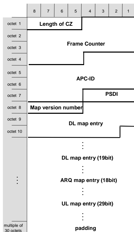
Figure 30: Bit structure of control zone (left bit transmitted first)
