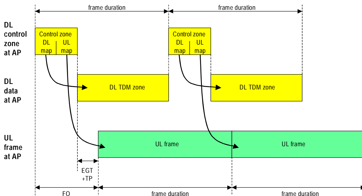
Figure 33: Minimum time relevance for UL map (FDD mode)
