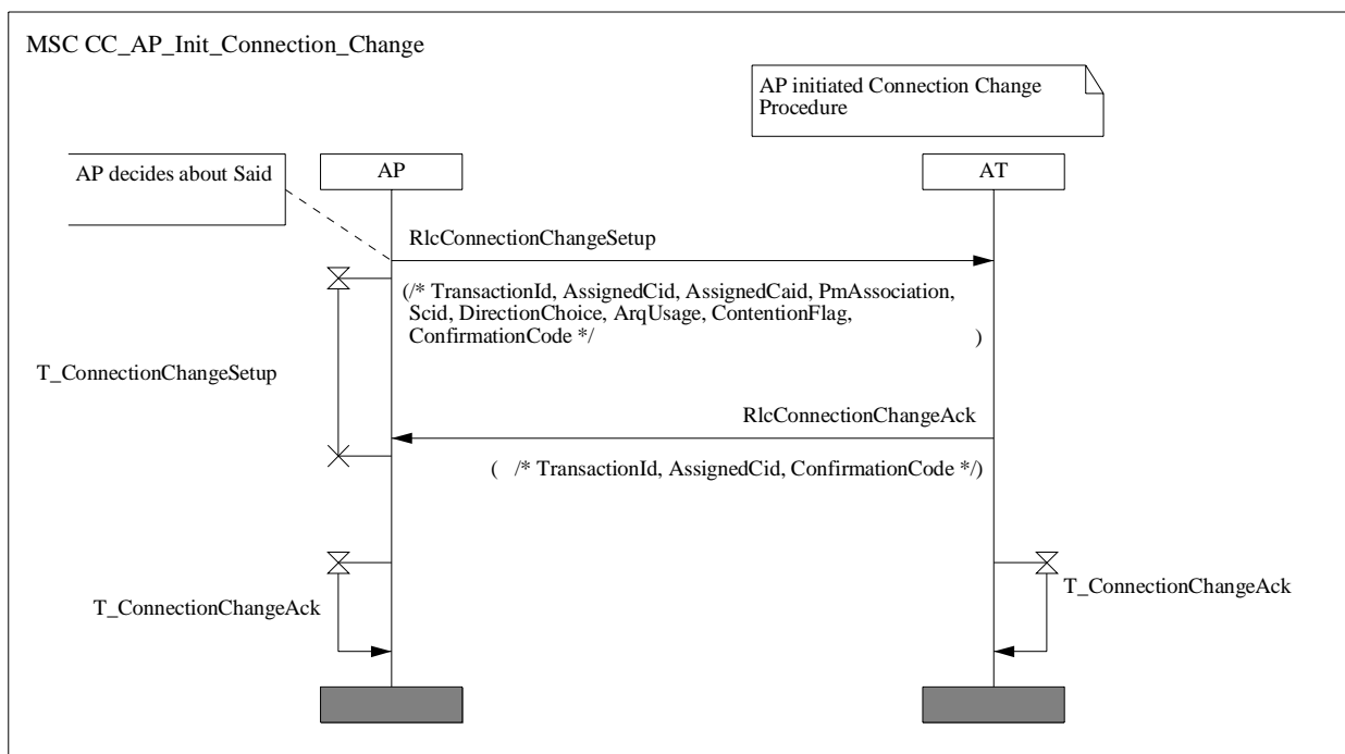
Diagram 39: MSC for AP initiated connection change
