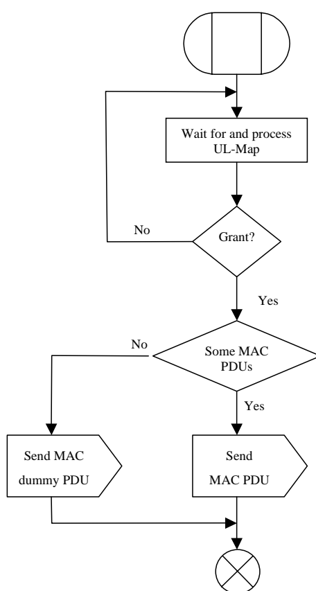
Figure 38: Grant per terminal
