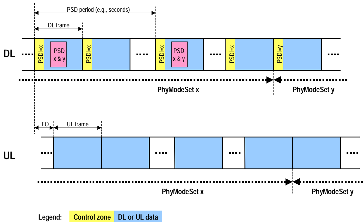
Figure 47: Change of PHY mode set
