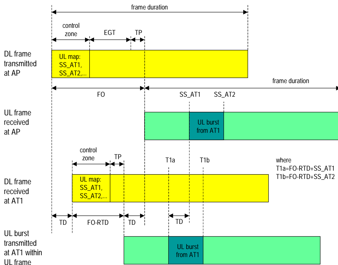
Figure 32: Starting times for UL bursts
