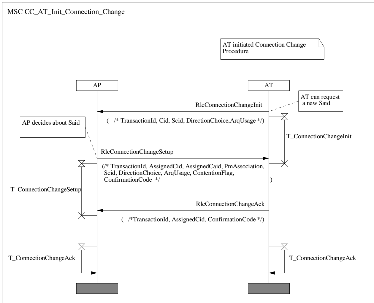
Diagram 38: MSC for AT initiated connection change
