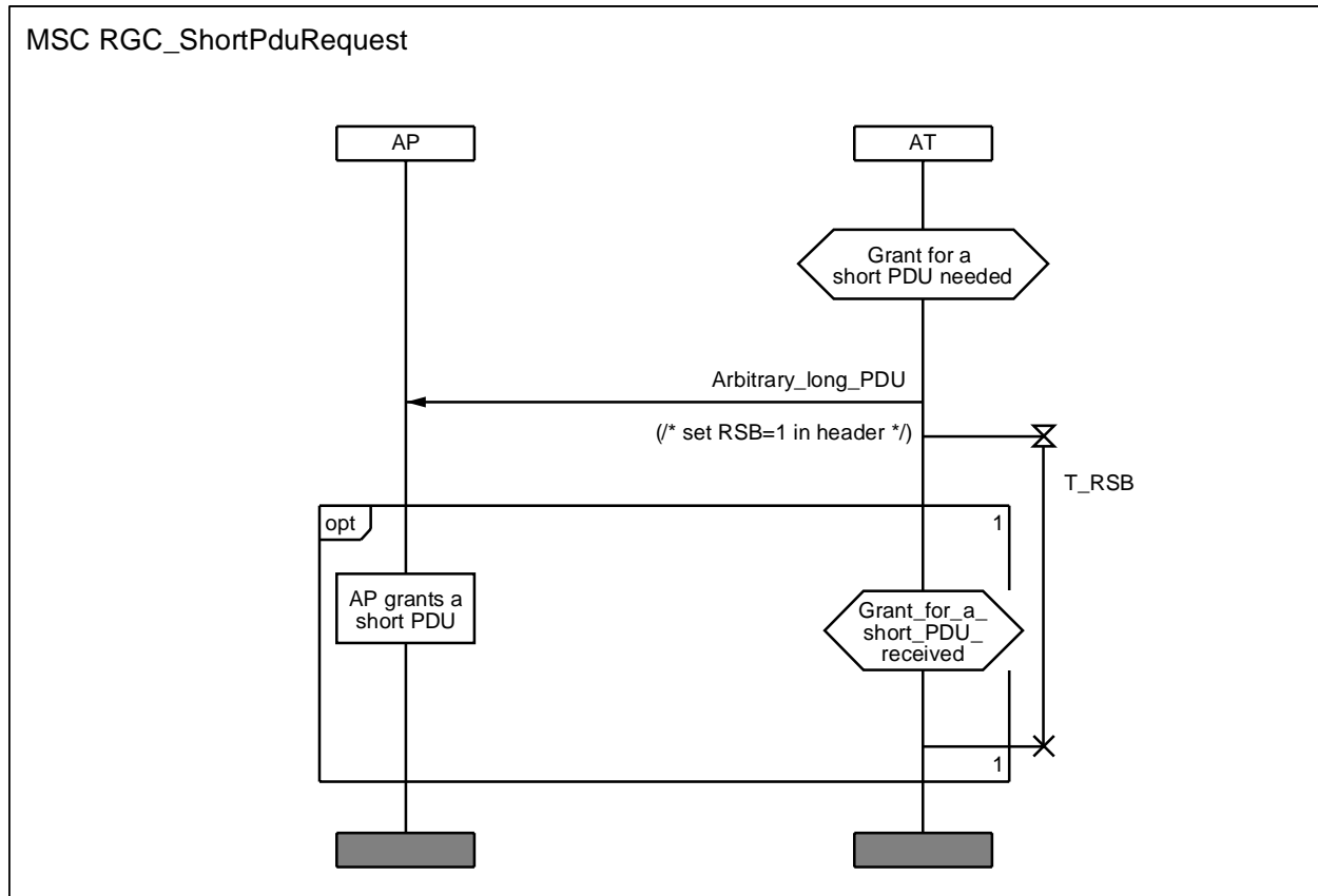
Diagram 1: MSC for the use of RSB
