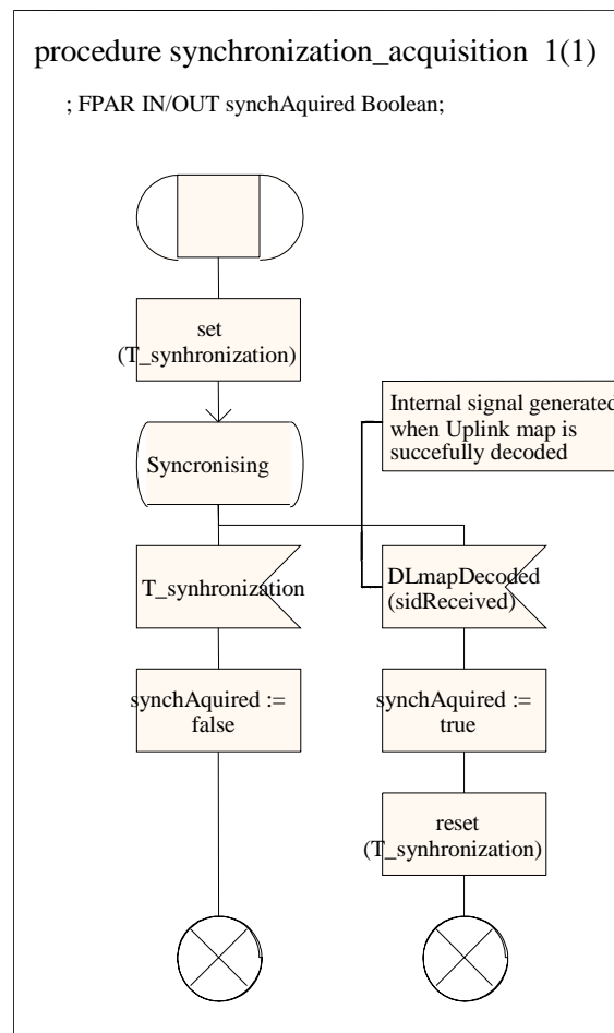
Figure 41: Synchronization acquisition
