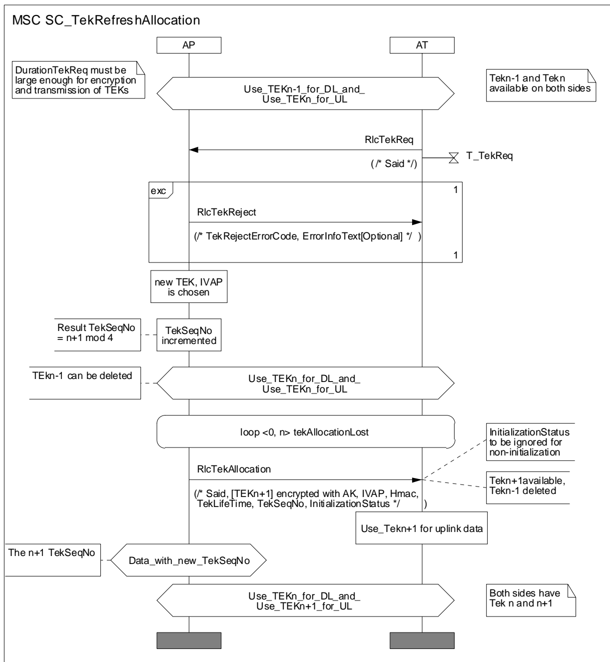
Diagram 29: MSC for TEK re-requesting due to loss of key request or key reply message
