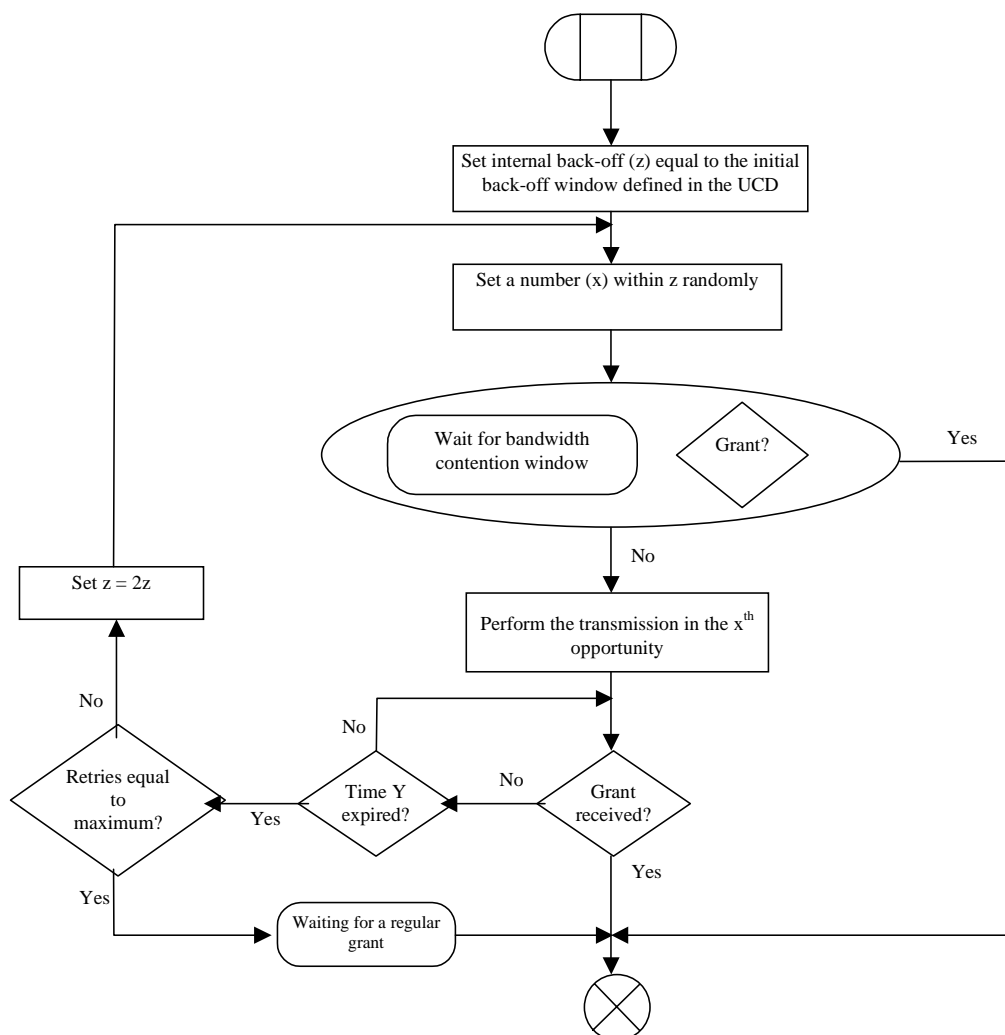
Figure 40: Contention algorithm for bandwidth request
