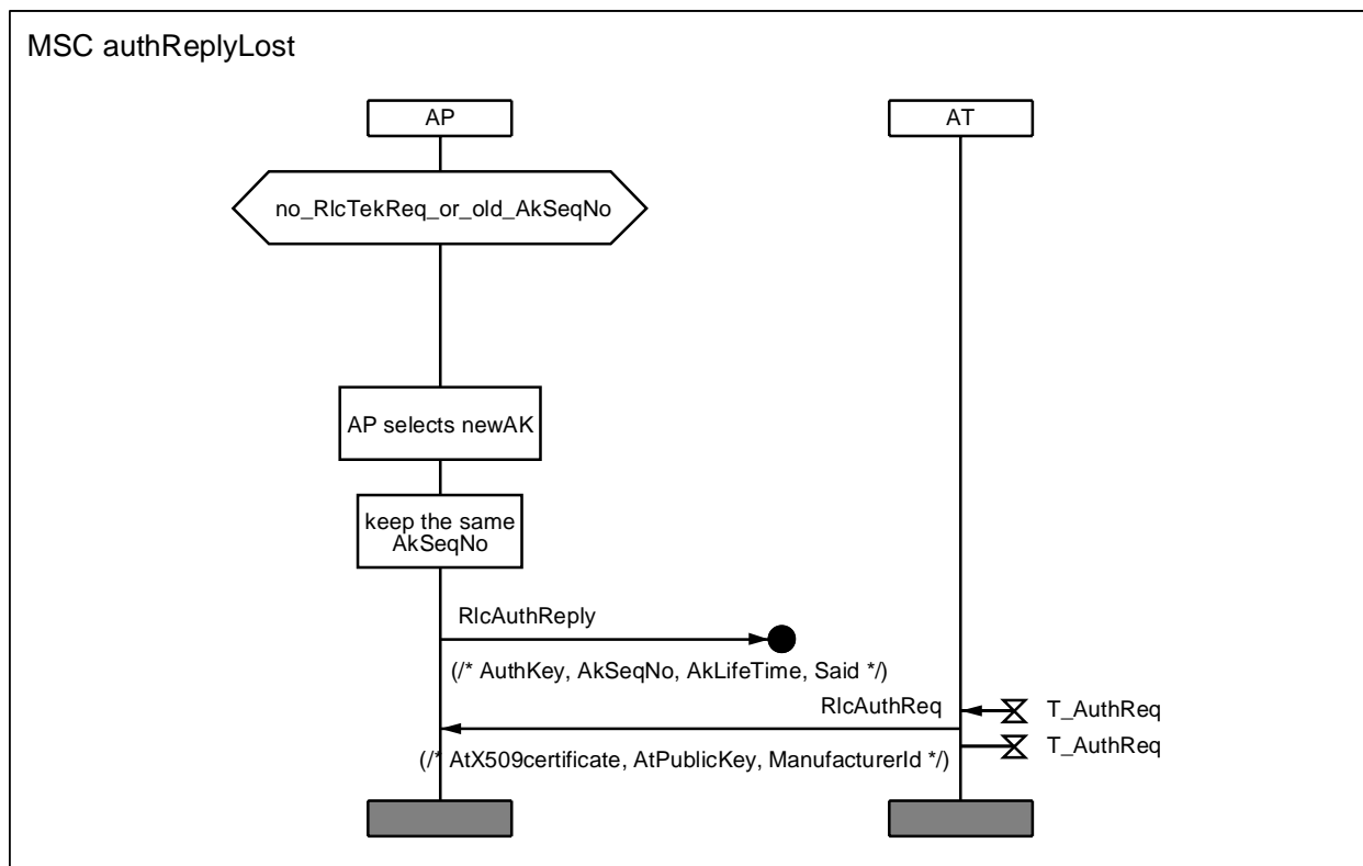
Diagram 23: MSC for retransmission in case of RlcAuthReply loss
