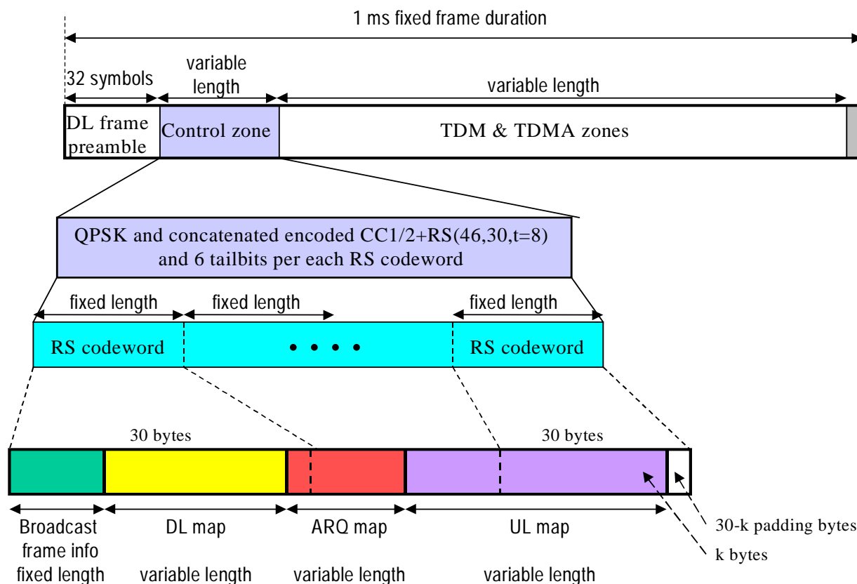
Figure 31: FEC protection of the control zone
