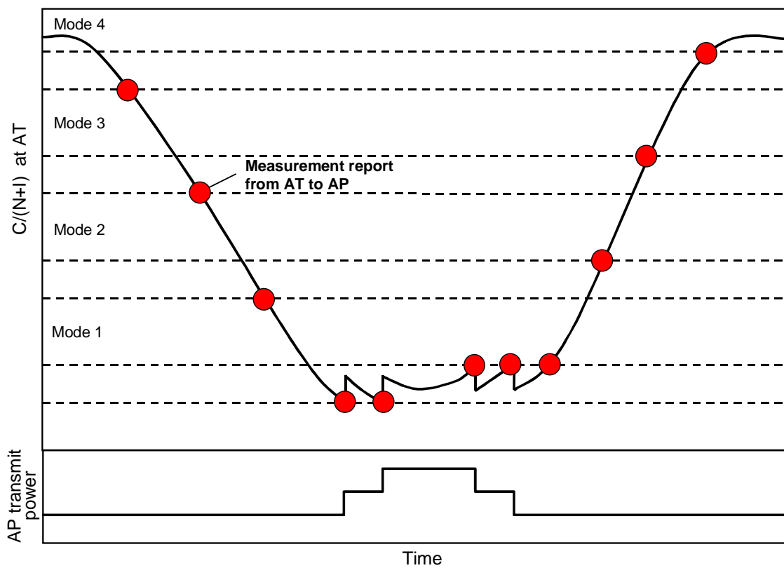
Figure 46: Exemplary illustration of the dynamic behaviour of DL ATPC
