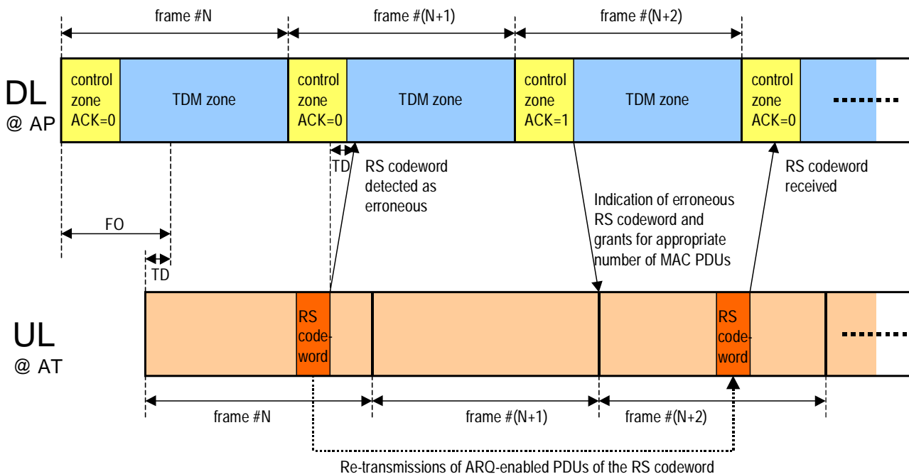
Figure 25: Relation between DL and UL frames for ARQ
