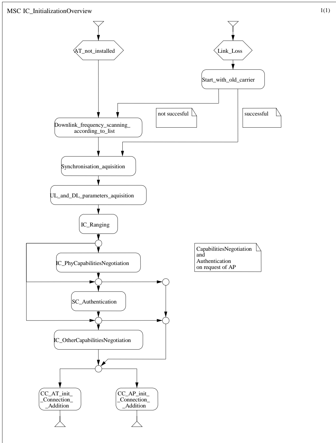
Diagram 4: HMSC for AT activities and states for initialization (update)
