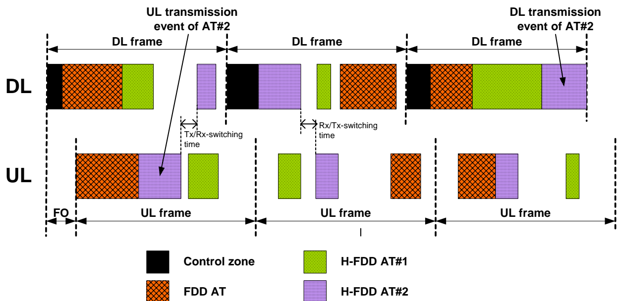
Figure 20: H-FDD operation
