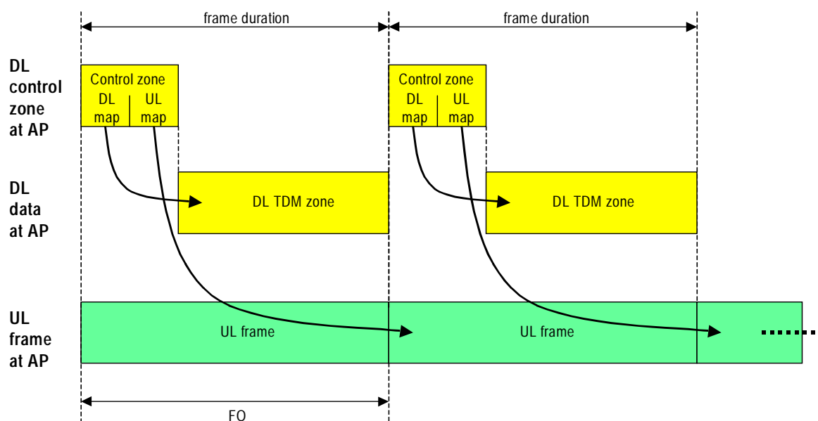
Figure 34: Maximum time relevance for UL map (FDD mode)
