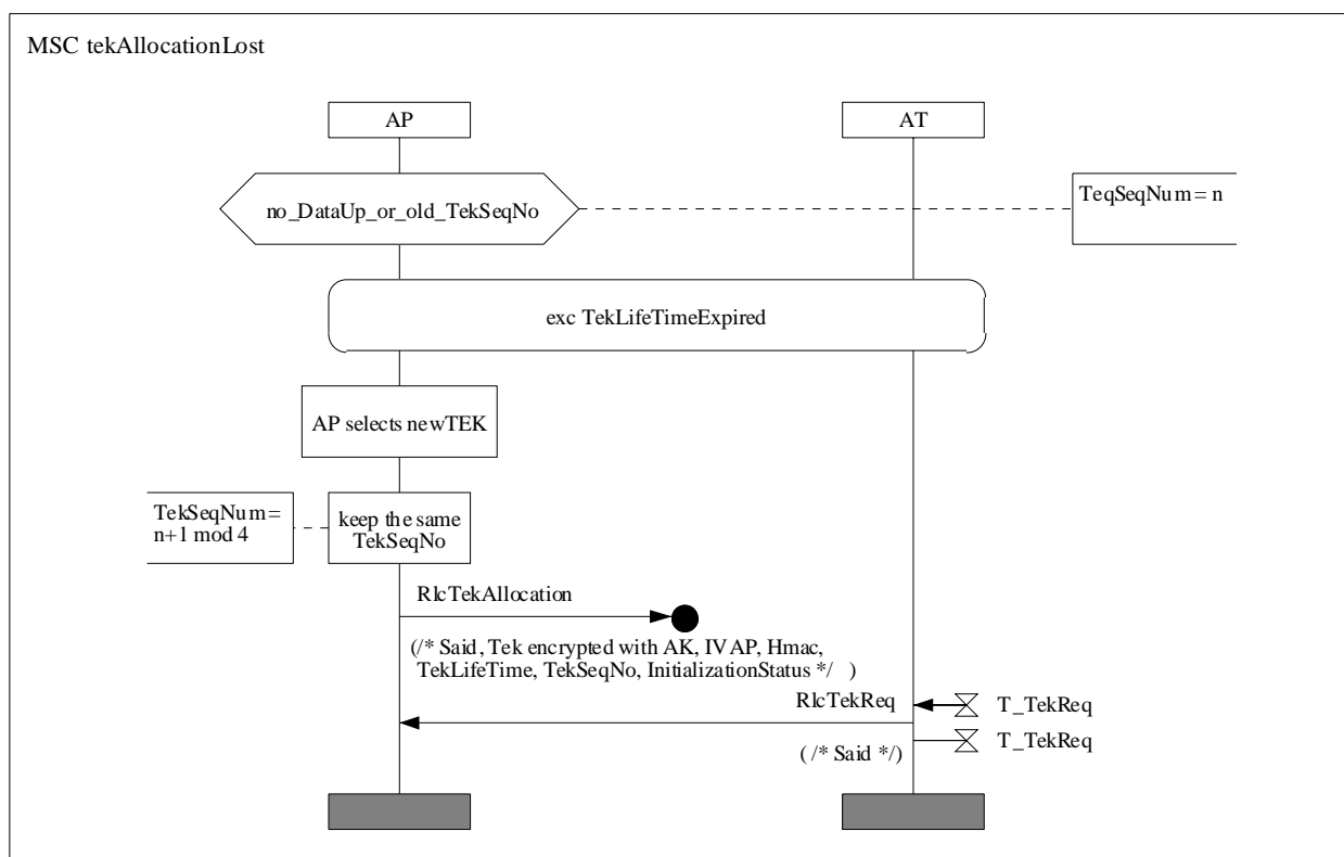
Diagram 28: MSC for retransmission in case of RlcTekAllocation loss during key renewal
