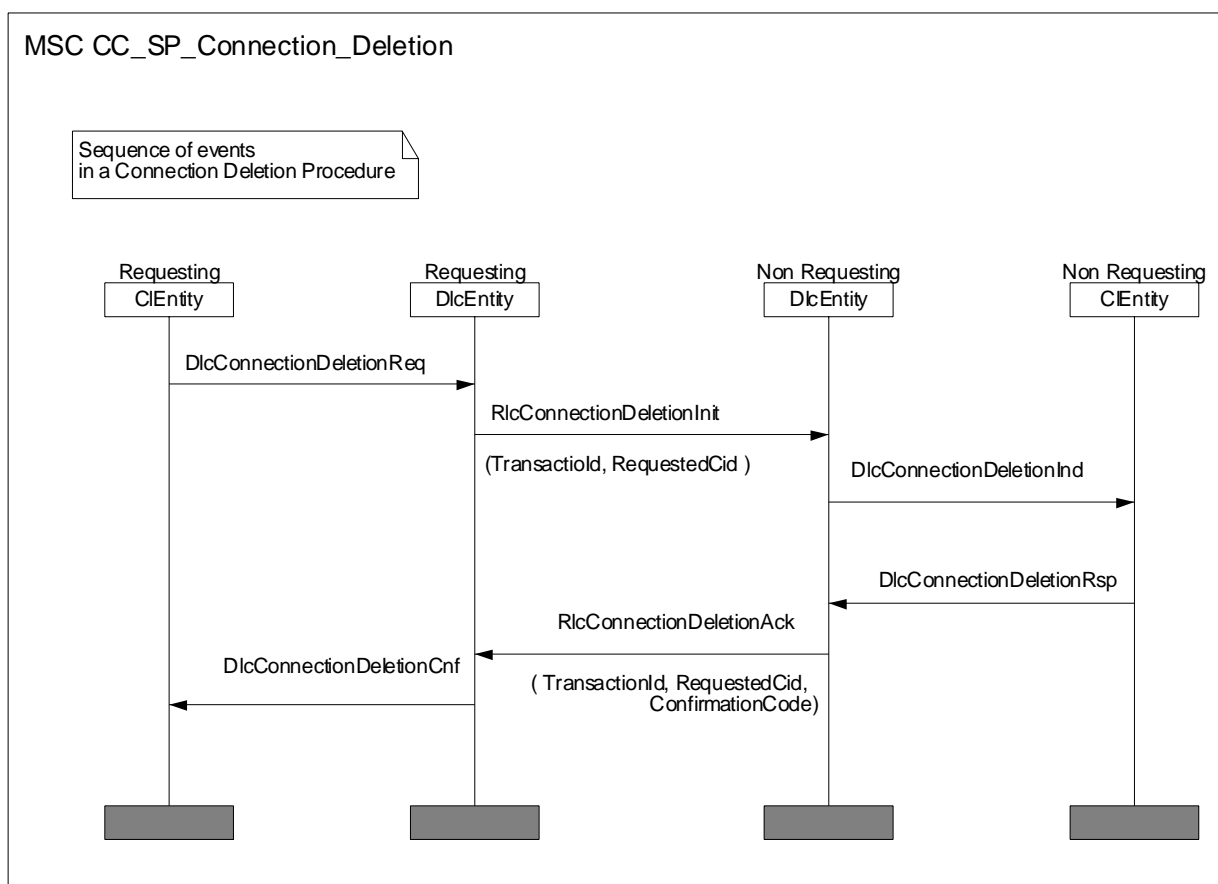
Diagram 34: MSC (4 entities) for AP/AT initiated connection release
