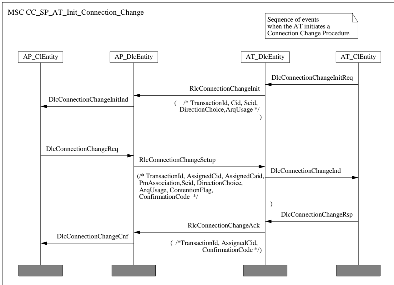
Diagram 32: MSC (4 entities) for AT initiated connection change
