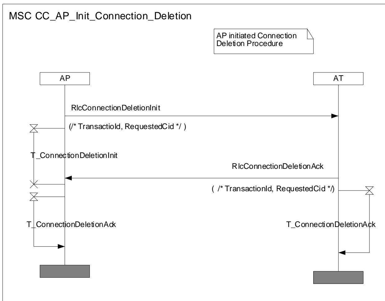
Diagram 41: MSC for AP initiated connection release
