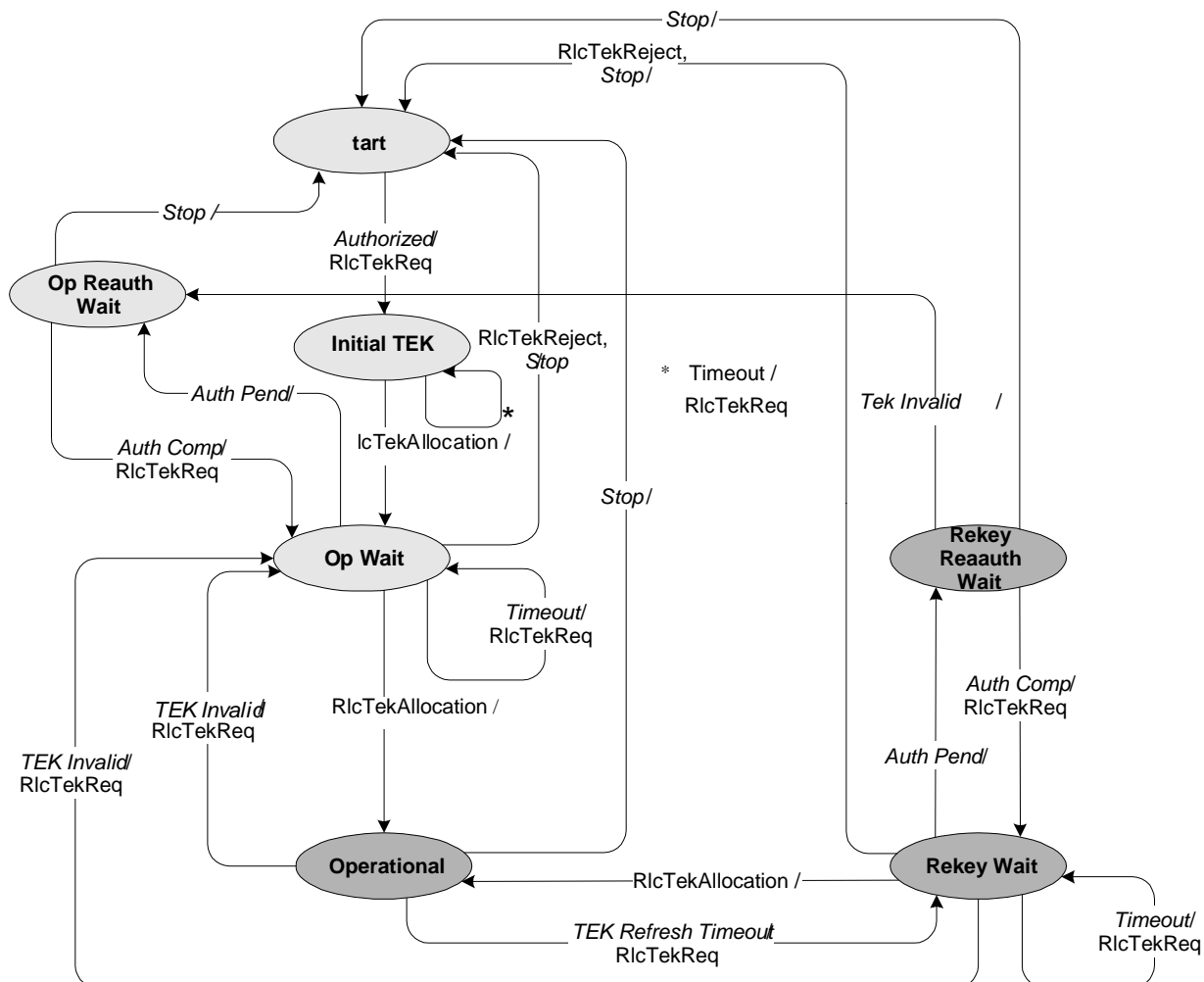
Figure 52: TEK Finite State Machine Flow Diagram
