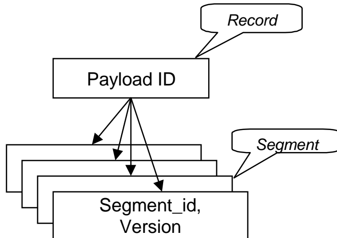
Figure 6: Relationship between records, payload IDs and segments
