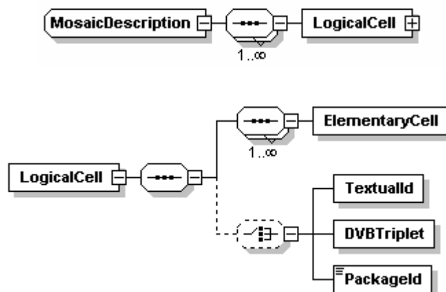
Figure C.4: MosaicDescription
