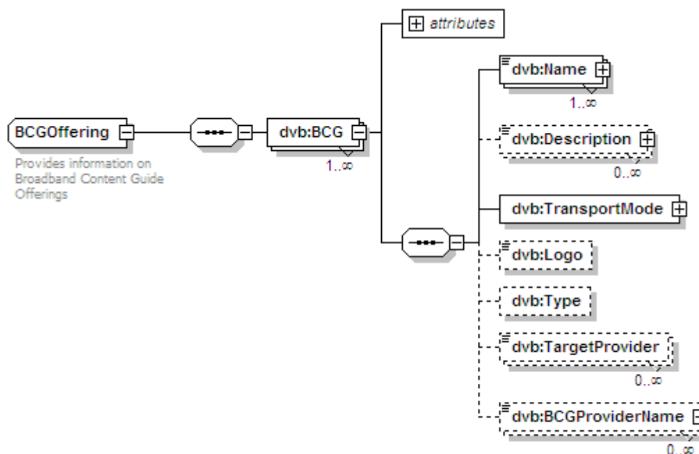
Figure C.16: BCGOffering
