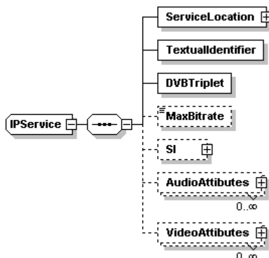
Figure C.2: IPService
