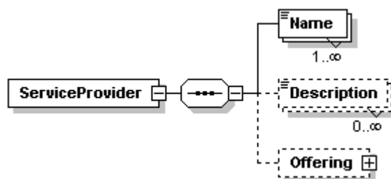
Figure C.15: Service Provider
