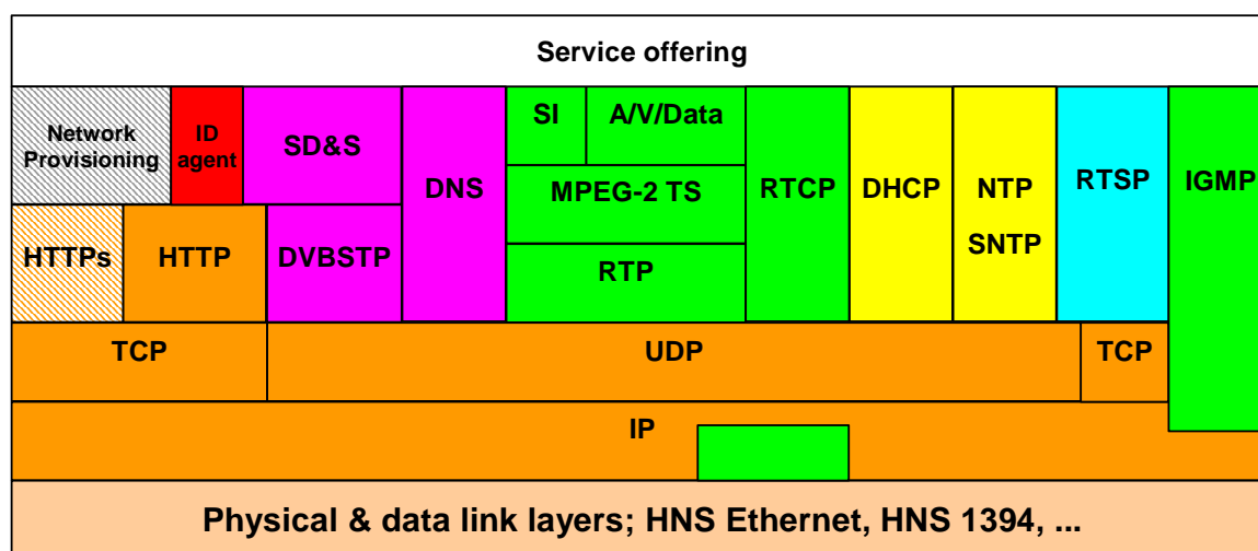
Figure 3: Diagram of the protocol stack for DVB-IP services
