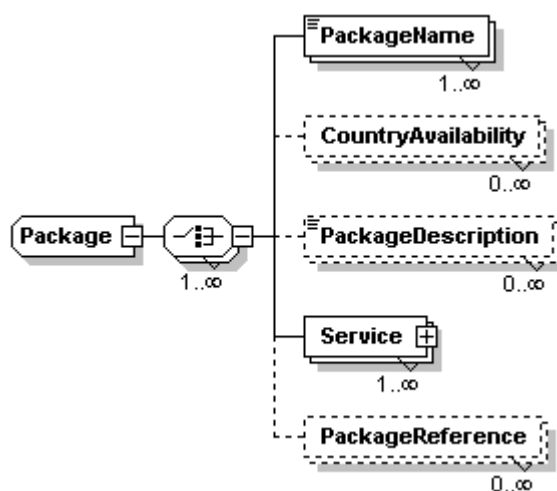
Figure C.10: Package
