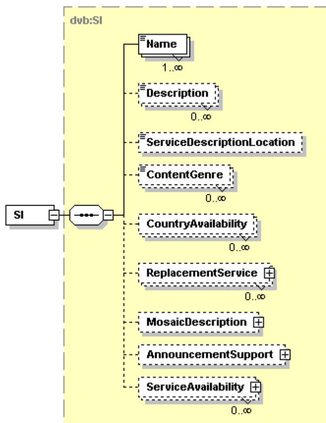
Figure C.9: SI
