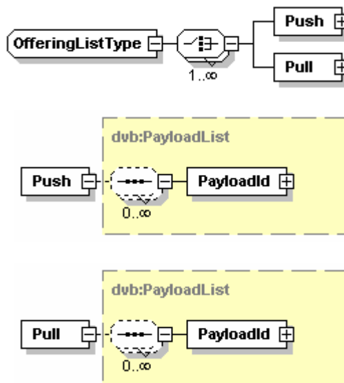
Figure C.5: OfferingListType
