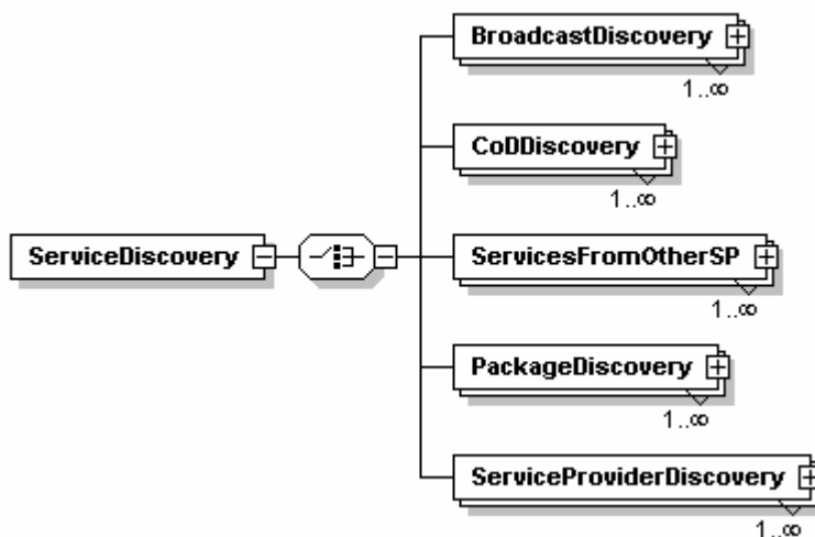
Figure C.17: Service discovery
