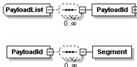
Figure C.6: PayloadList
