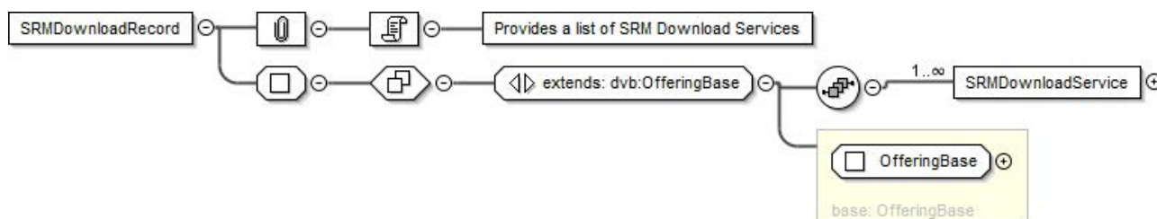
Figure 7cl: SRMDownloadRecord
