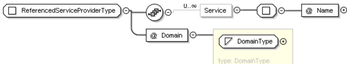
Figure 7bc: ReferencedServiceProviderType
