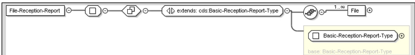
Figure C.18: File-Reception-Report
