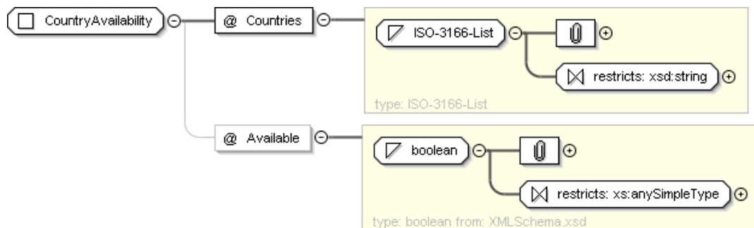
Figure 7aj: CountryAvailability
