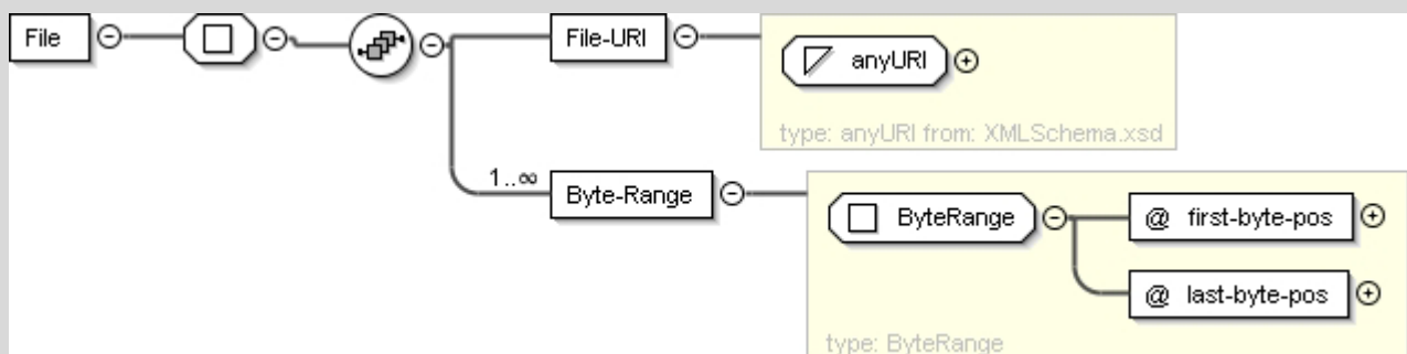
Figure C.21: File
