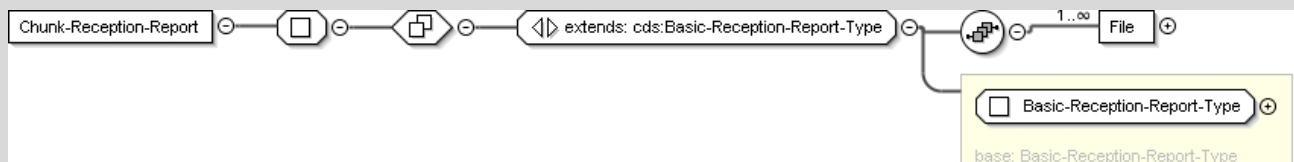
Figure C.20: Chunk-Reception-Report
