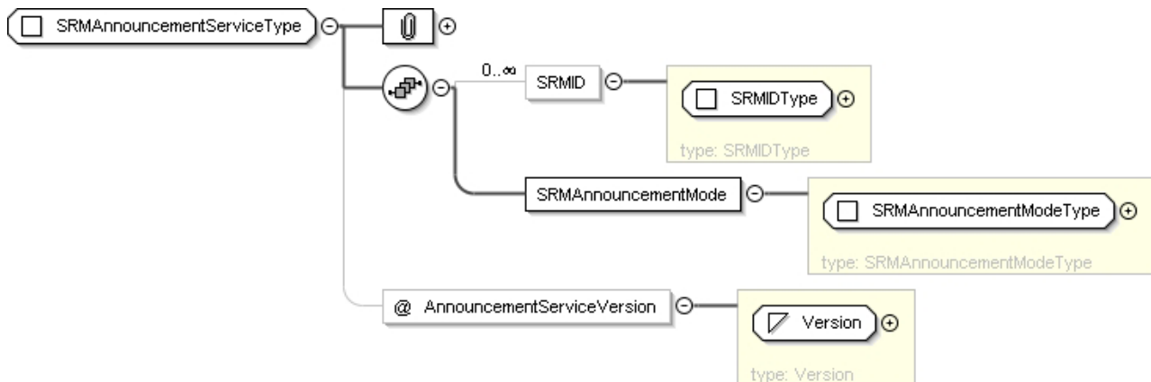
Figure 7bp: SRMAnnouncementServiceType
