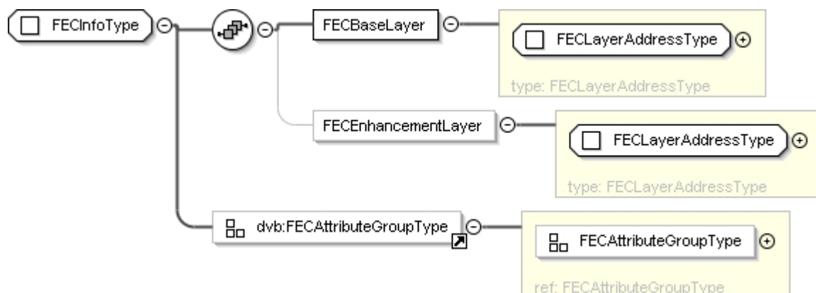
Figure 7an: FECInfoType Type
