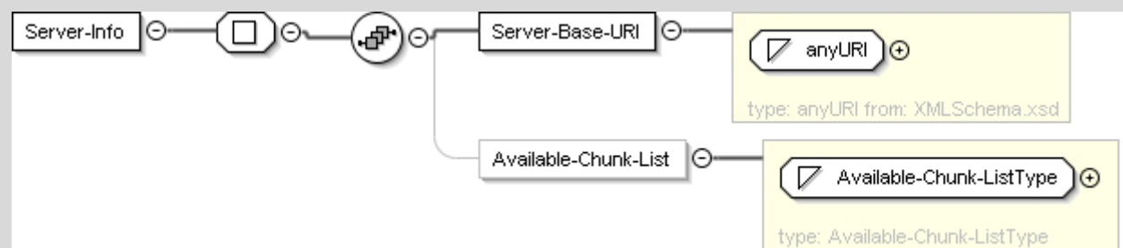
Figure C.14: Server-Info
