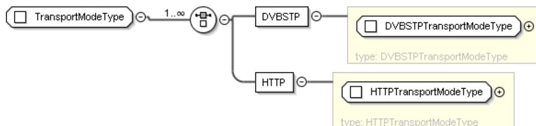
Figure 7by: TransportModeType
