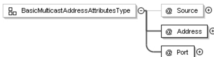
Figure 7ab: BasicMulticastAddressAttributesType
