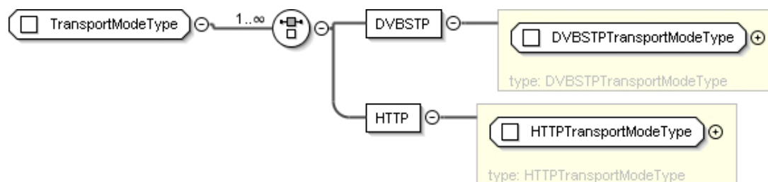
Figure 7by: TransportModeType
