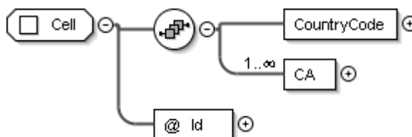
Figure 7ah: Cell
