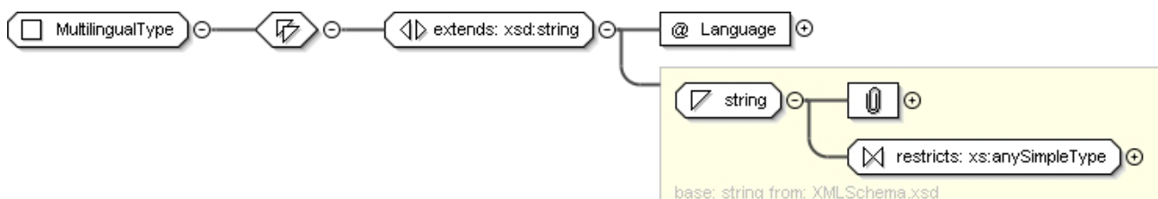
Figure 7av: MultilingualType
