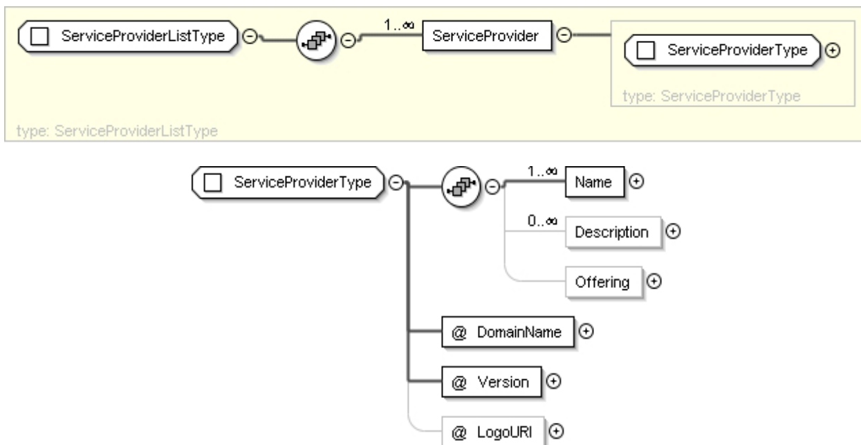
Figure 7ch: ServiceProviderDiscoveryType
