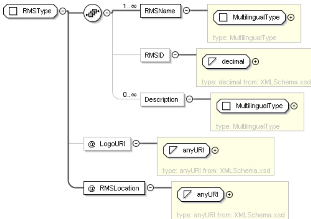
Figure 7bg: RMSType
