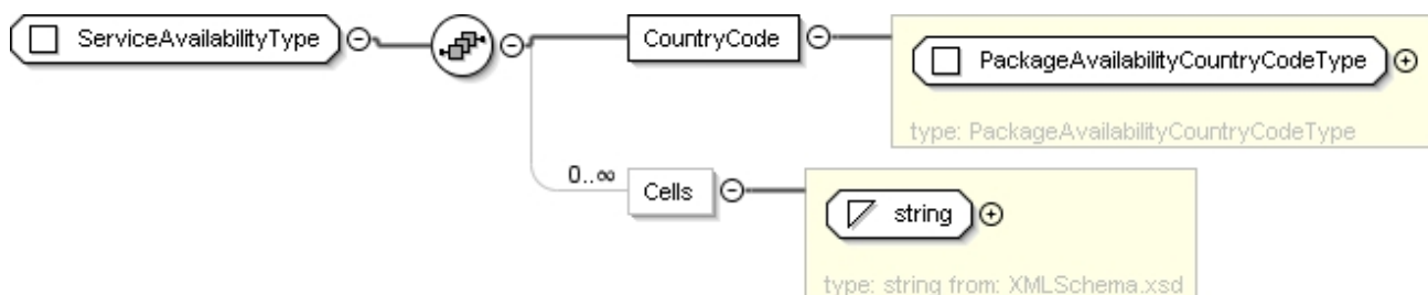
Figure 7bk: ServiceAvailabilityType
