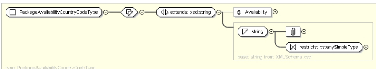
Figure 7ay: PackageAvailabilityCountryCodeType
