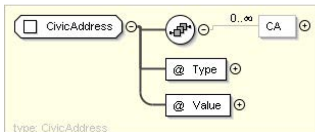
Figure 7ai: CivicAddress
