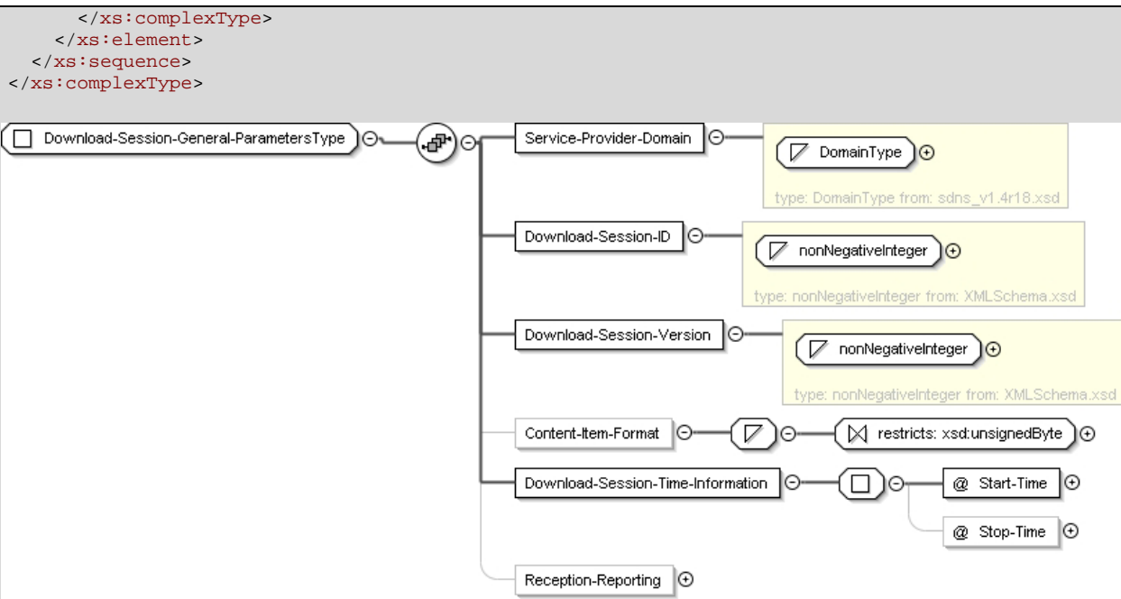
Figure C.1: Download-Session-General-ParametersType
