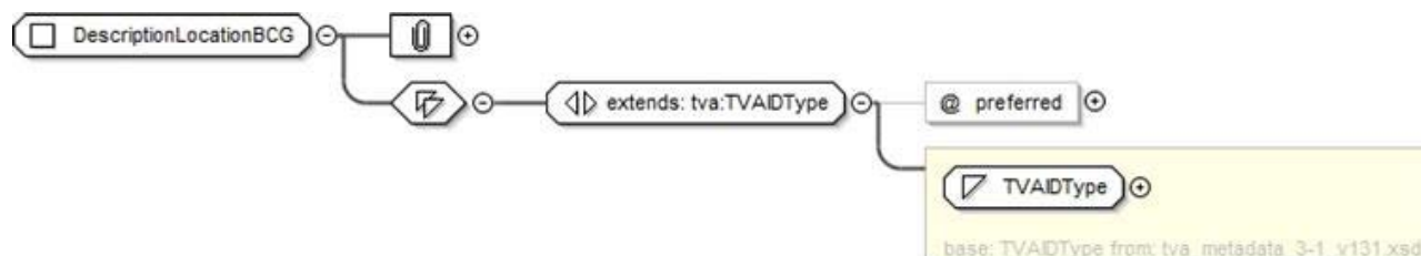
Figure 7ak: DescriptionLocationBCG
