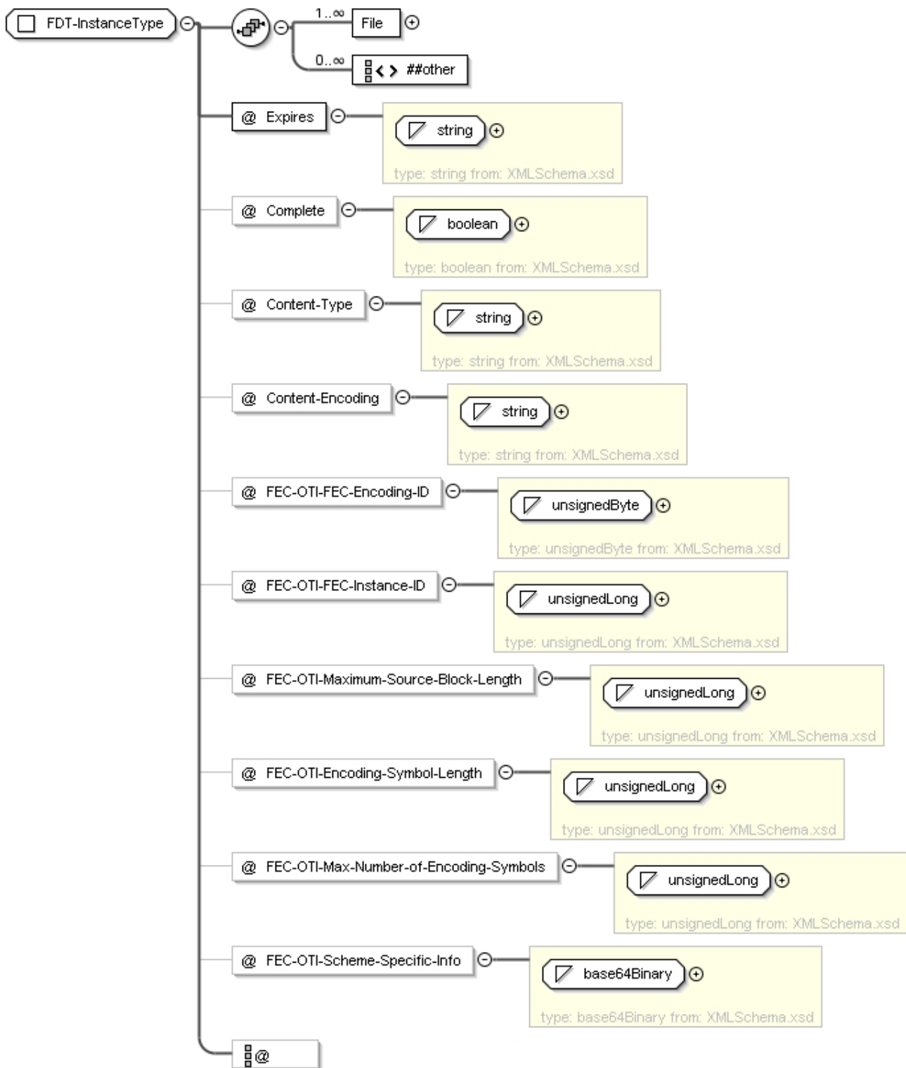
Figure C.24: FDT-InstanceType
