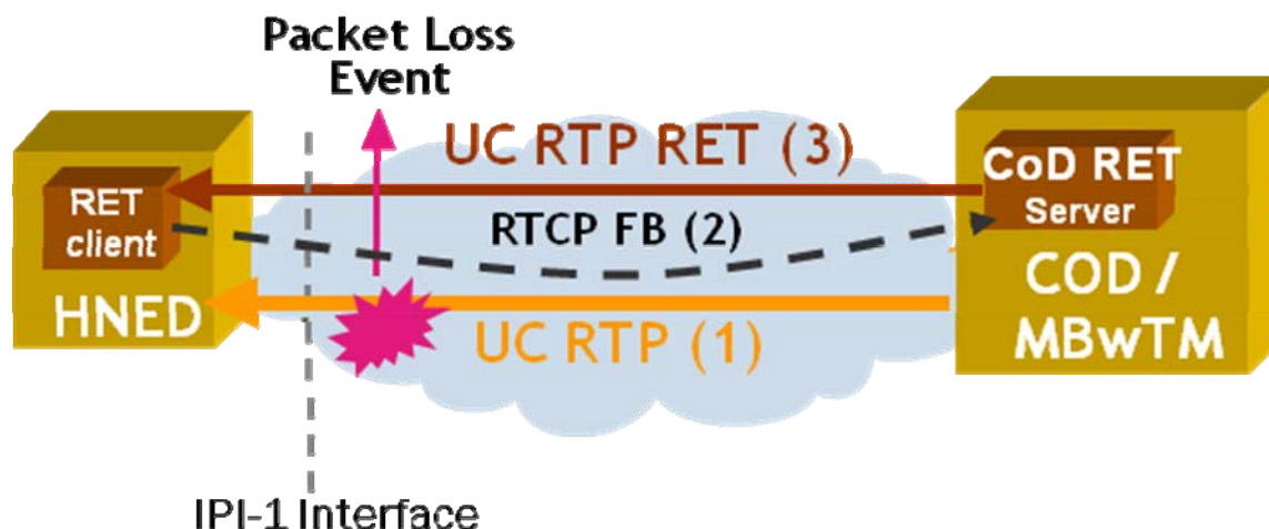
Figure F.1: RET Architecture and messaging for CoD/MBwTM services overview
