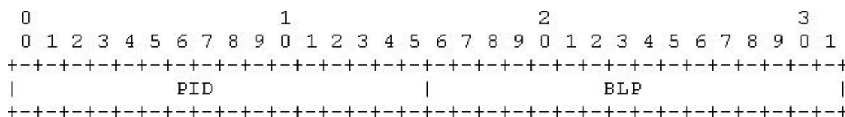
Figure F.5: Format of the Generic NACK put in the FCI field in the RTCP FB message
