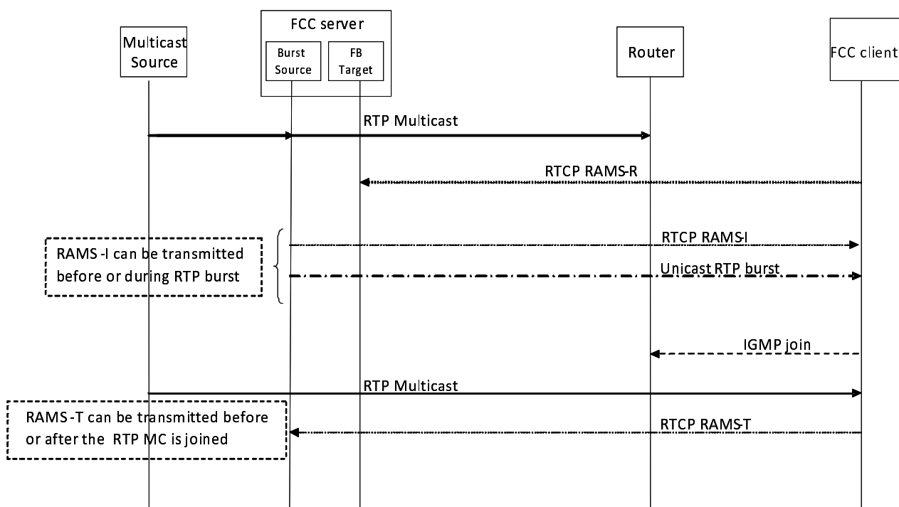
Figure I.2: Basic RAMS messaging between DVB FCC(/RET) client and DVB FCC (/LMB RET) server
