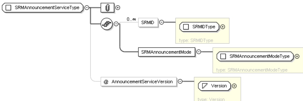
Figure 7bp: SRMAnnouncementServiceType
