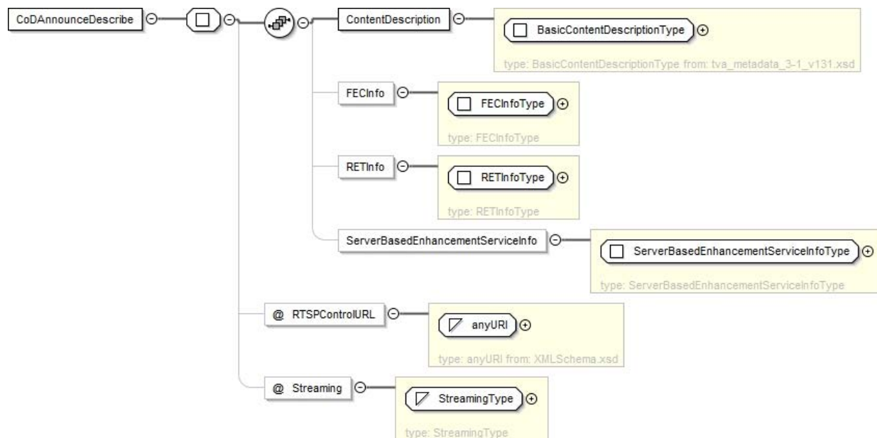
Figure 7ck: CoDAnnounceDescribe
