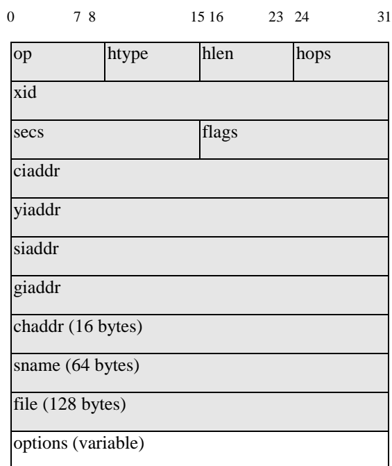
Figure 14: DHCP Format
