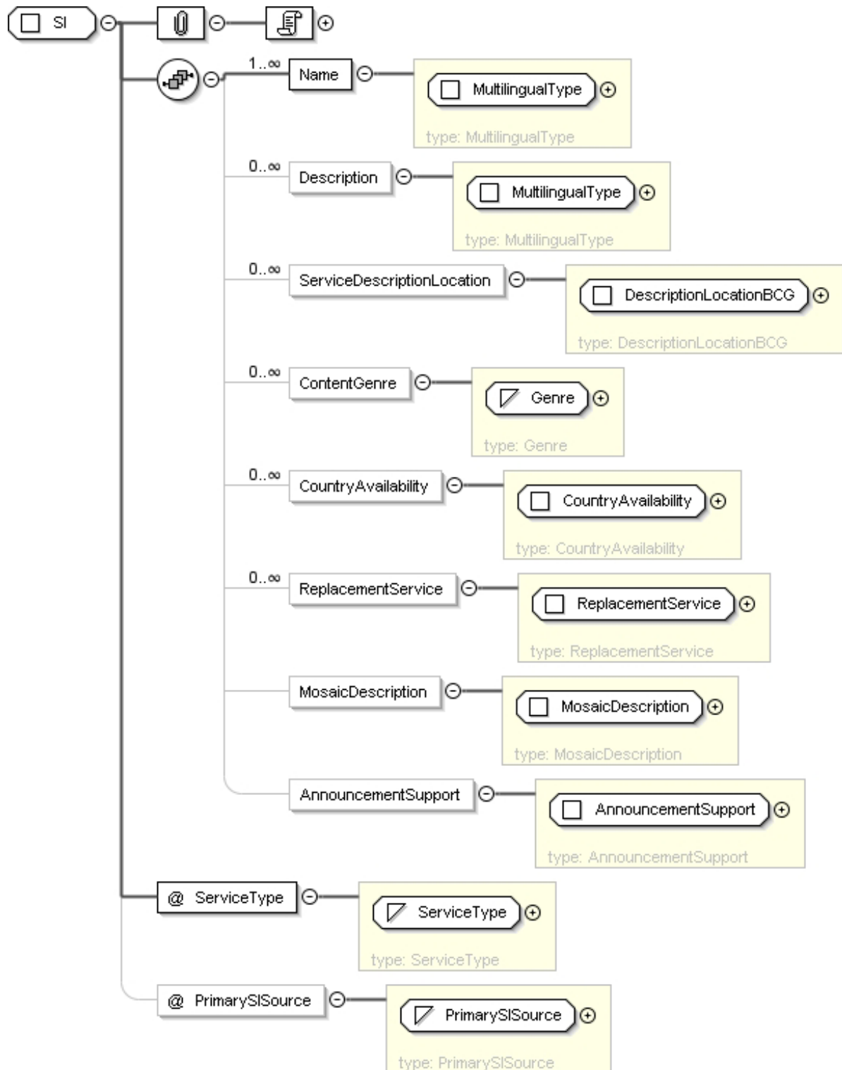
Figure 7bm: SI
