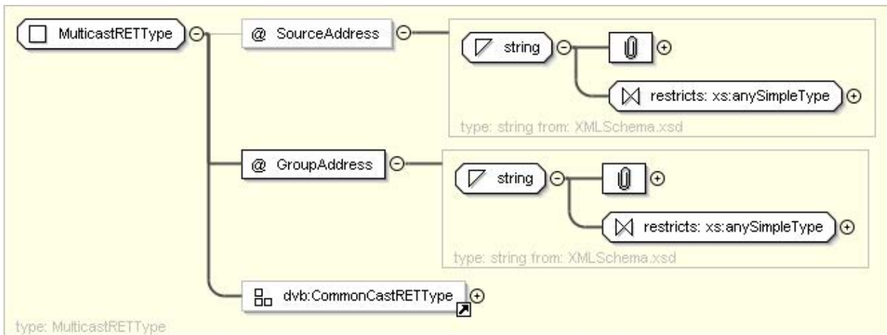
Figure 7au: MulticastREType
