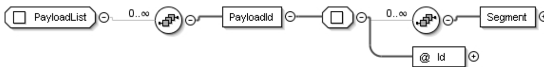
Figure 7ba: PayloadList
