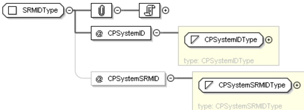
Figure 7bt: SRMIDType
