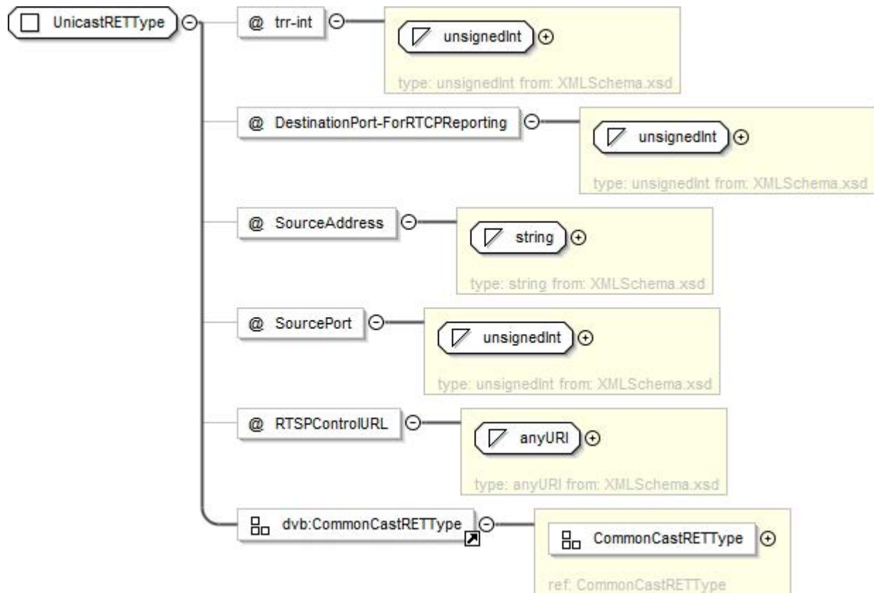
Figure 7bz: UnicastRETType
