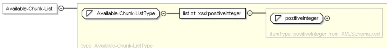
Figure C.15: Available-Chunk-List
