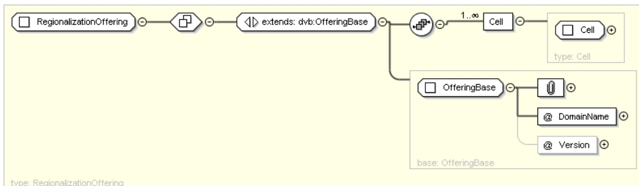
Figure 7ci: Regionalization Offering
