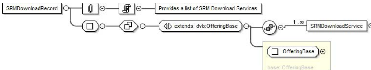
Figure 7cl: SRMDownloadRecord
