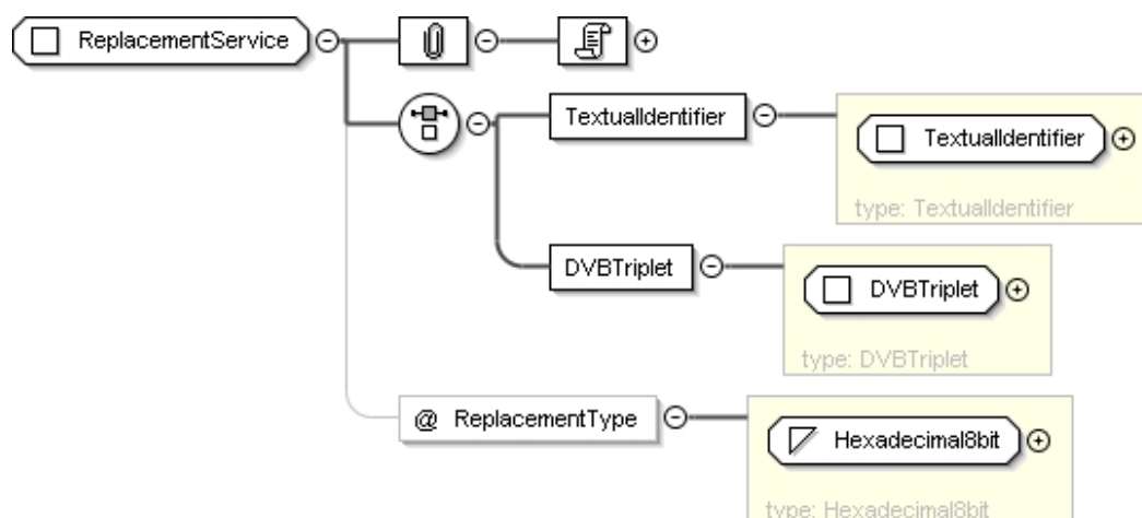
Figure 7bd: ReplacementService
