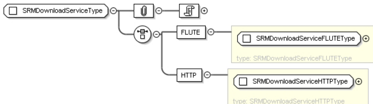
Figure 7bs: SRMDownloadServiceType
