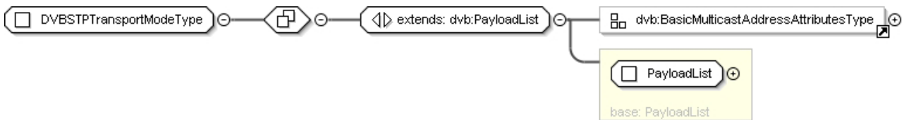
Figure 7a: DVBSTPTransportModeType
