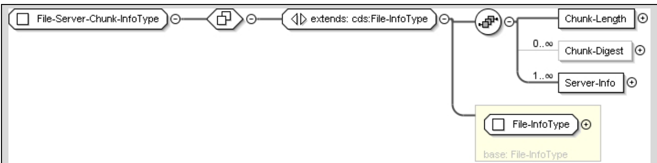
Figure C.12: File-Server-Chunk-InfoType
