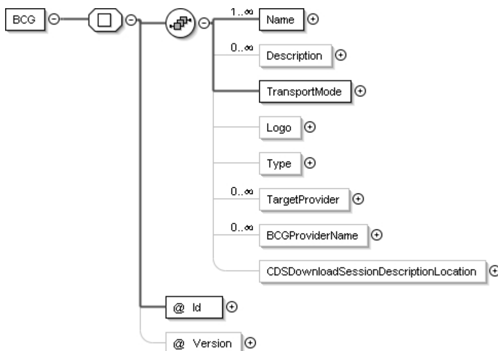
Figure 7cb: BCGOffering
