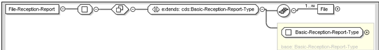
Figure C.18: File-Reception-Report
