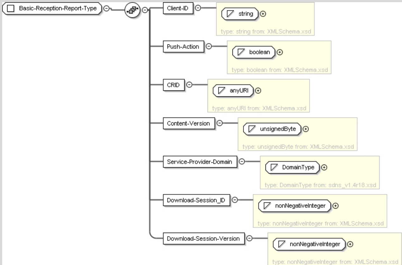
Figure C.22: Basic-Reception-ReportType
