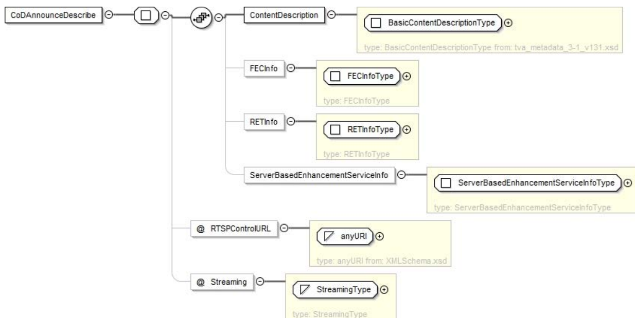
Figure 9b: RTSPAnnounceDescribe
