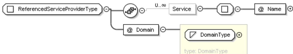
Figure 7bc: ReferencedServiceProviderType
