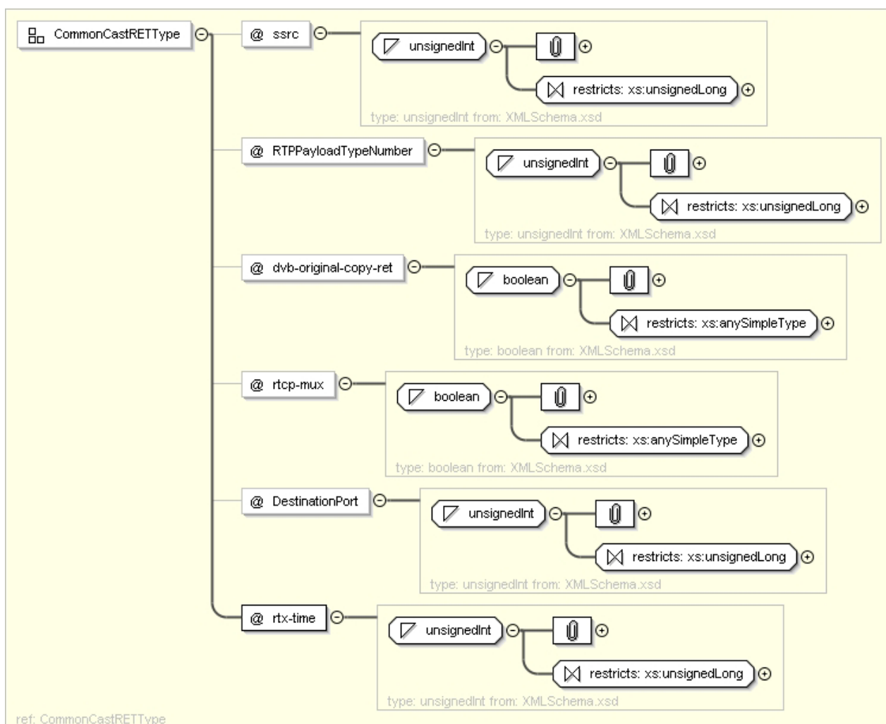
Figure 7ac: CommonCastRETRType
