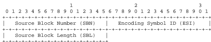
Figure E.6: Repair FEC Payload ID
