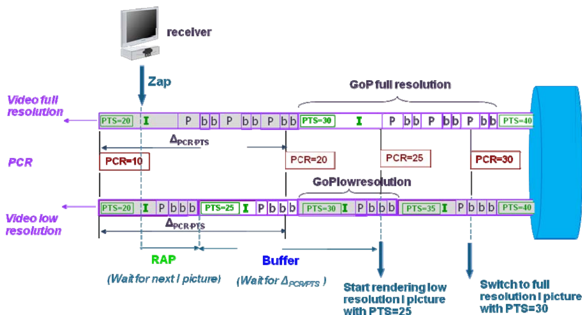
Figure J.3: Companion Stream FCC process: RAP delay-only improvement
