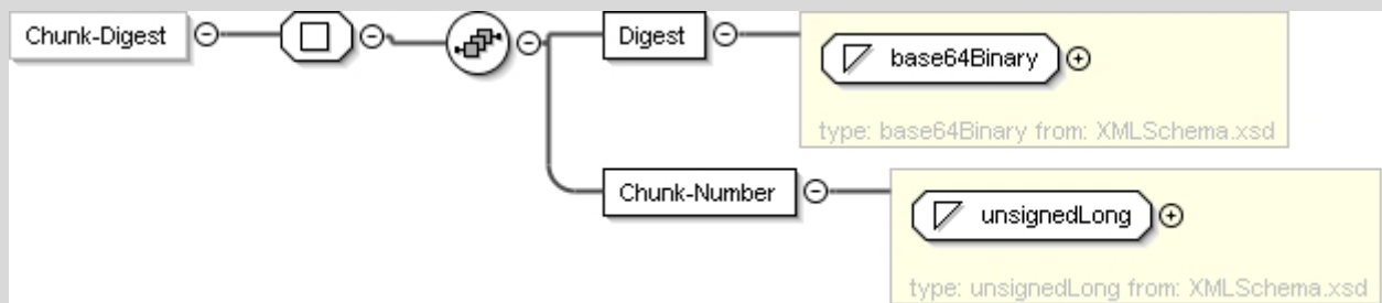
Figure C.13: Chunk-Digest
