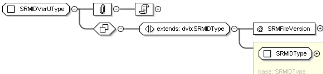
Figure 7bv: SRMIDVerUType
