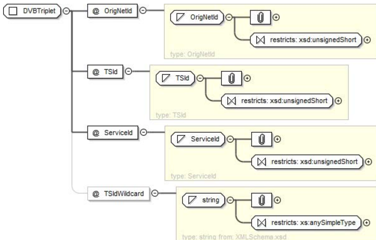
Figure 7a: DVBTripлет
