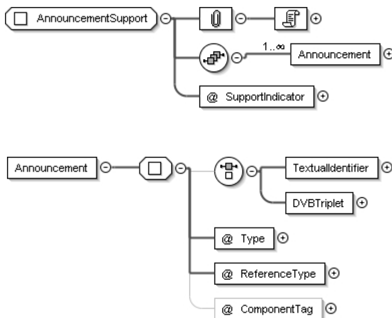
Figure 7af: AnnouncementSupport
