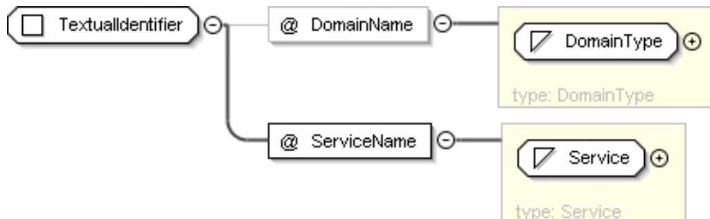
Figure 7bx: TextualIdentifier
