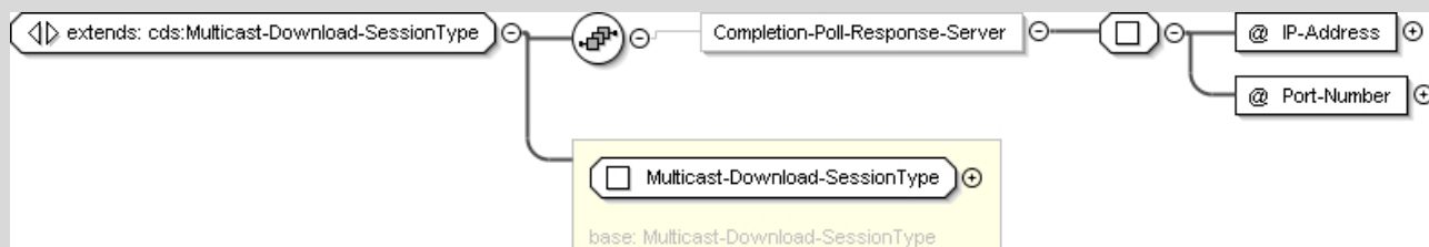
Figure C.7: Extended Multicast-Download-SessionType
