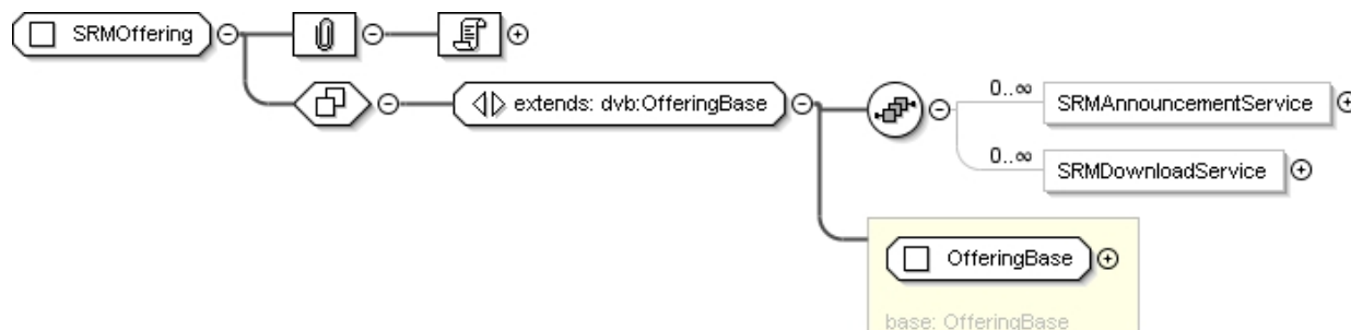
Figure 7cj: SRMOffering
