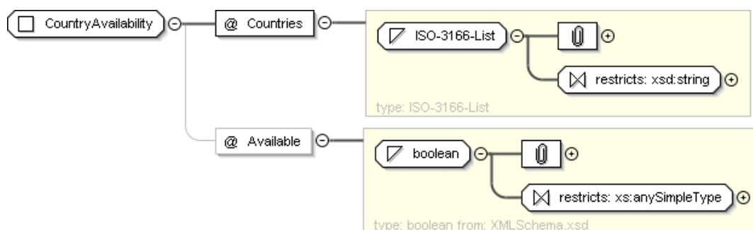
Figure 7aj: CountryAvailability
