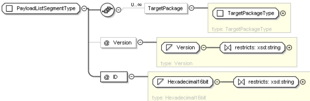
Figure 7bb: PayloadListSegmentType
