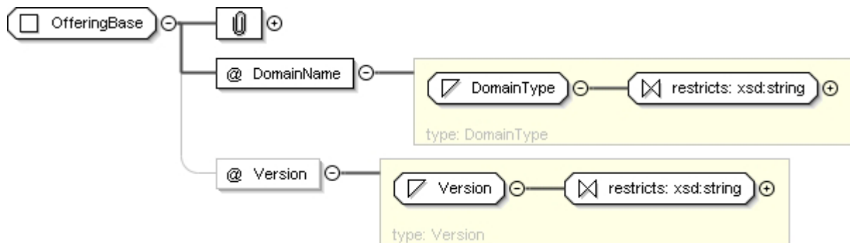
Figure 7aw: OfferingBase
