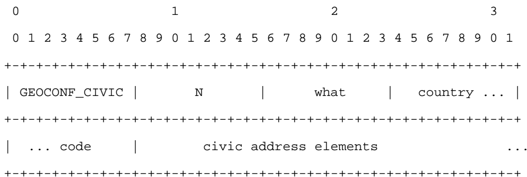
Figure 15: GEOCONF_CIVIC Format
