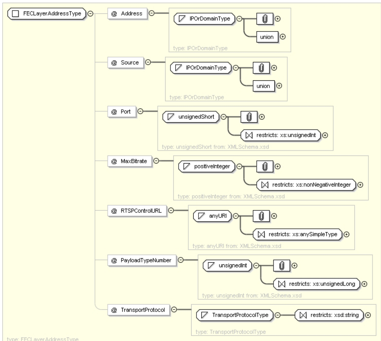
Figure 7a0: FECLayerAddressType
