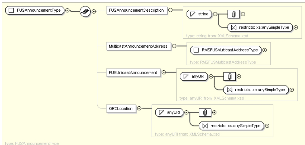
Figure 7ap: FUSAnnouncementType
