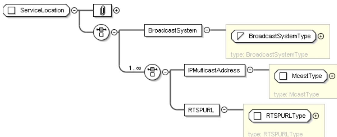
Figure 7bl: ServiceLocation
