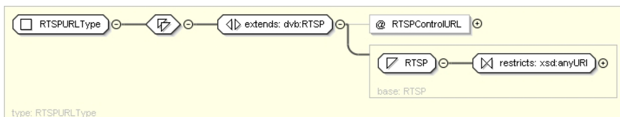
Figure 7bi: RTSPURLType
