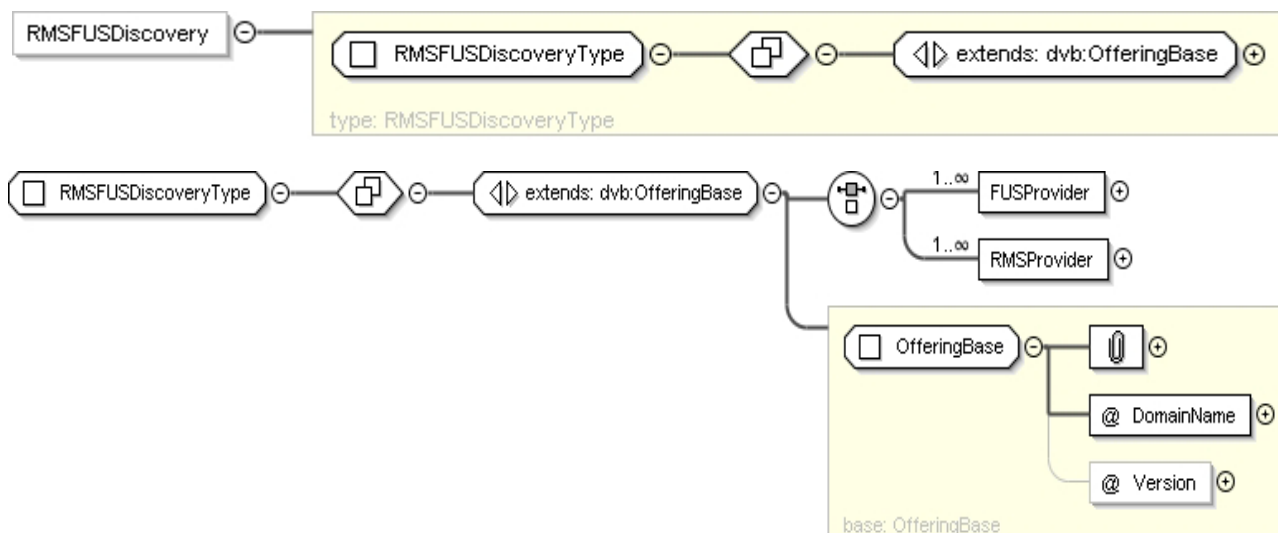
Figure 7cg: RMSFUSDiscoveryType
