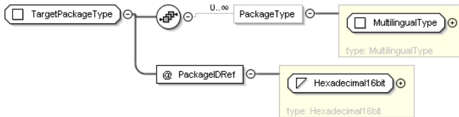
Figure 7bw: TargetPackageType
