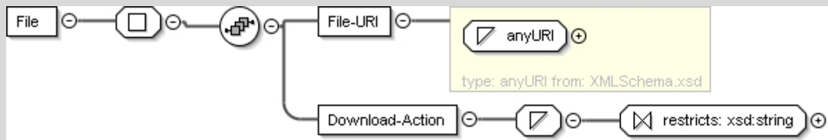
Figure C.17: File
