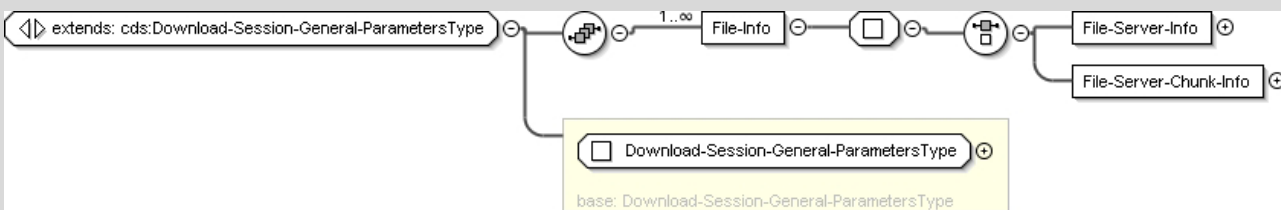
Figure C.4: Extended Download-Session-General-ParametersType
