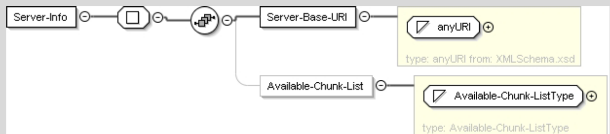
Figure C.14: Server-Info
