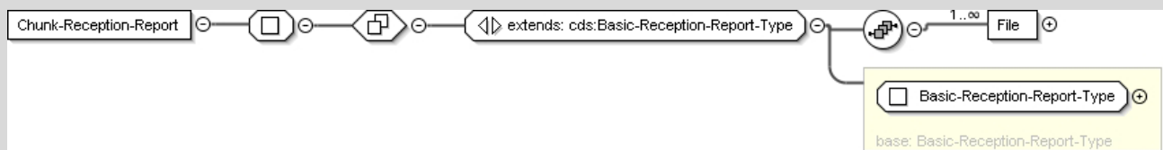
Figure C.20: Chunk-Reception-Report
