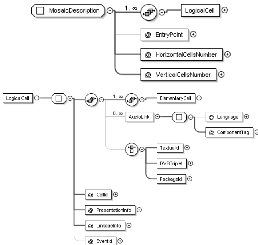
Figure 7at: MosaicDescription
