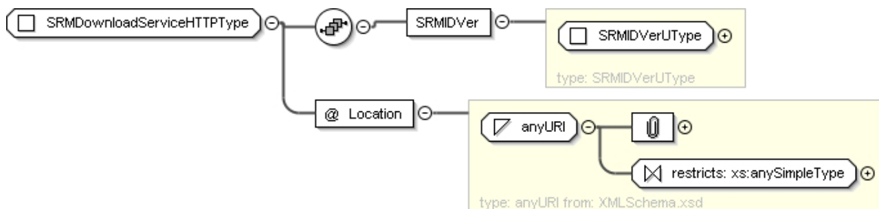
Figure 7br: SRMDownloadServiceHTTPType
