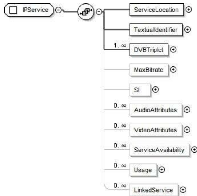
Figure 7cc: IPService (Informative)
