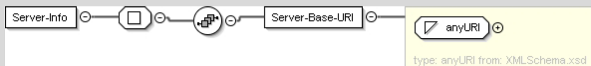
Figure C.11: Server-Info
