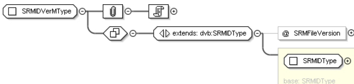
Figure 7bu: SRMIDVerMType
