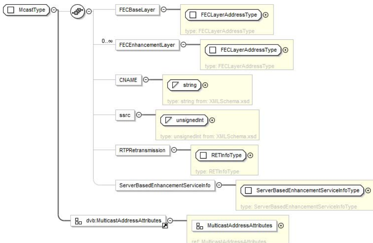
Figure 7as: McastType
