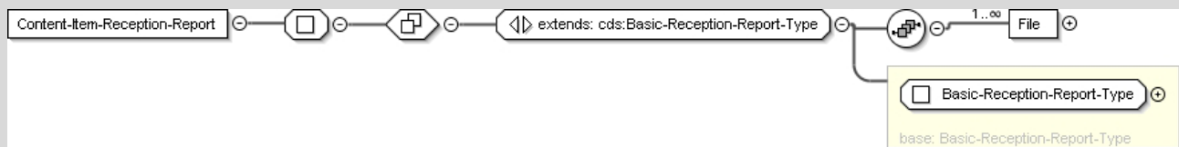
Figure C.16: Content-Item-Reception-Report
