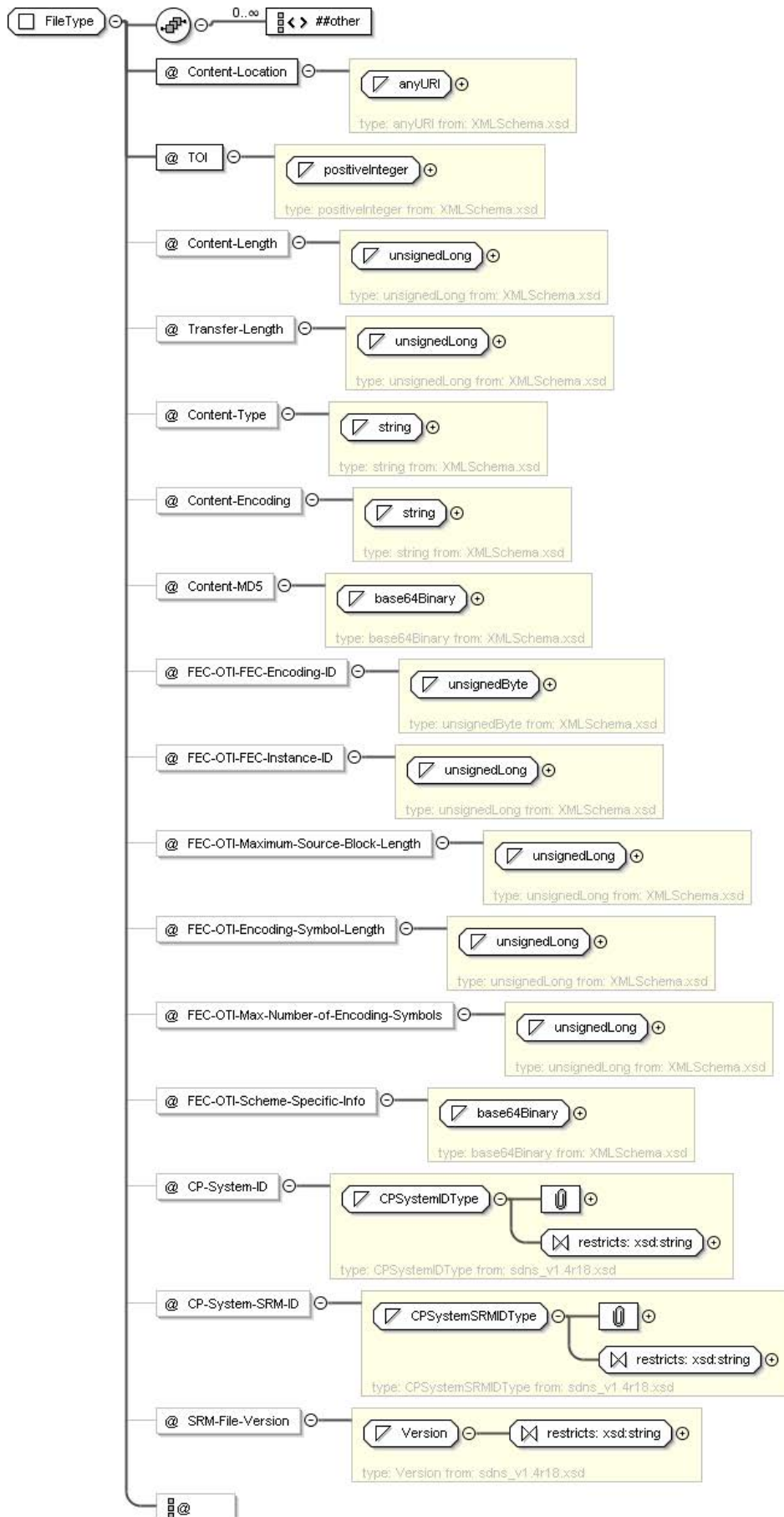
Figure C.25: FileType
