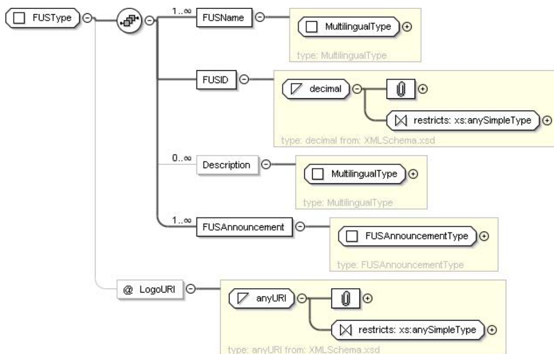
Figure 7aq: FUSType
