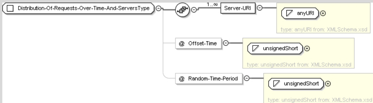
Figure C.8: Distribution-Of-Requests-Over-Time-And-ServersType
