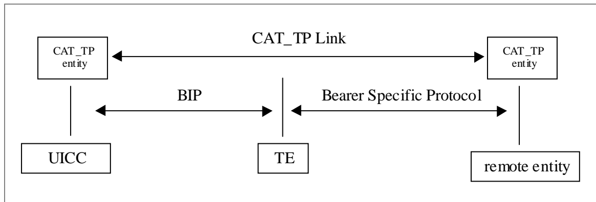
Figure 1: Environment description
