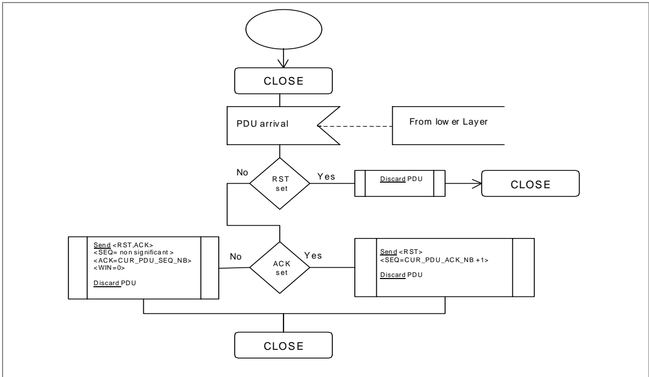
Figure 24: CLOSE state PDU arrival event processing
