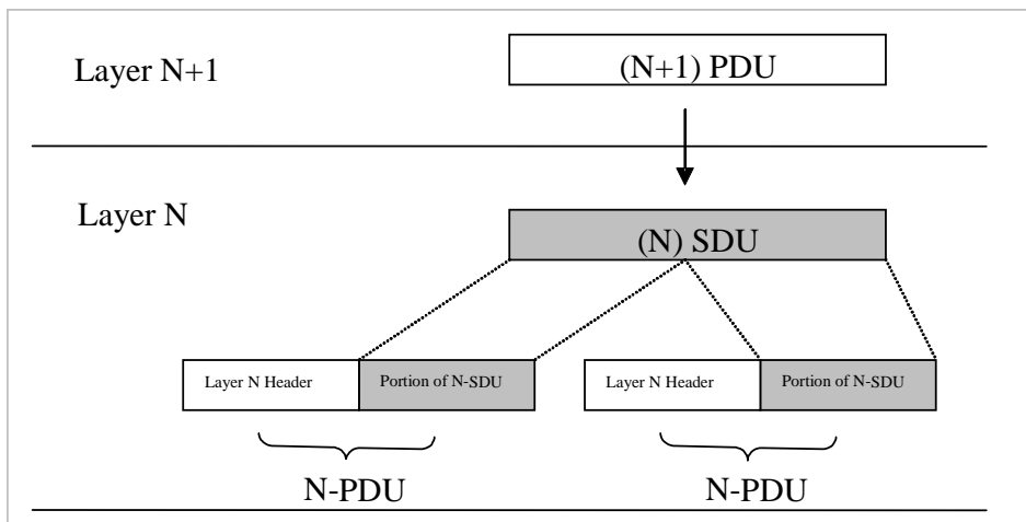
Figure 5: N-SDU and N-PDU with segmentation
