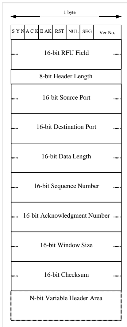
Figure 38: CAT_TP Header Format
