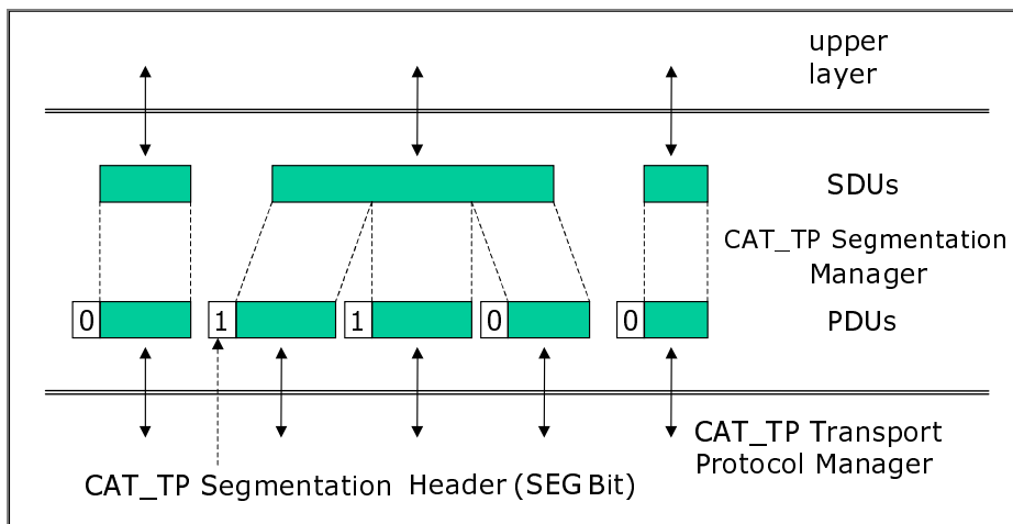
Figure 7: Segmentation description
