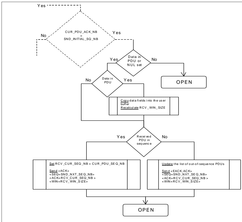
Figure 34: SYN-RCVD state PDU arrival event processing 4/4
