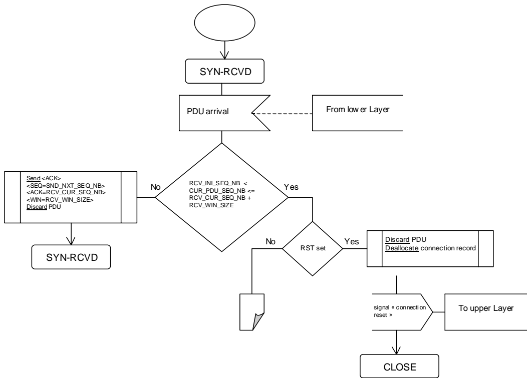
Figure 31: SYN-RCVD state PDU arrival event processing 1/4
