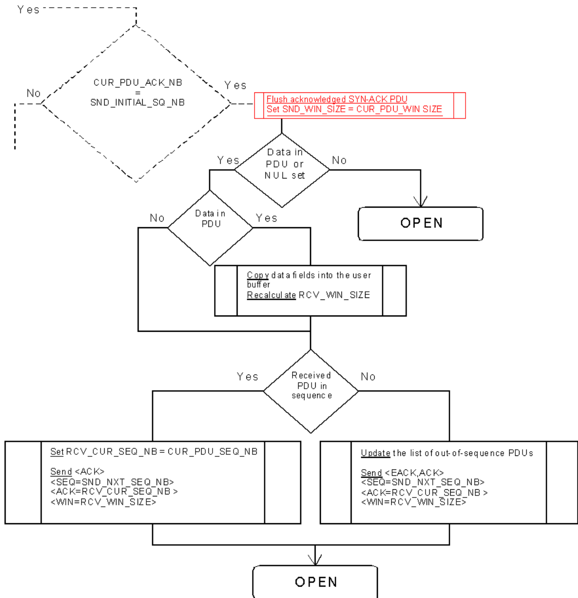
Figure 34: SYN-RCVD state PDU arrival event processing 4/4
