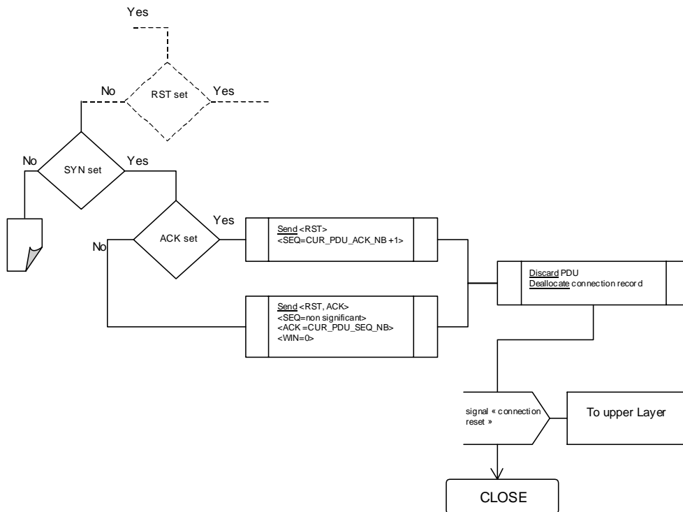
Figure 26: OPEN state PDU arrival event processing 2/4
