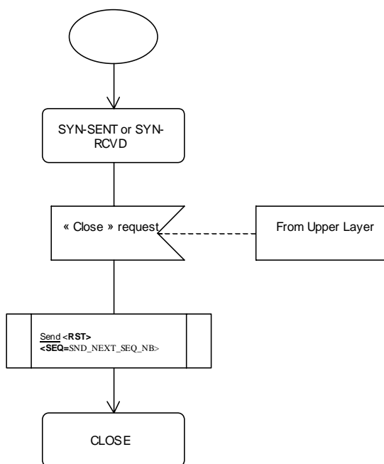
Figure 15: Close request in SYN-SENT or SYN-RCVD state
