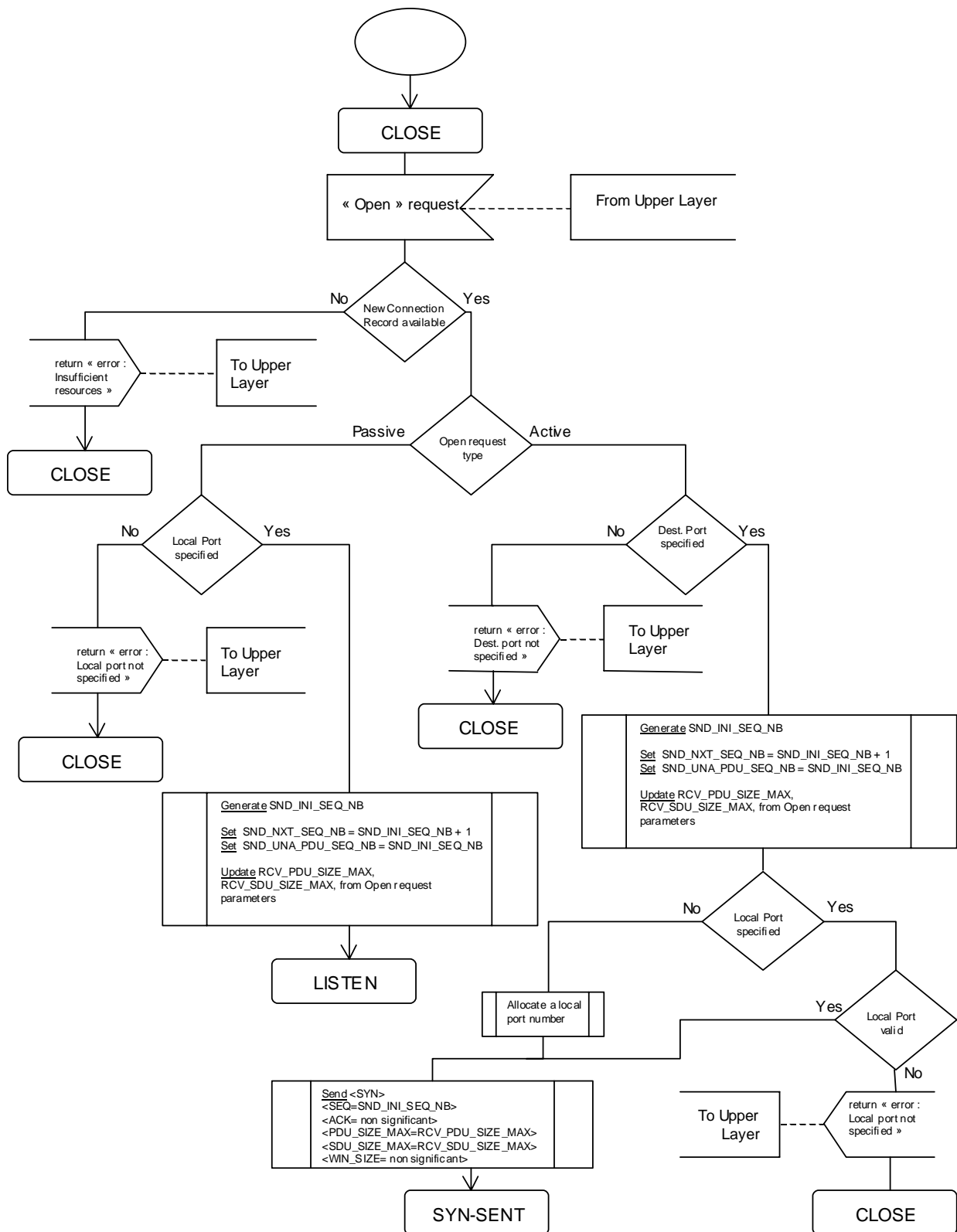
Figure 11: Open request in CLOSED state
