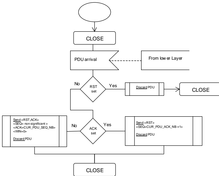
Figure 24: CLOSE state PDU arrival event processing
