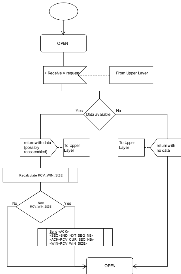
Figure 17: Receive request in OPEN state
