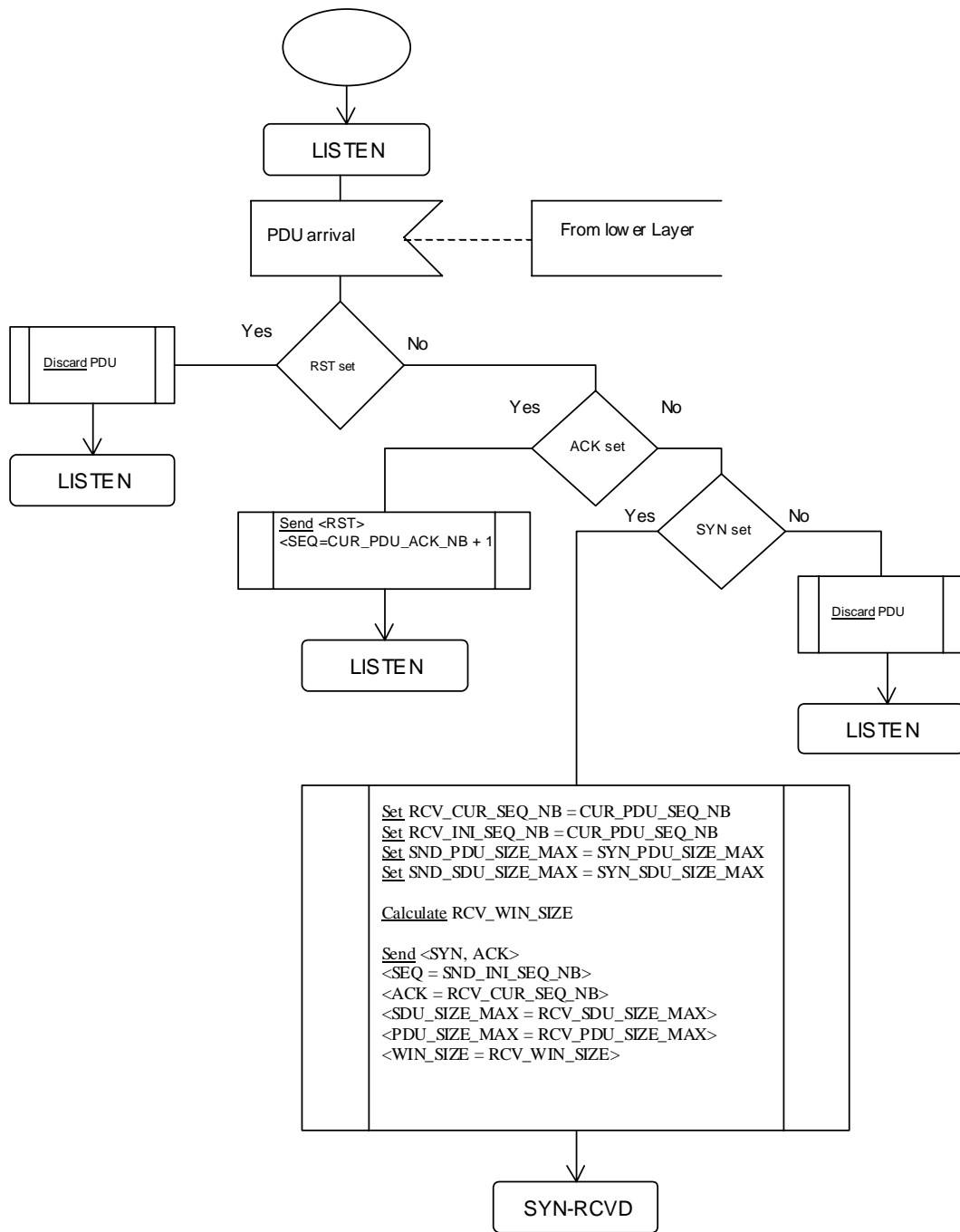
Figure 29: LISTEN state PDU arrival event processing
