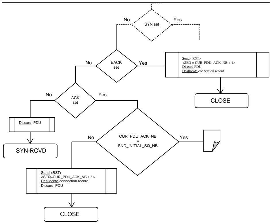
Figure 33: SYN-RCVD state PDU arrival event processing 3/4
