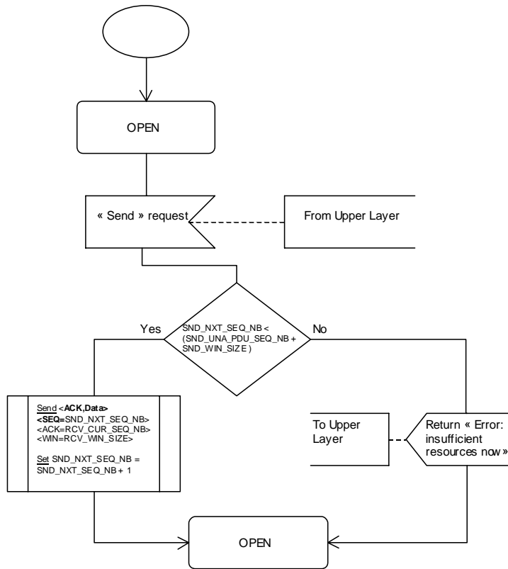
Figure 21: Send request in OPEN state
