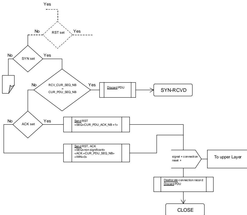
Figure 32: SYN-RCVD state PDU arrival event processing 2/4
