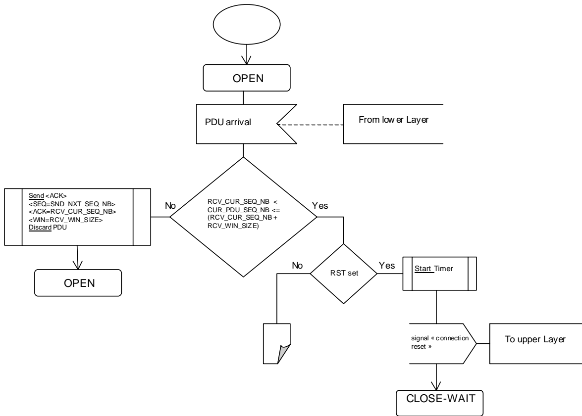
Figure 25: OPEN state PDU arrival event processing 1/4
