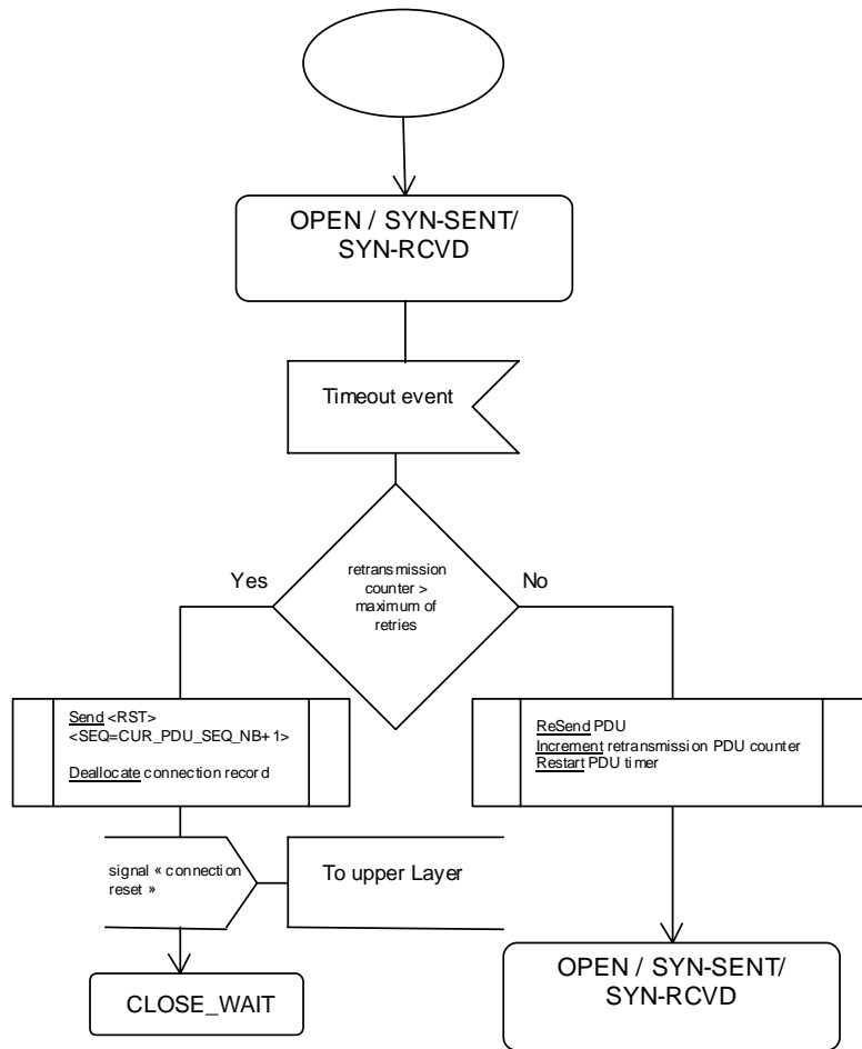
Figure 36: PDU retransmission timeout
