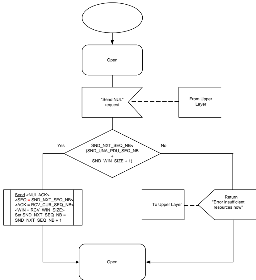
Figure 21a: Send NUL request in OPEN state
