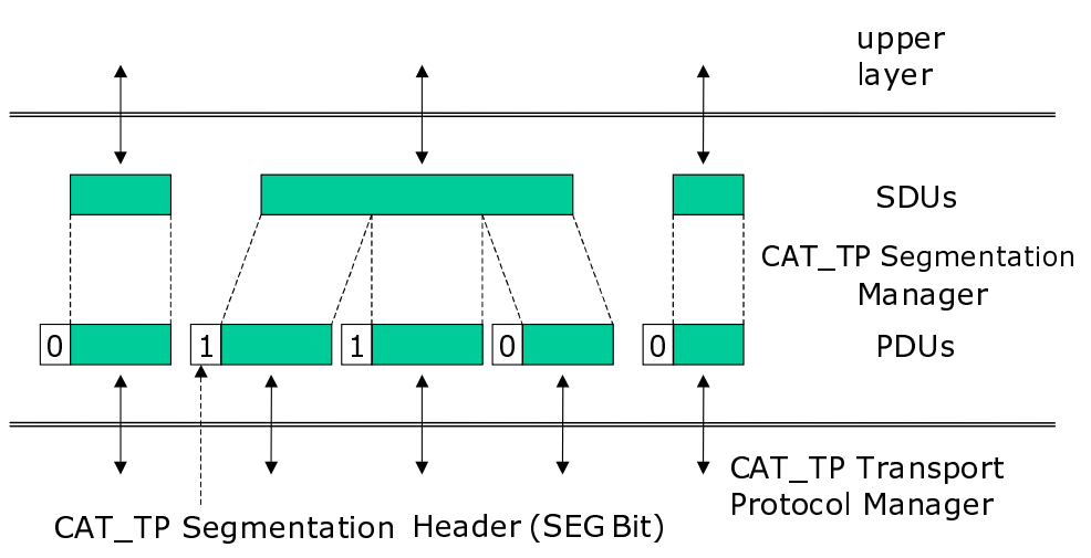
Figure 7: Segmentation description
