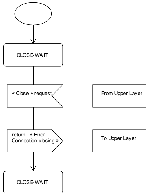
Figure 14: Close request in CLOSE-WAIT state
