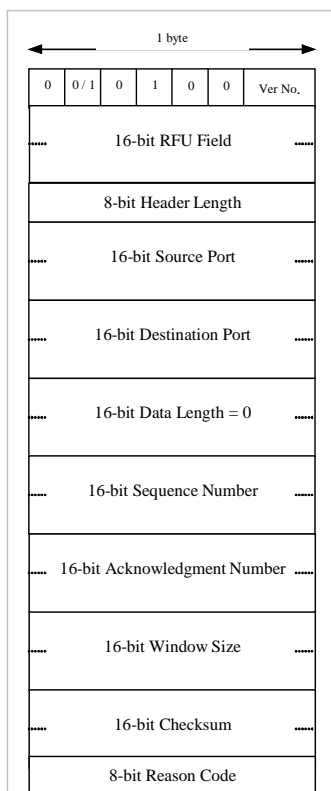
Figure 43: RST PDU structure
