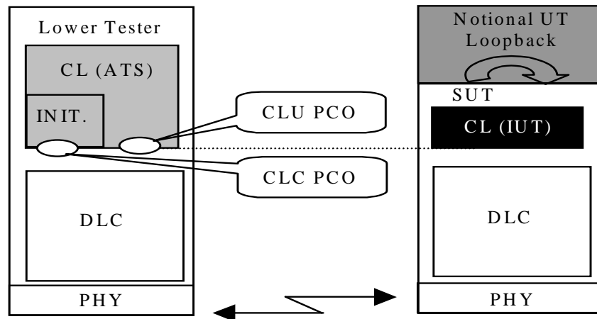
Figure 1: Test architecture for Cell CL - Common Part
