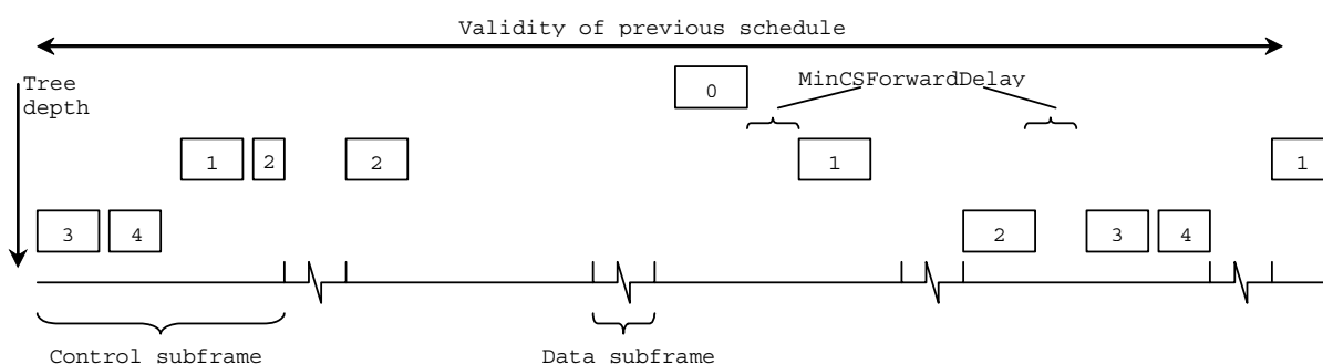
Figure 17: MSH-CSCH schedule validity
