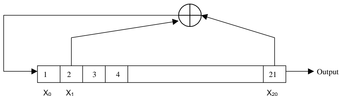
Figure 5.5.3.3: Beacon slot PN sequence
