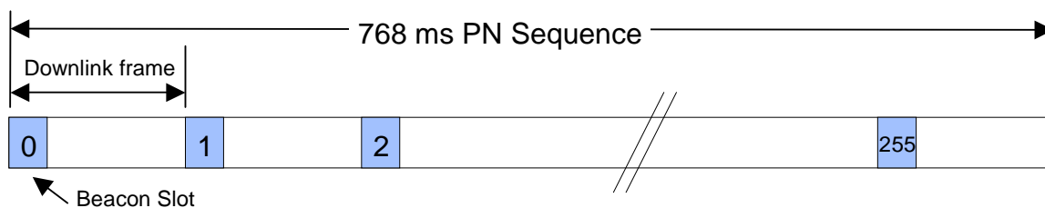
Figure 5.5.1: Superframe
