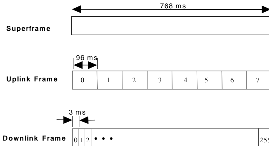
Figure 5.5.2.1: Frame relationships
