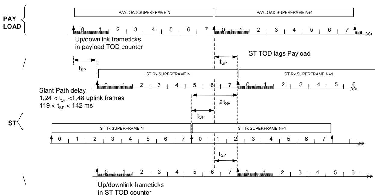
Figure 5.4.1: ToD reference
