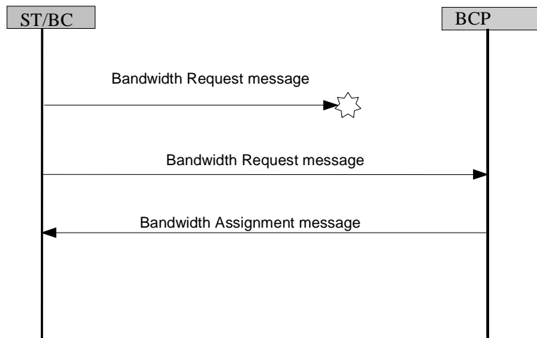
Figure B.4: Message corruption/lost during transmission
