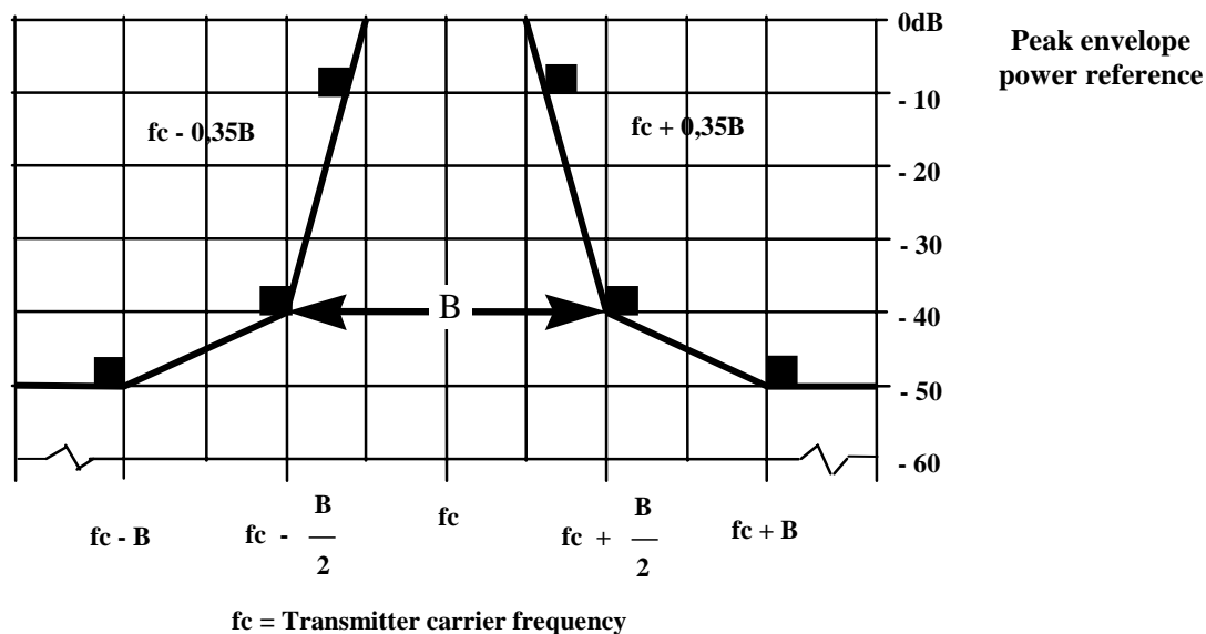
Figure 4: Scaleable spectral mask for digital modulation with B = 600 kHz, 1 200 kHz
