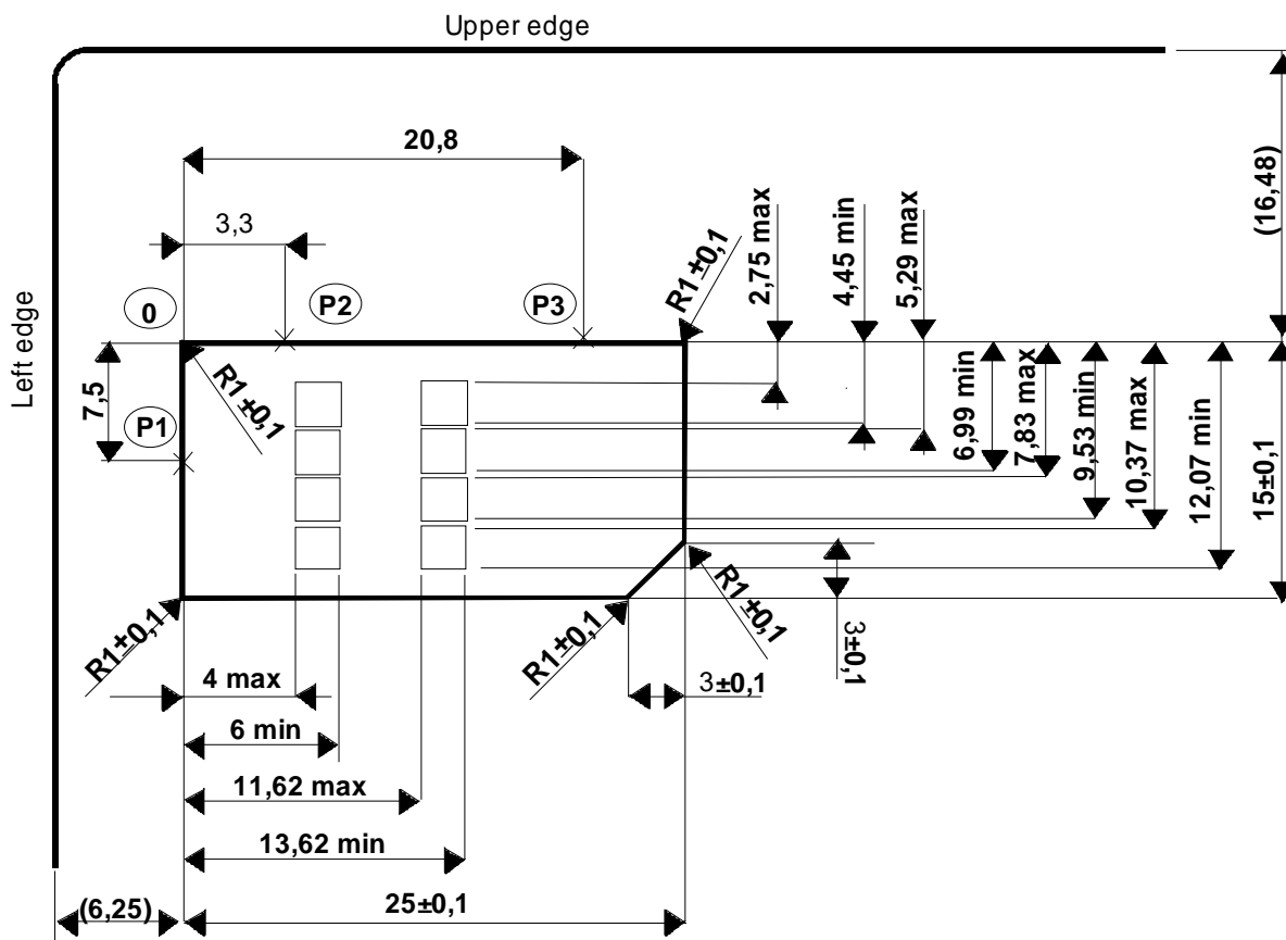
Figure 4.1: Plug-in UICC
