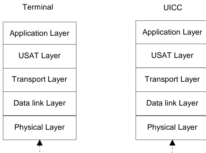
Figure 7.1: Layers
