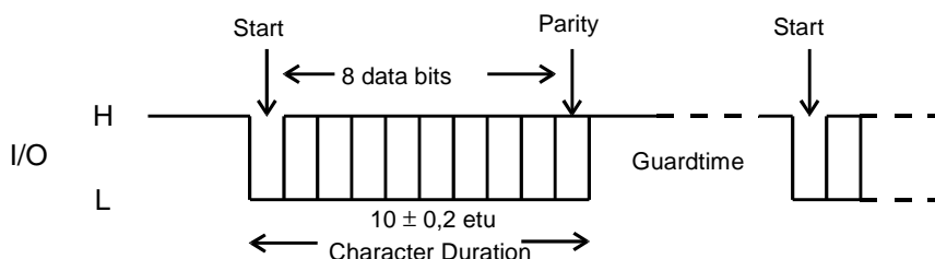
Figure 7.2: Character frame
