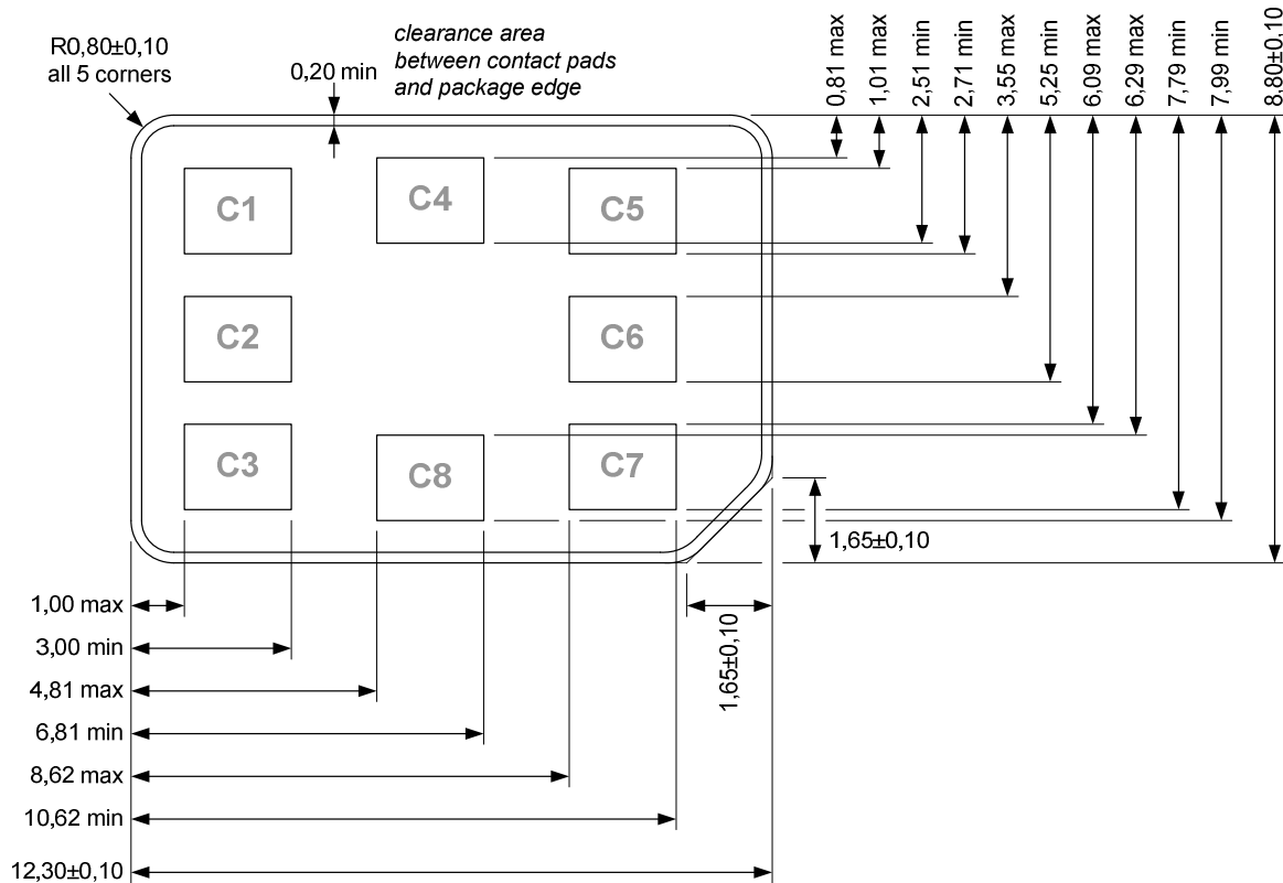
Figure 4.3: 4FF
