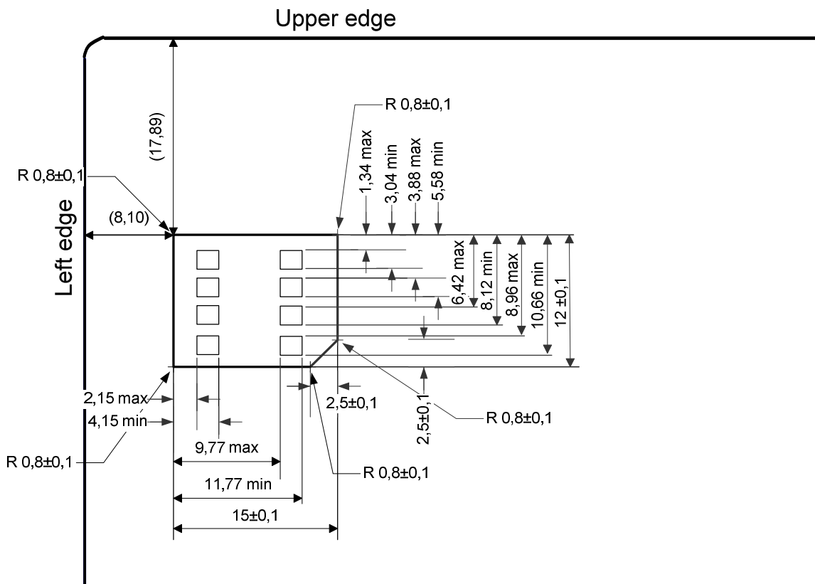
Figure 4.2: Mini-UICC
