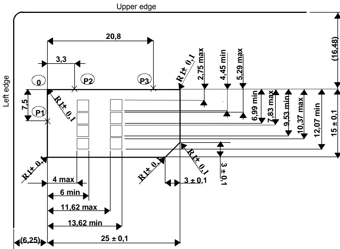
Figure 4.1: Plug-in UICC
