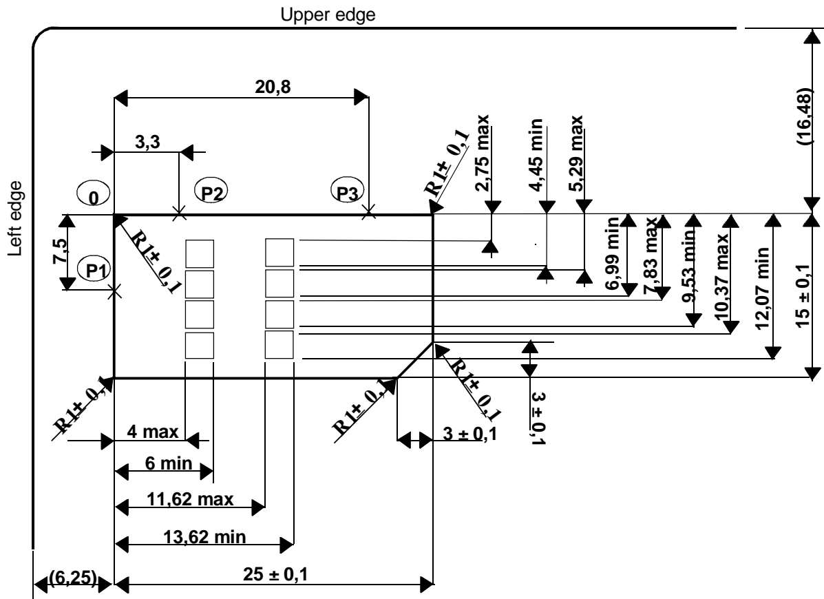
Figure 4.1: Plug-in UICC
