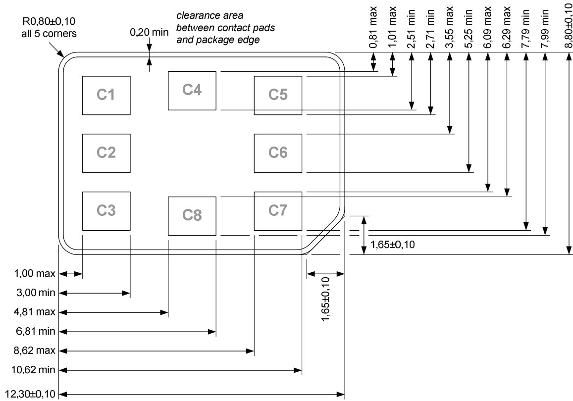
Figure 4.3: 4FF
