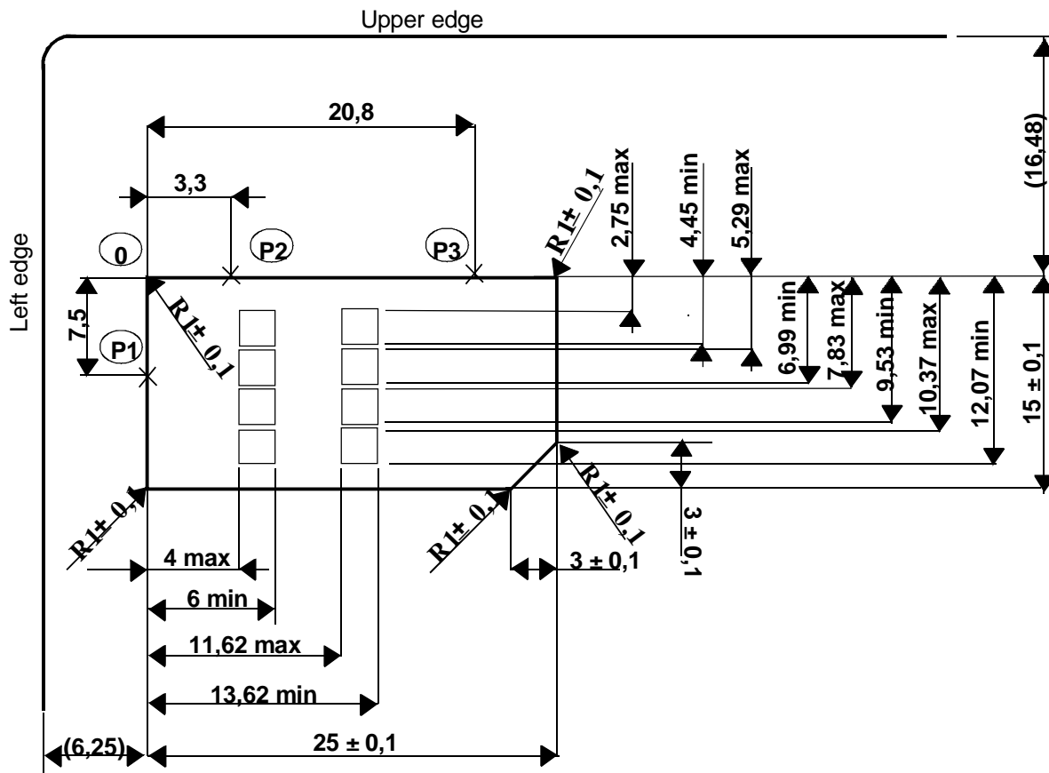
Figure 4.1: Plug-in UICC
