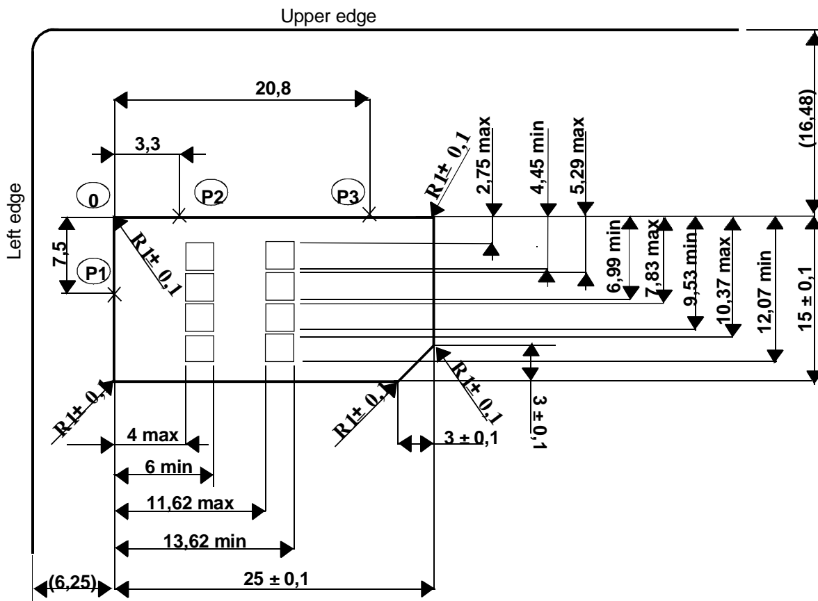
Figure 4.1: Plug-in UICC
