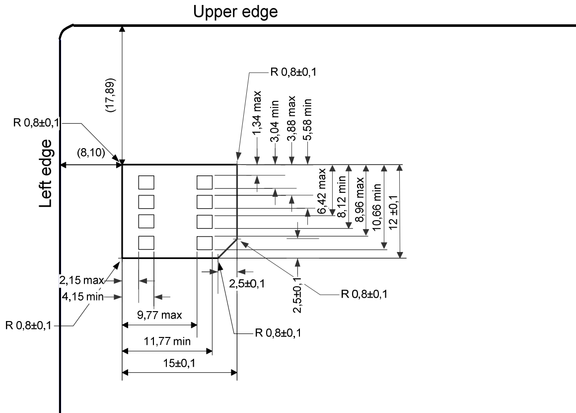
Figure 4.2: Mini-UICC
