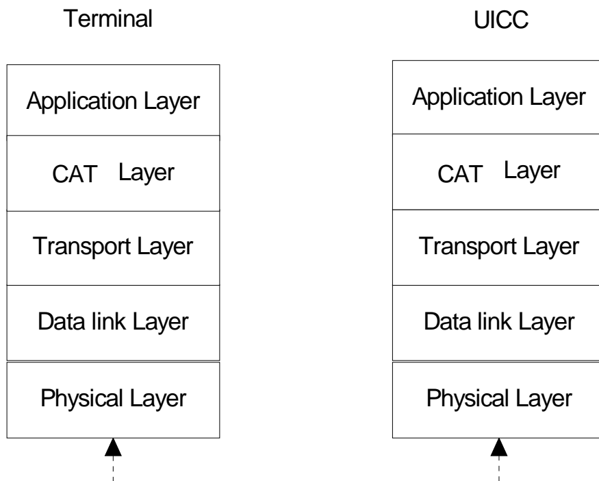
Figure 7.1: Layers
