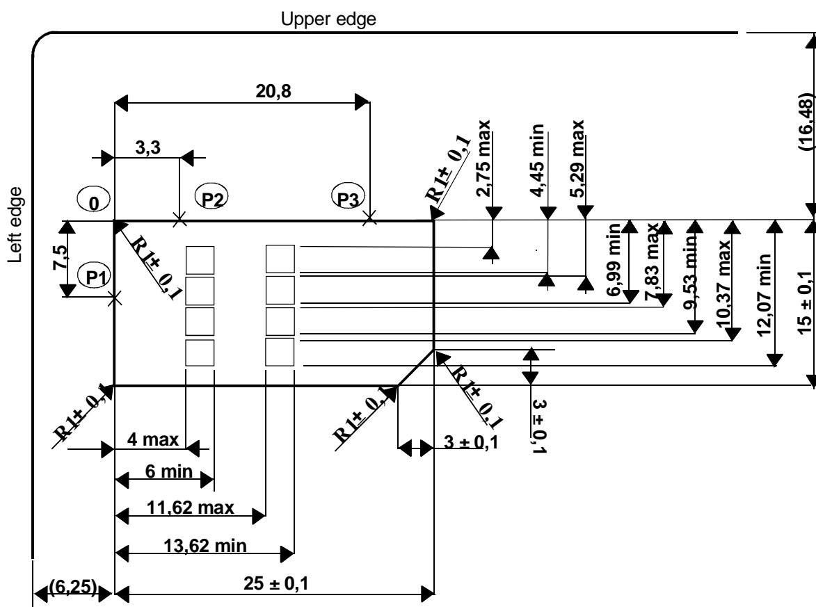
Figure 4.1: Plug-in UICC
