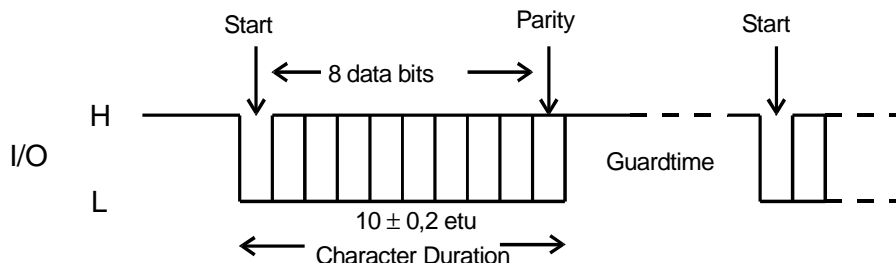
Figure 7.2: Character frame
