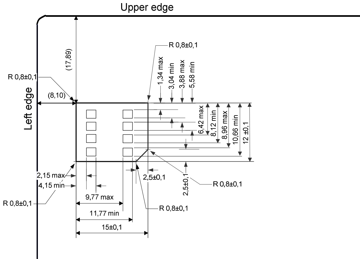
Figure 4.2: Mini-UICC
