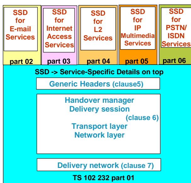
Figure 2: TS 102 232 IP HO Family
