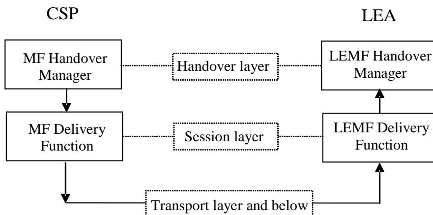
Figure 3: Protocol stack
