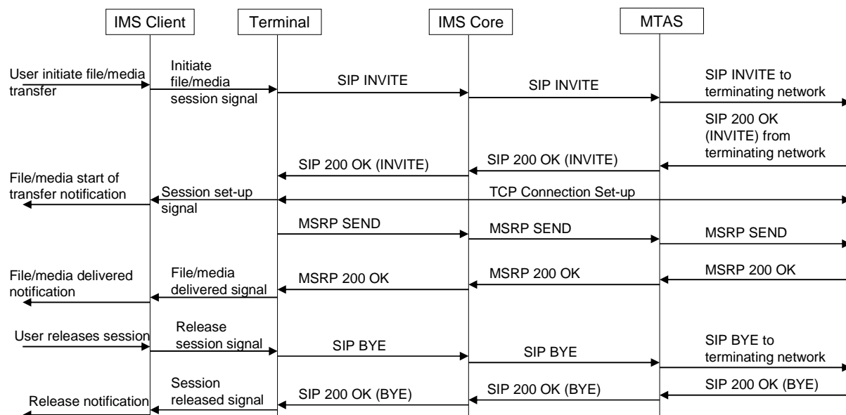
Figure 56: File/Media Sharing using MTSI
