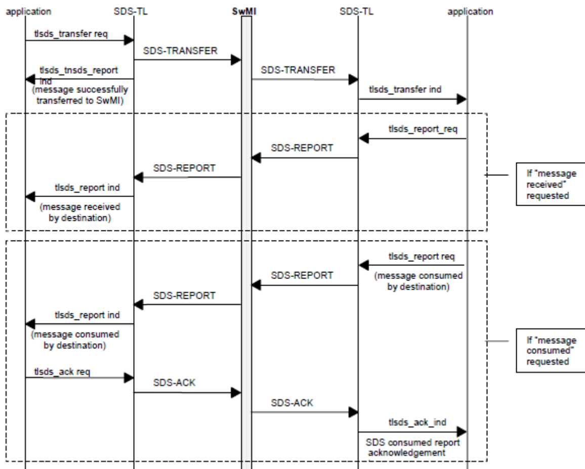
Figure 70: SDS signalling flow chart for SDS type 4 via SDS-TL protocol according to EN 300 392-2 [27], clause 29.3.3 with transparent SwMI transport (SwMI store-and-forward functionality uses additional SDS-REPORT and SDS-ACK messages)
