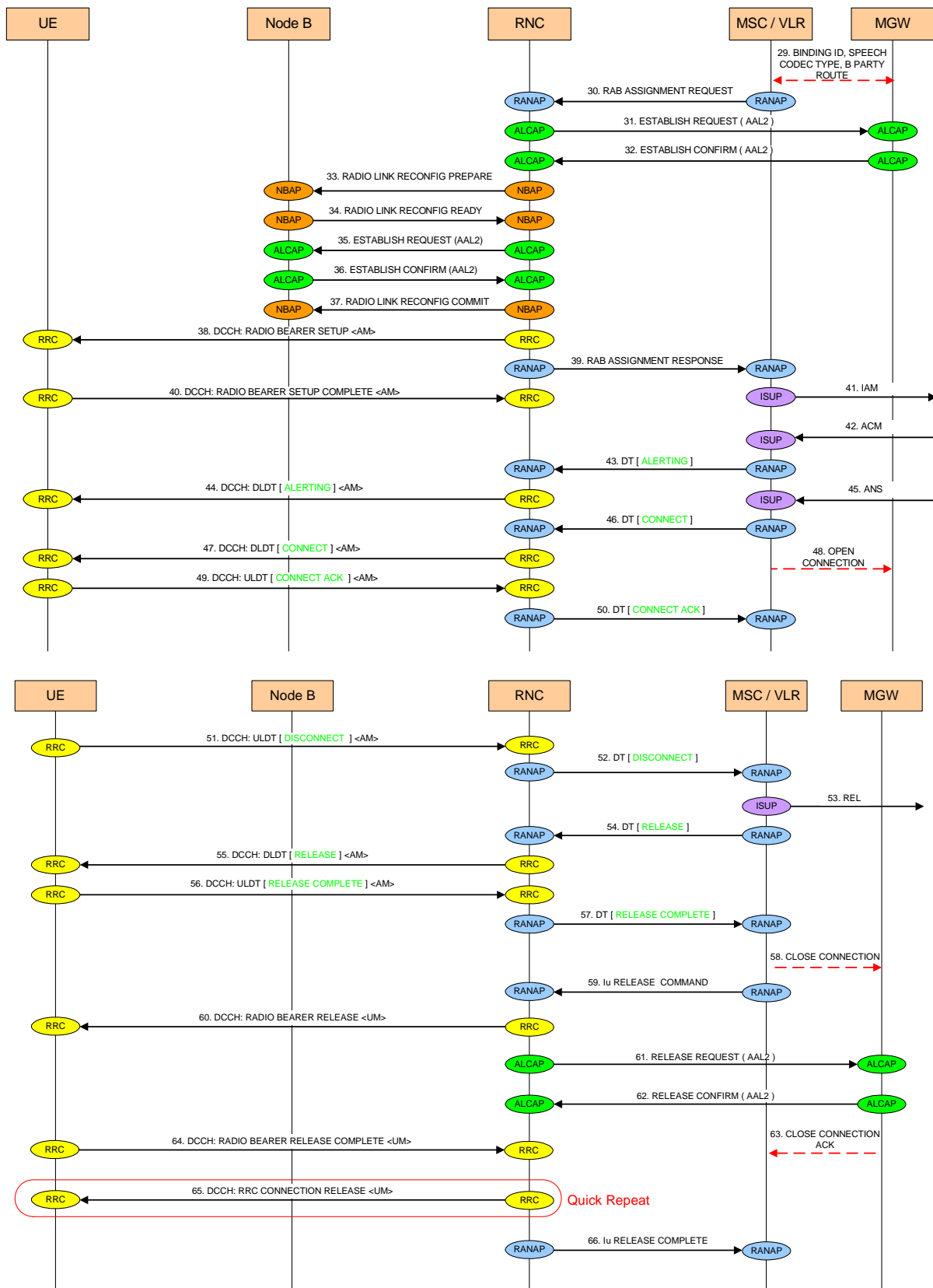
Figure 30: Video telephony signalling flow chart
