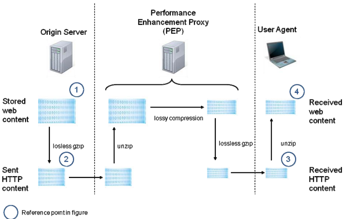
Figure 31: HTTP content download
