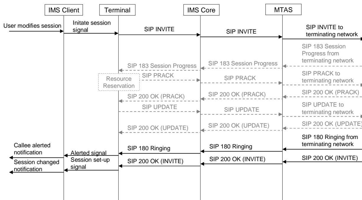
Figure 48: Modification of the MTSI Session
