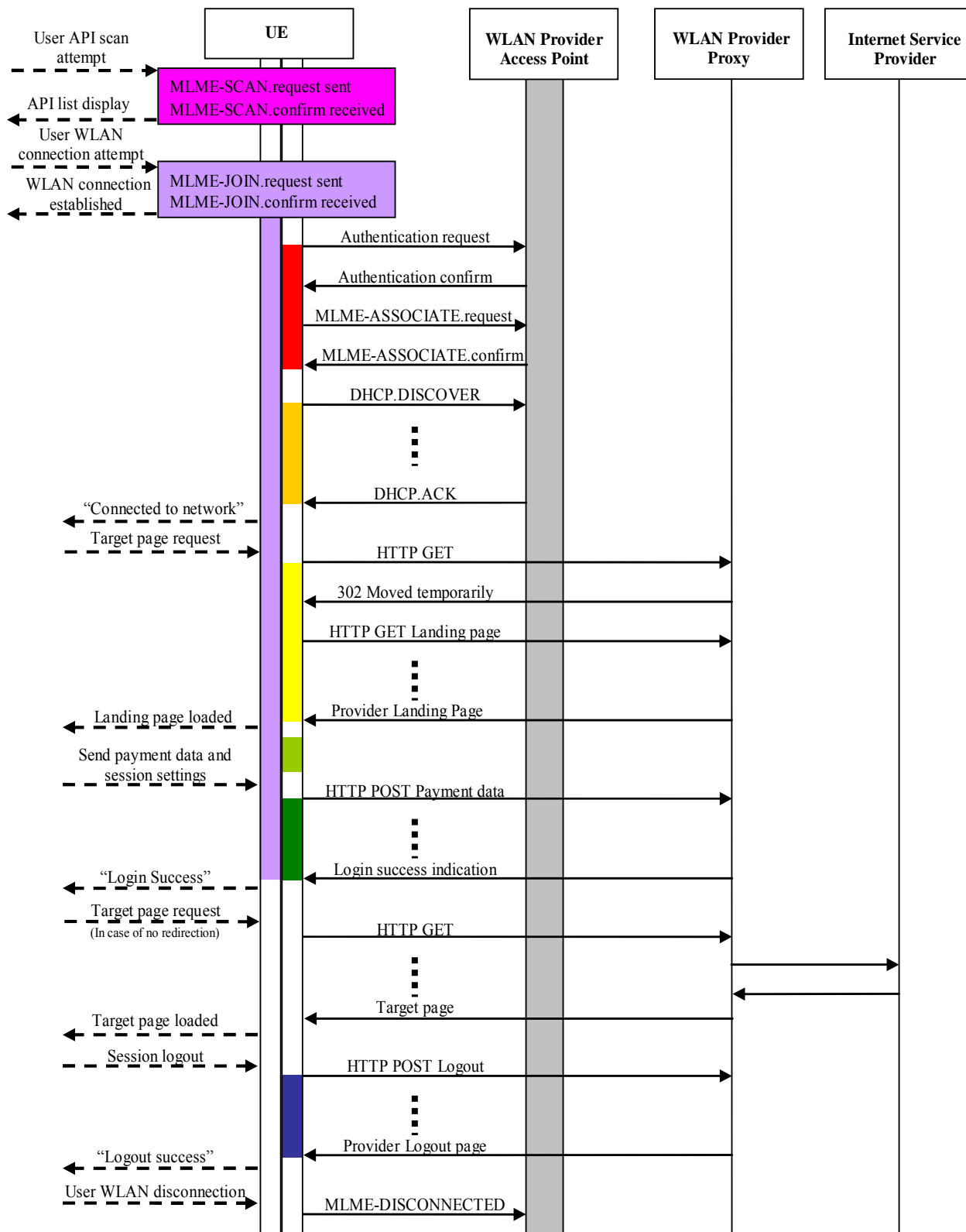
Figure 32: Generic Signal Flow
