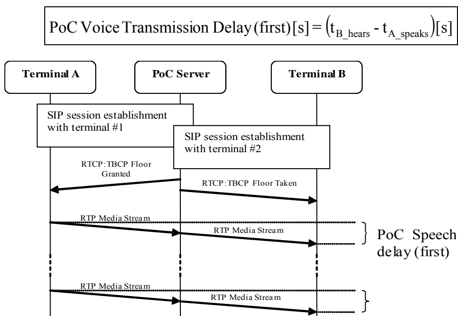
Figure 22: PoC speech transmission delay (first) and PoC speech transmission delay (others)
