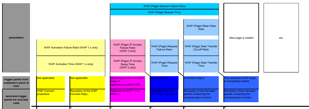
Figure 43: Parameter and service overview
