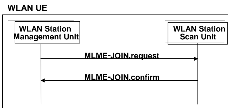
Figure 35: JOIN Signal Flow
