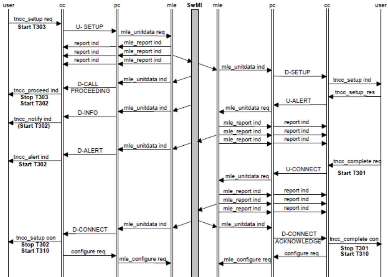
Figure 27: Individual call set-up using on/off hook signalling (EN 300 392-2 [27], clause 14.5.1)
