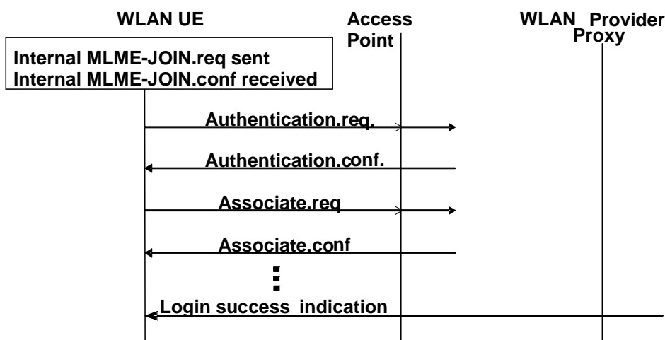
Figure 38: WLAN PS Data Service Provisioning Signal Flow
