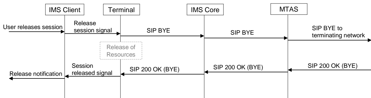
Figure 49: Signalling to end an MTSI Session
