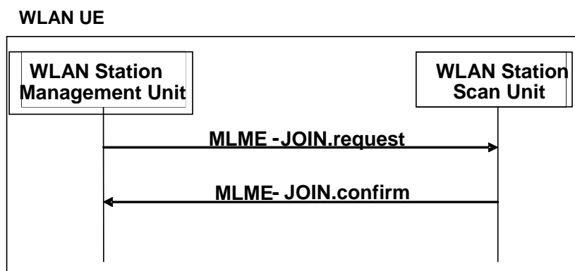
Figure 37: JOIN Signal Flow
