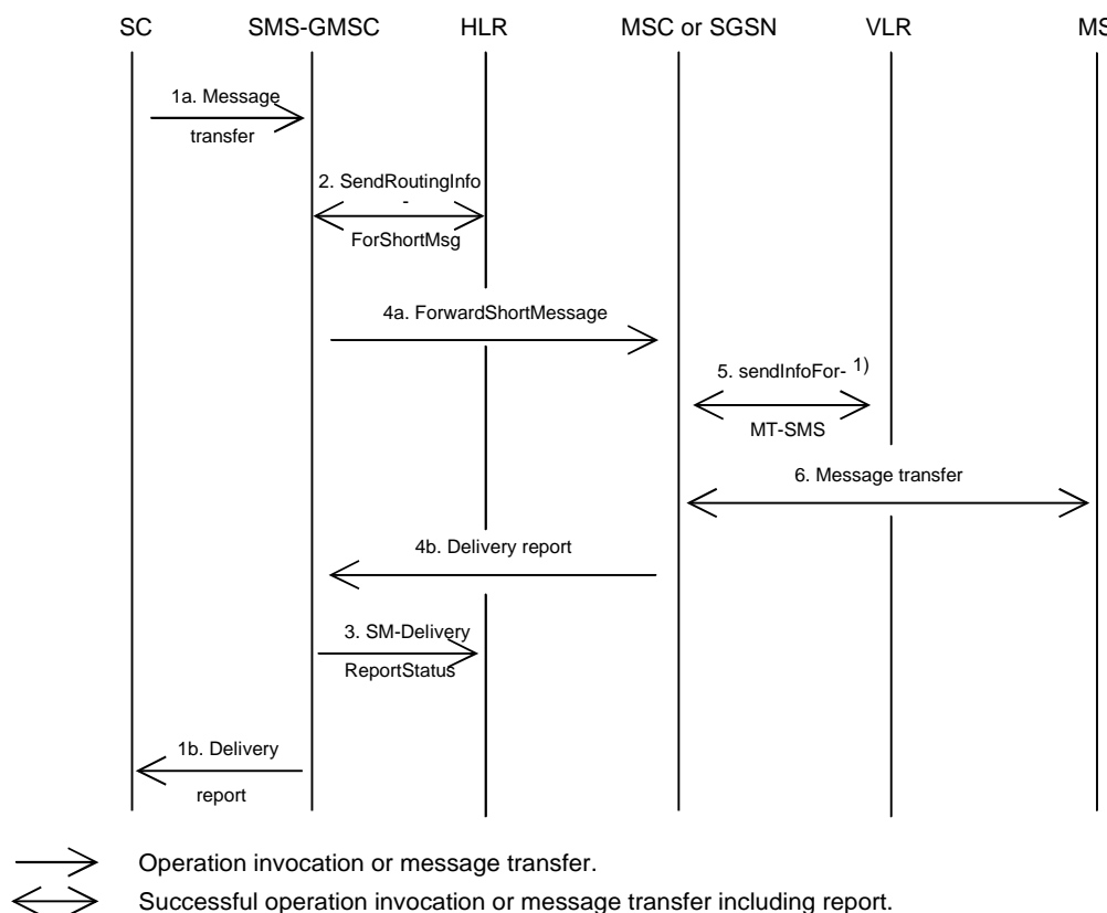
Figure 69: SMS Transaction flow – Terminating UE
