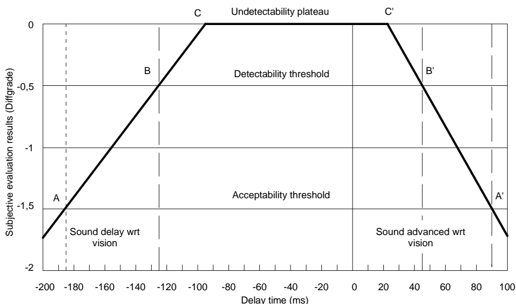
Figure 54: The impact of audio video de-synchronization on perceived quality
