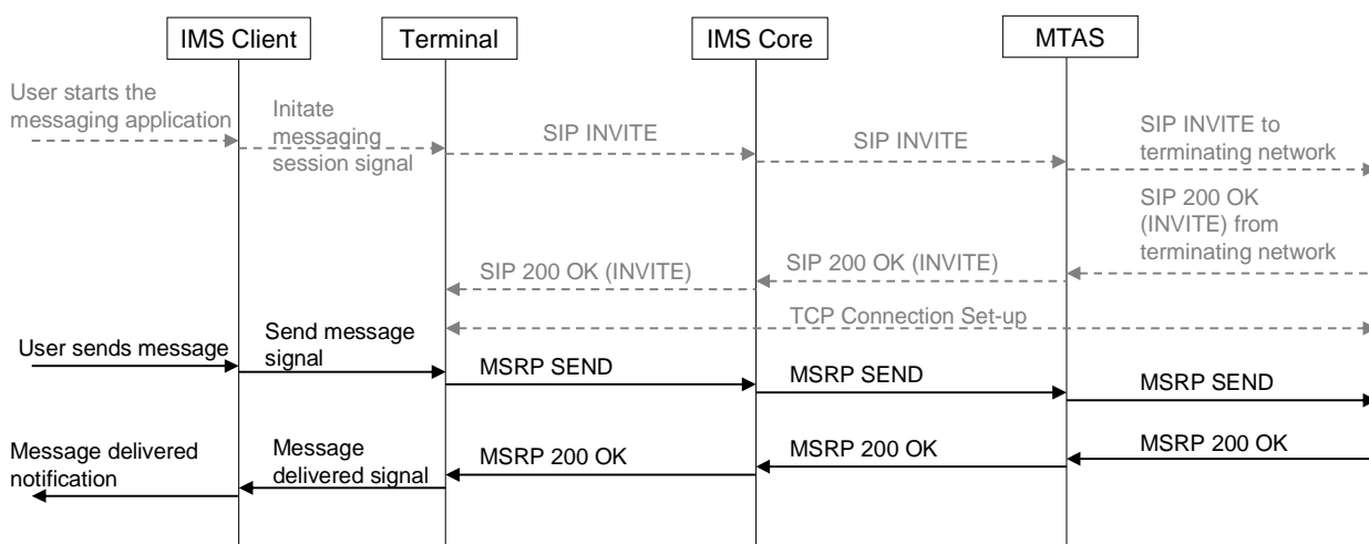
Figure 55: Messaging using MSRP
