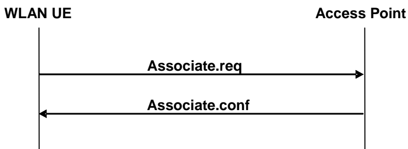
Figure 42: WLAN RE-ASSOCIATION Signal Flow
