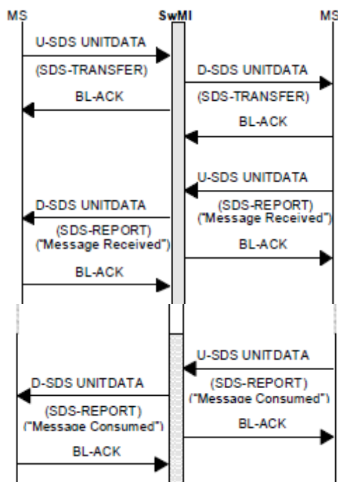
Figure 68: SDS signalling flow chart
