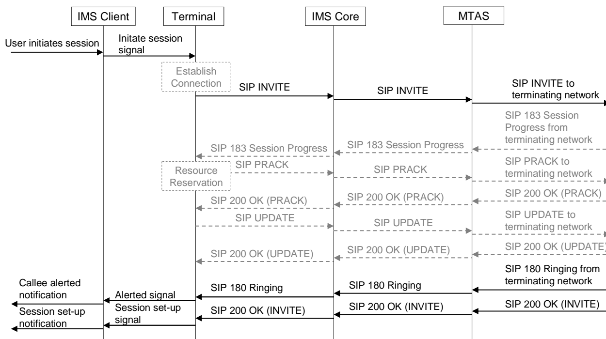
Figure 47: Implicit Initiation of the MTSI Session
