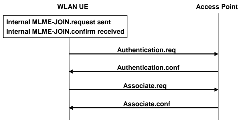
Figure 39: WLAN ASSOCIATION Signal Flow
