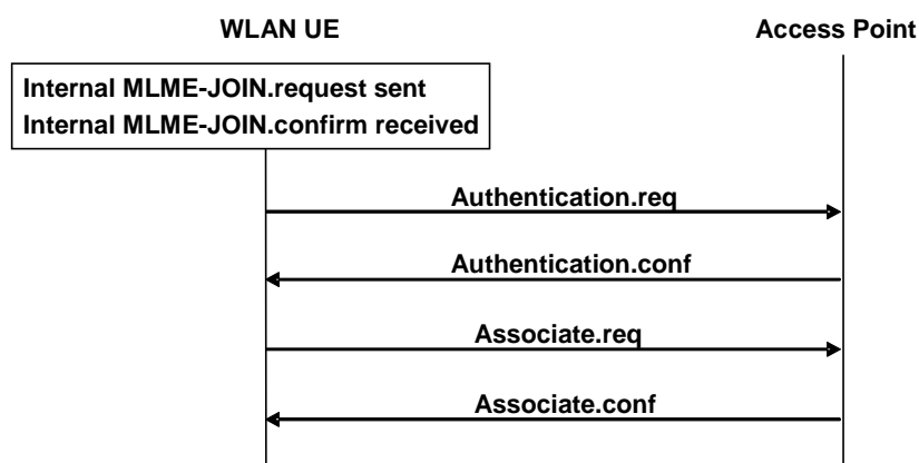
Figure 40: WLAN ASSOCIATION Signal Flow
