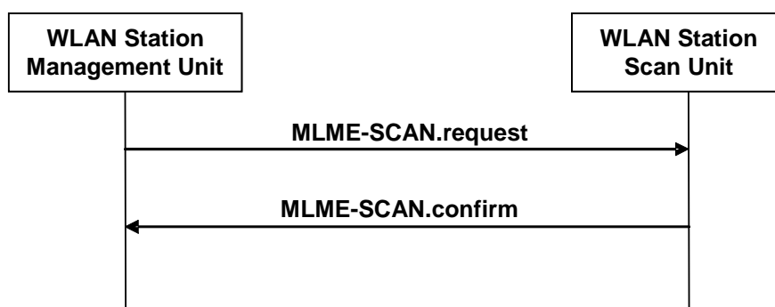
Figure 33: SCAN Signal Flow
