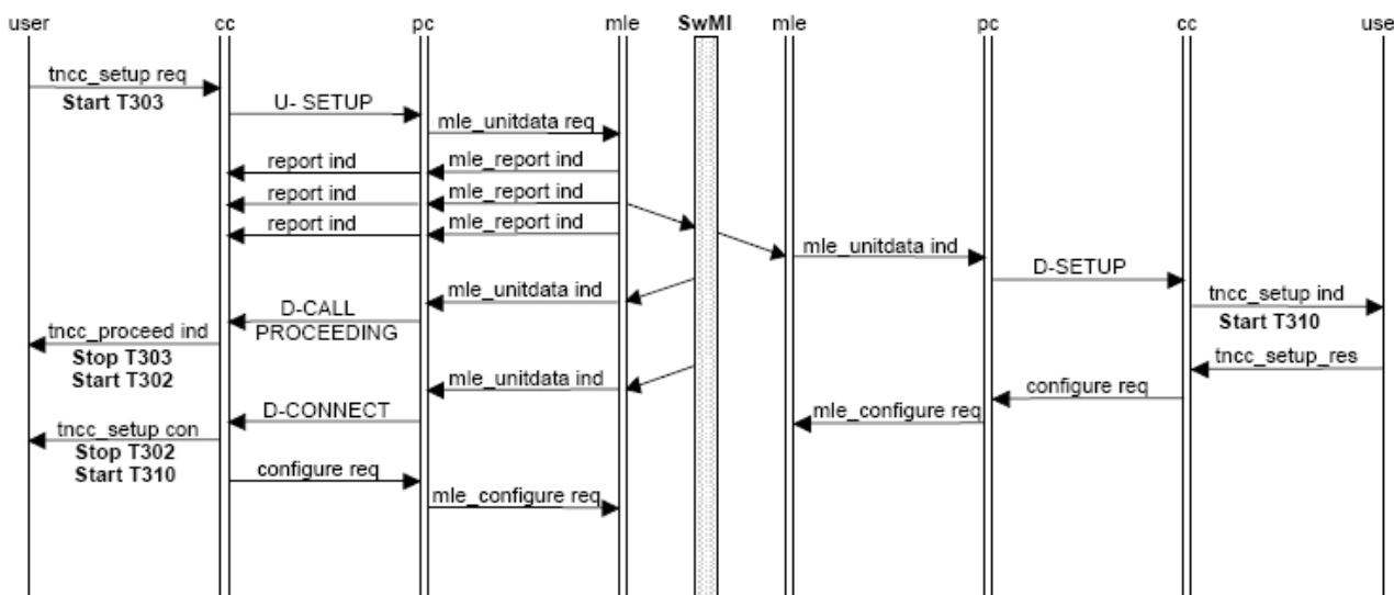
Figure 58: Group call setup procedure
