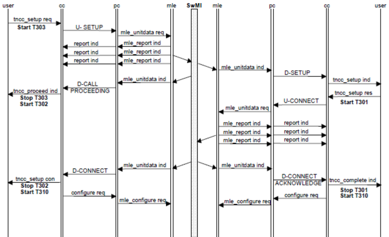
Figure 28: Individual call set-up using direct set-up signalling (EN 300 392-2 [27], clause 14.5.1)
