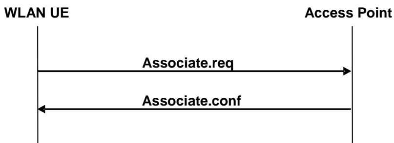
Figure 41: WLAN RE-ASSOCIATION Signal Flow
