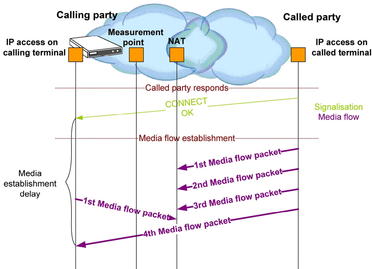
Figure 57: Media setup delayed due to NAT devices
