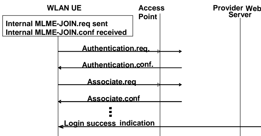
Figure 36: WLAN PS Data Service Provisioning Signal Flow
