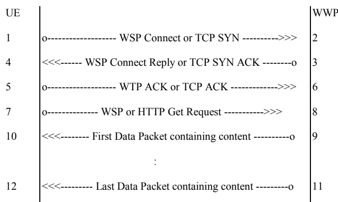
Figure 44: WAP Message Sequence Chart
