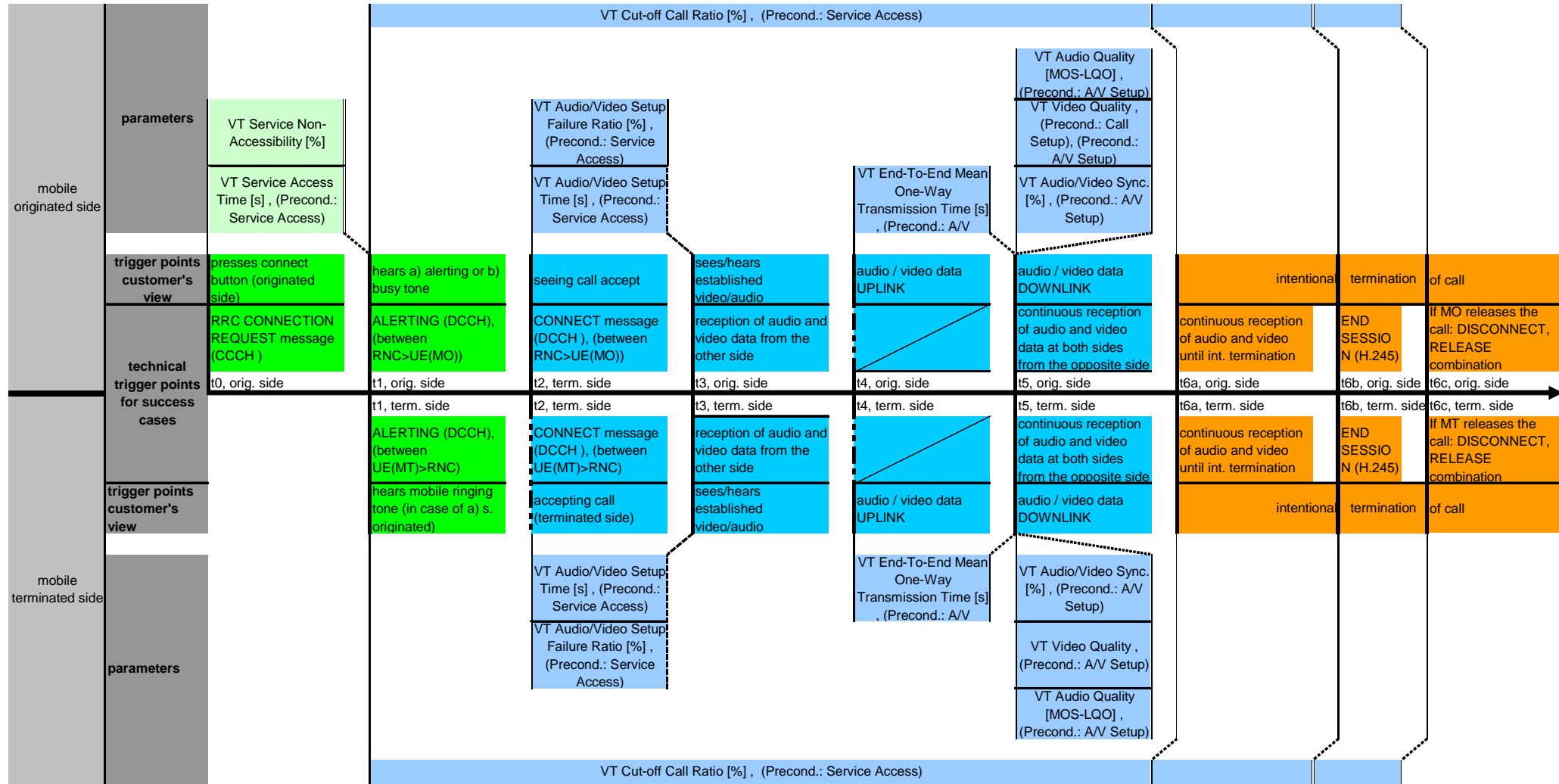
Figure 29: Parameter overview with trigger points
