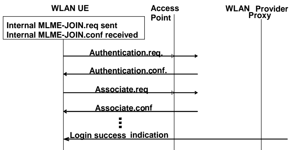
Figure 40: WLAN PS Data Service Provisioning Signal Flow
