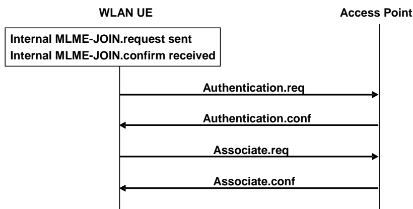
Figure 42: WLAN ASSOCIATION Signal Flow
