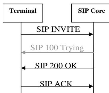
Figure 13: Media parameters negotiation for pre-established session
