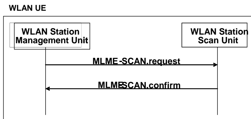
Figure 36: SCAN Signal Flow
