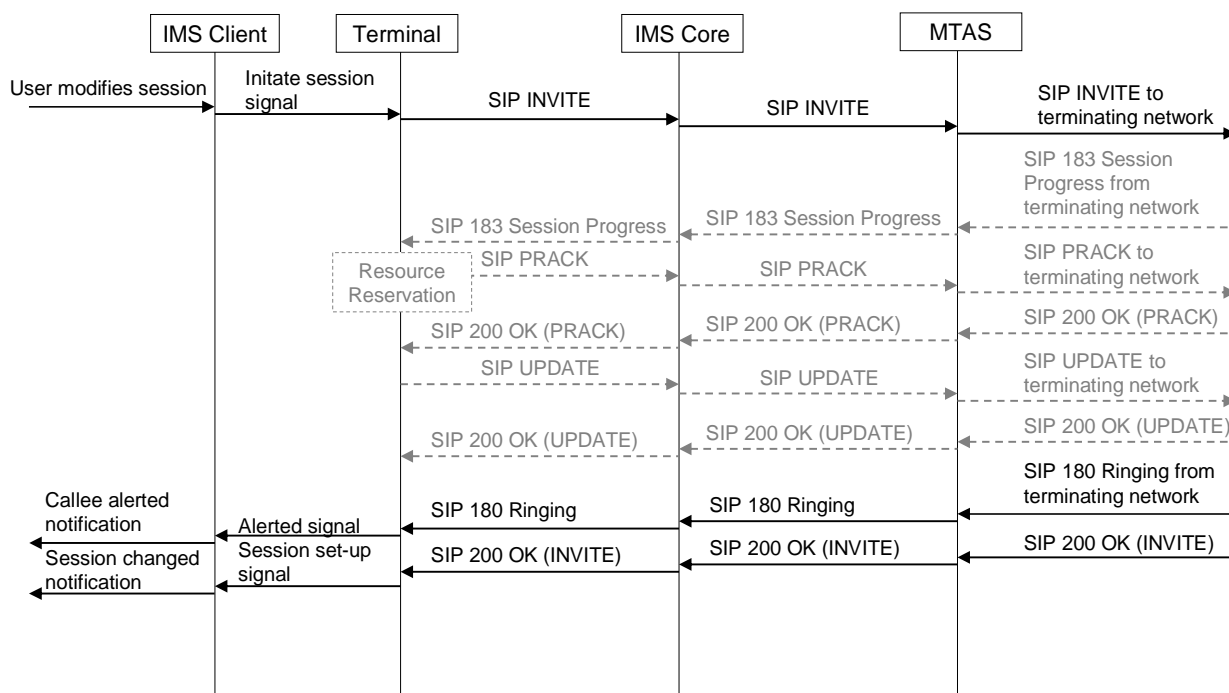
Figure 50: Modification of the MTSI Session
