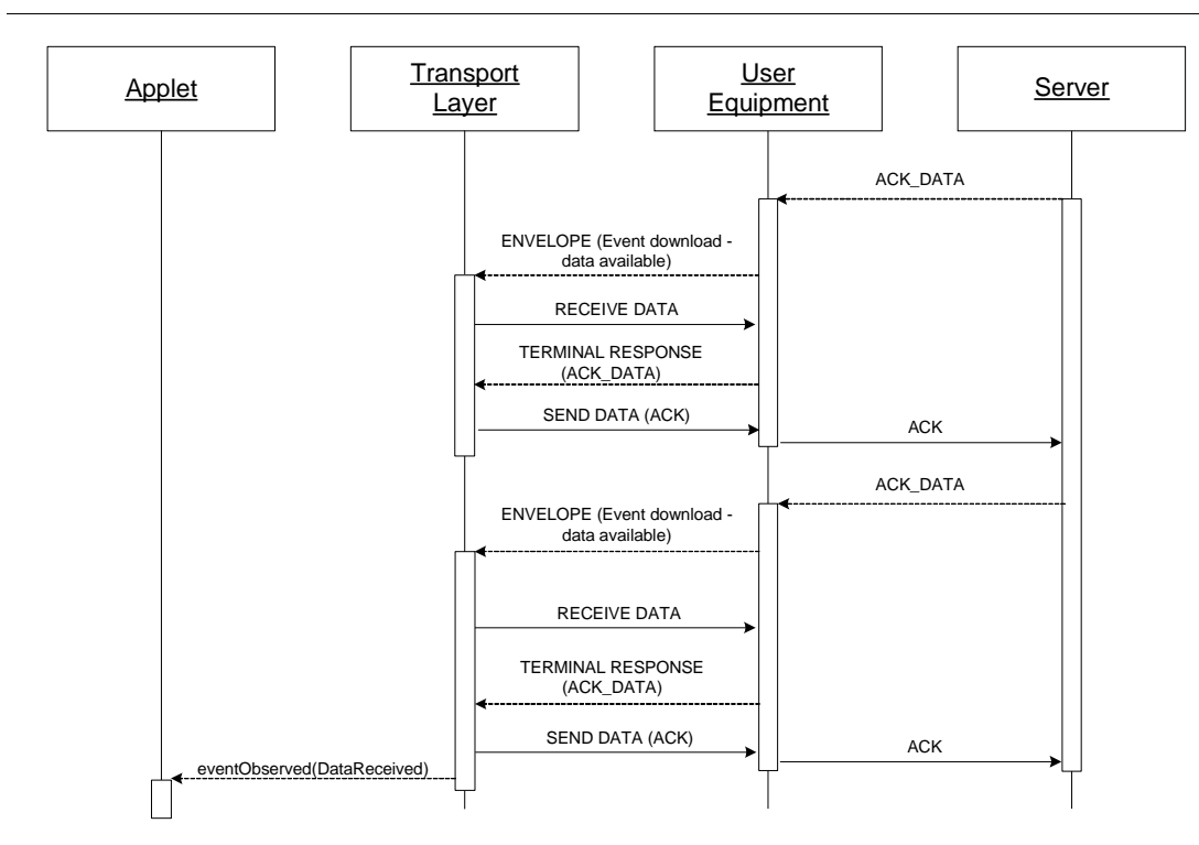
Figure 4: Receiving data
