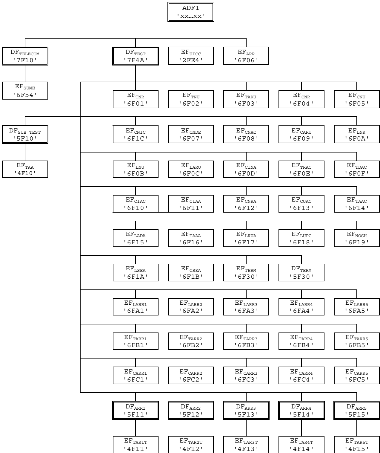
Figure B.2: File identifiers and directory structures under ADF1
