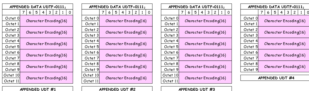
Figure B.30: Unified Data Transport Format (16 bit character) 18 character symbols to 23 character symbols
