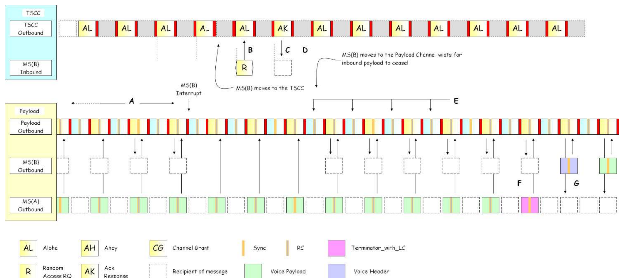
Figure 6.37: Payload Interrupt
