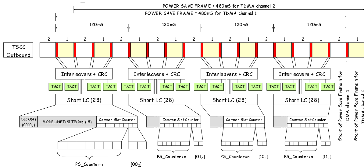
Figure 6.26: Power Save Frame Structure
