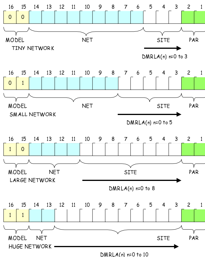
Figure 6.15: Allocation of NET and SITE information elements in C_SYSCode
