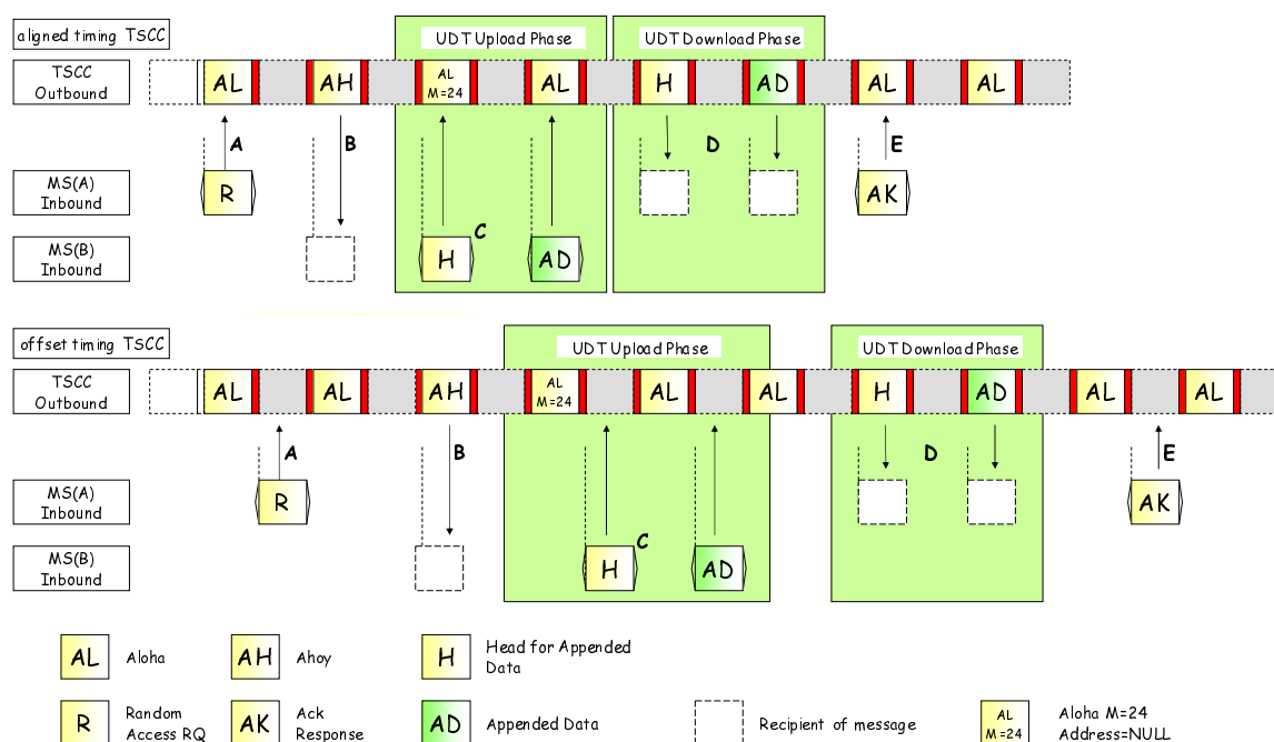
Figure 6.52: Example of a Short Data Polling transfer
